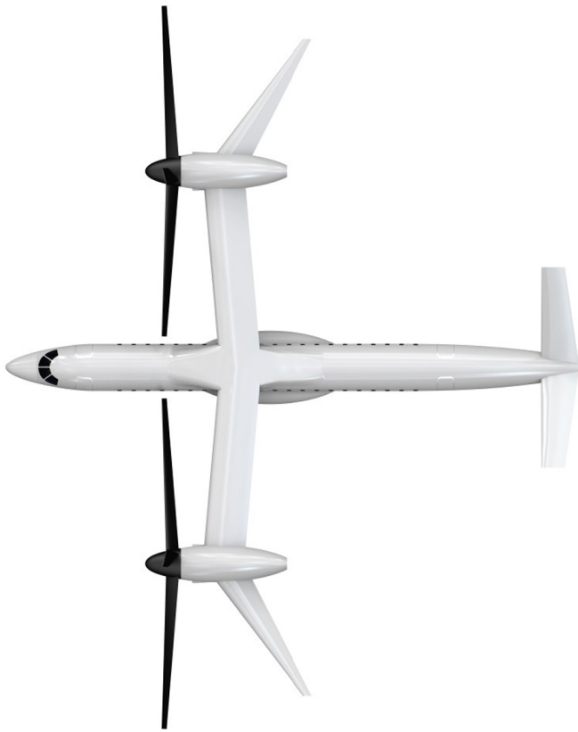
Fig. 5. LCTR with 25-ft swept extensions.
