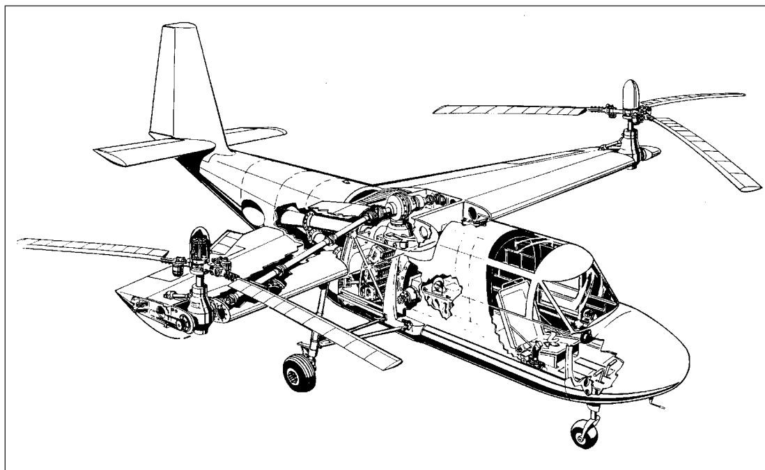
Figure A-3. Transcendental Model 2 cutaway drawing.
