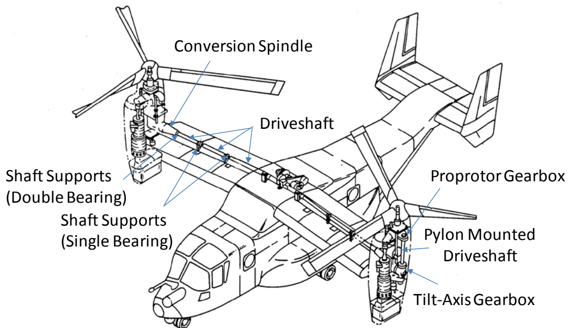
Figure 3-12. A representative tiltrotor drive system illustration
