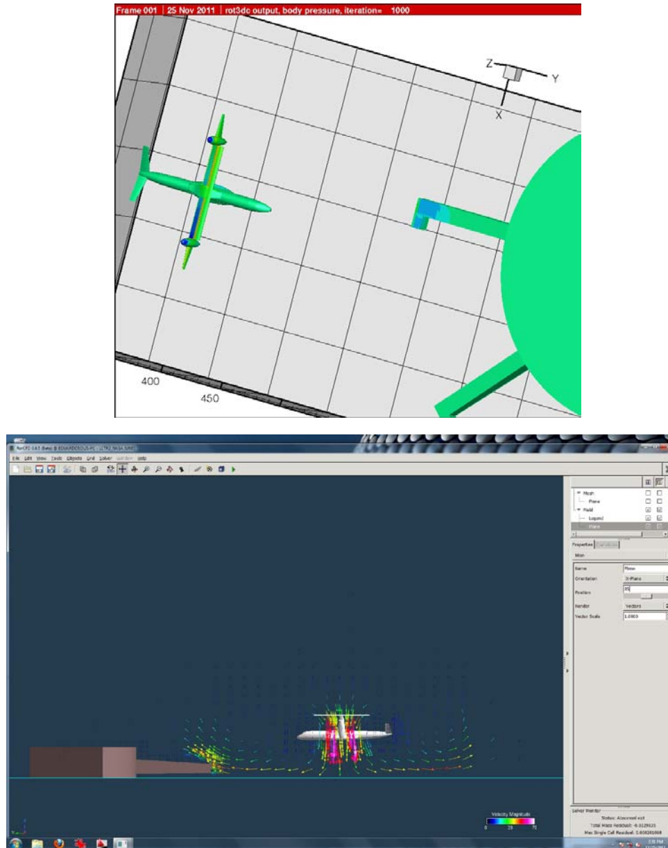
Figure 3-13. A notional CTR gate area layout and potential wake effects (courtesy of Solera Helitech)
