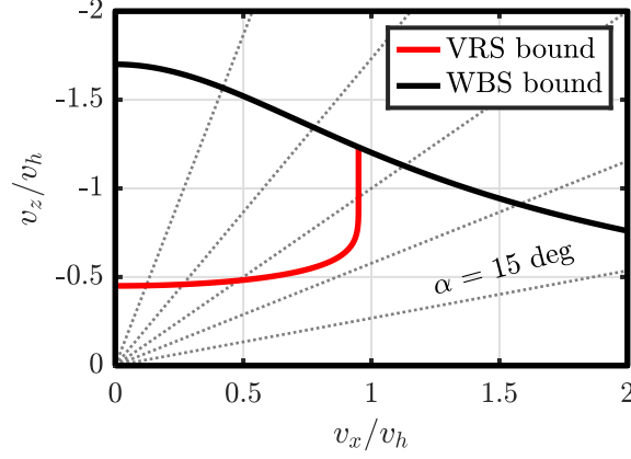
Fig. 6 VRS boundary from [15] and empirical WBS boundary used to predict the onsets of VRS and WBS. The dashed lines are lines of constant shaft angle spaced 15 deg apart; shaft angle increases counterclockwise from 0 deg to 90 deg.
