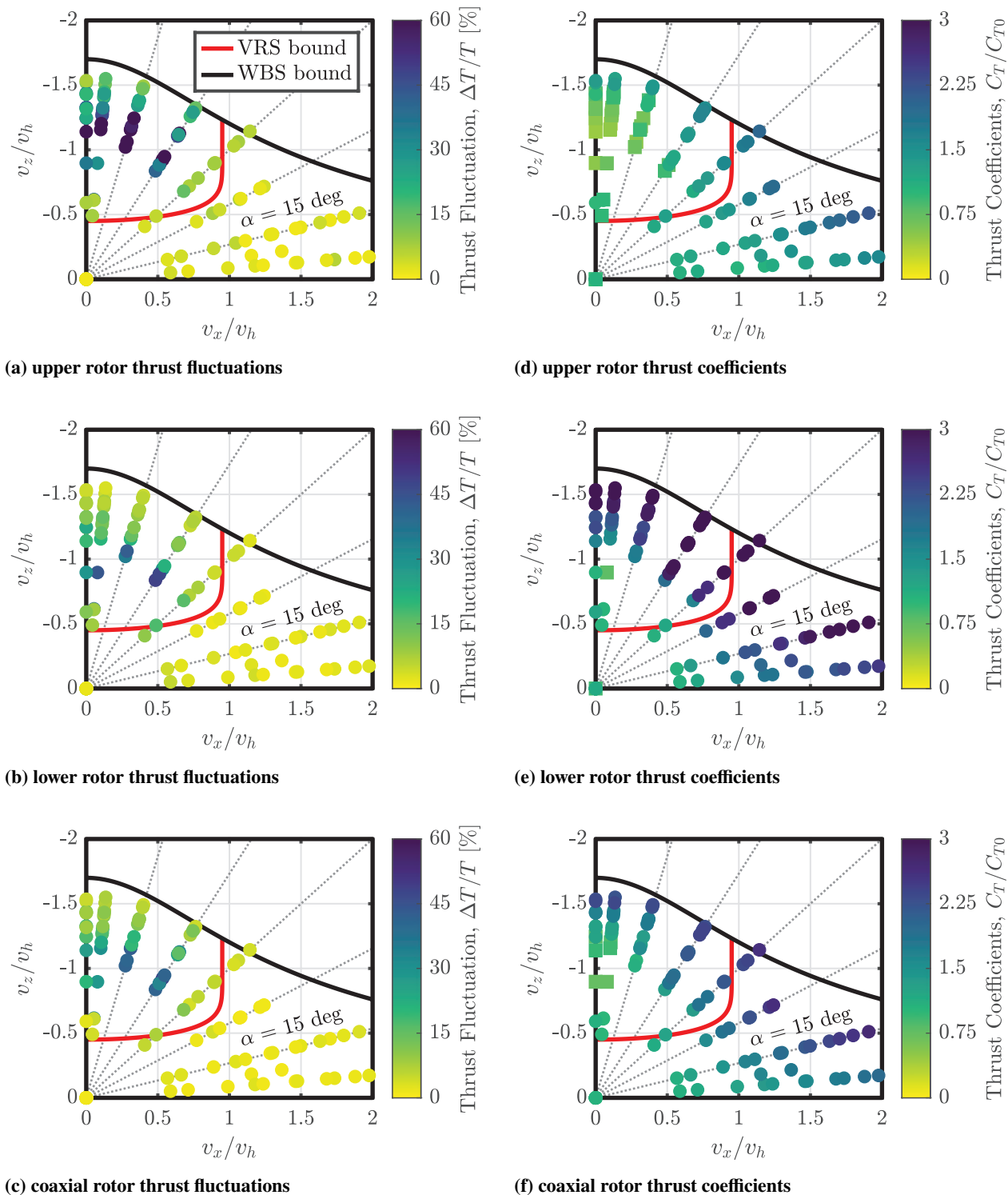
Fig. 16 Unsteady thrust fluctuations relative to the mean (a-c) and thrust coefficients normalized relative to hover (d-f) for quasi-steady test points at 600 RPM and 750 RPM. In (d-f), the square symbols denote points where C_T/C_{T0} < 1 . The dashed lines are lines of constant shaft angle spaced 15 deg apart; shaft angle increases counterclockwise from 0 deg to 90 deg.
