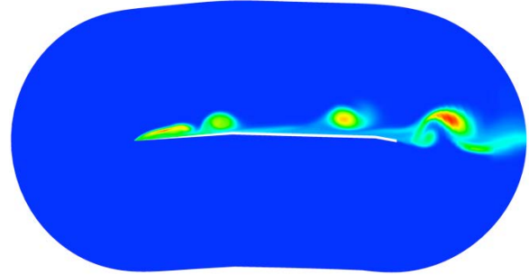
Fig. 28 Amplification factor at \alpha = 5.0^\circ , Re = 10,117 for M = 0.30 ; highest amplification factor in red, \tilde{n}_{max} = 7.2 (transition model, time-accurate).
