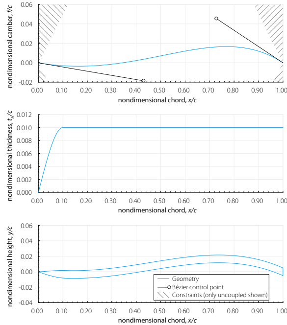
Fig. 10 Cambered plate camber, baseline thickness, and airfoil shape. The vertical axis is enlarged to show details.
