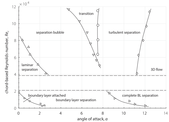
Fig. 7 Regions of characteristic flow modes of an NACA 0012, from Huang et al. 36
