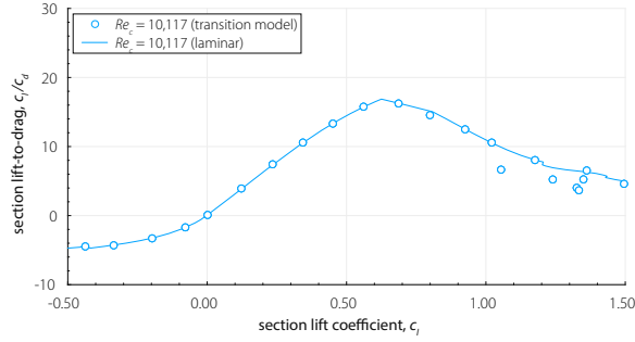
Fig. 25 OVERFLOW Lift-to-drag ratio for Re/M = 33,724 ( Re = 10,117 ) for M = 0.30 .
