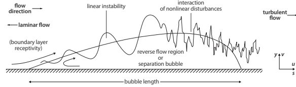
Fig. 4 Aspects of laminar flow breakdown in the separation region, from Boiko et al. 21
