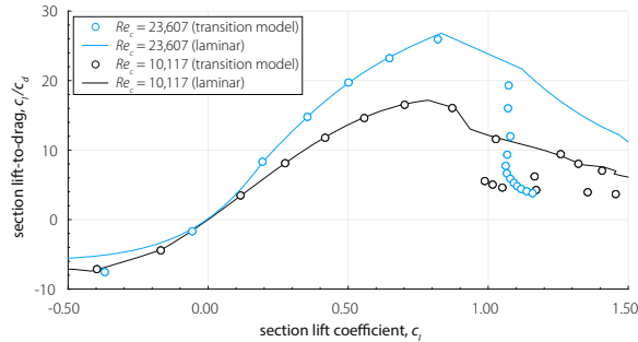
Fig. 27 OVERFLOW Lift-to-drag ratio for Re/M = 33,724 ( Re = 23,607 ) and Re = 10,117 for M = 0.70 .
