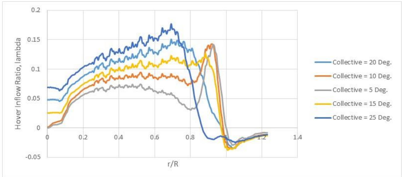
Figure 8. Collective sweep showing CFD rotor inflow results for \Delta\theta_{\text{Tip}} = +8.75 degrees with untwisted tip outer-span.
