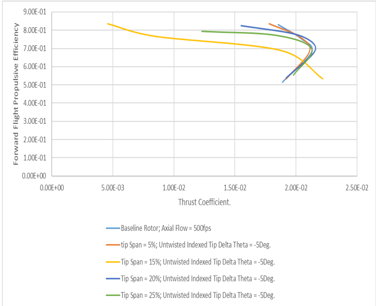
Figure 62. Cruise propulsive efficiency as a function of thrust coefficient, for \Delta\theta = -5 degrees, for different tip spans (percent of rotor radius) for an axial-flow cruise speed of 500 fps.
