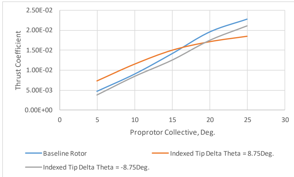
Figure 17. Thrust coefficient trends with collective at two different indexed-tip \Delta\theta settings.
