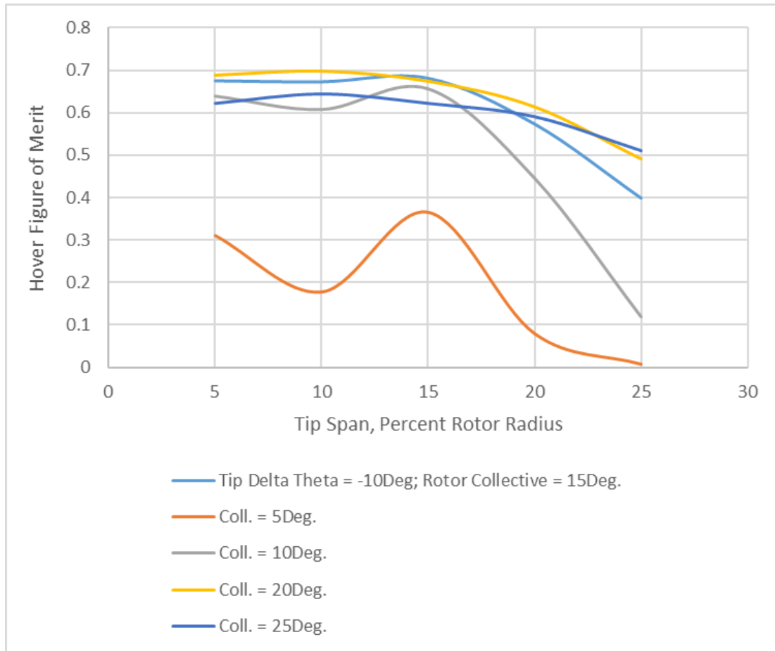
Figure 53. Effect of untwisted tip span for a \Delta\theta = -10 degrees for different rotor collectives for hover.
