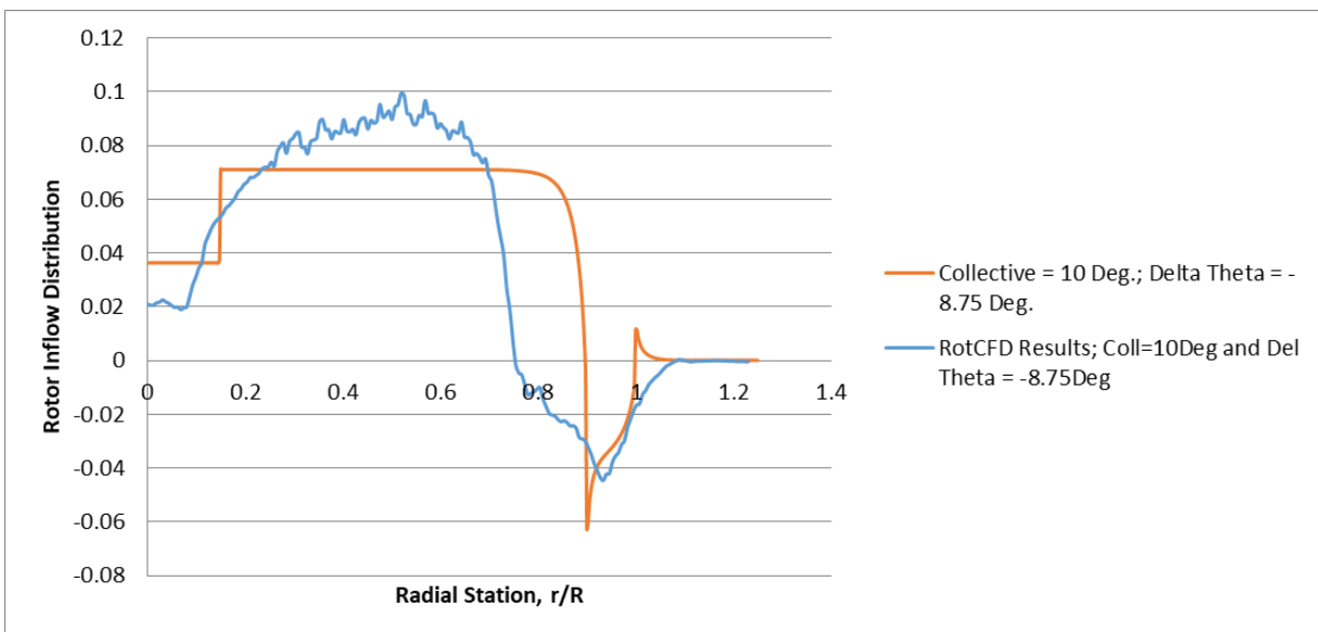
Figure 13. RotCFD and Prandtl-type superposition analysis for hover inflow radial distribution at \theta=10 and \Delta\theta_{tip} = -8 .
