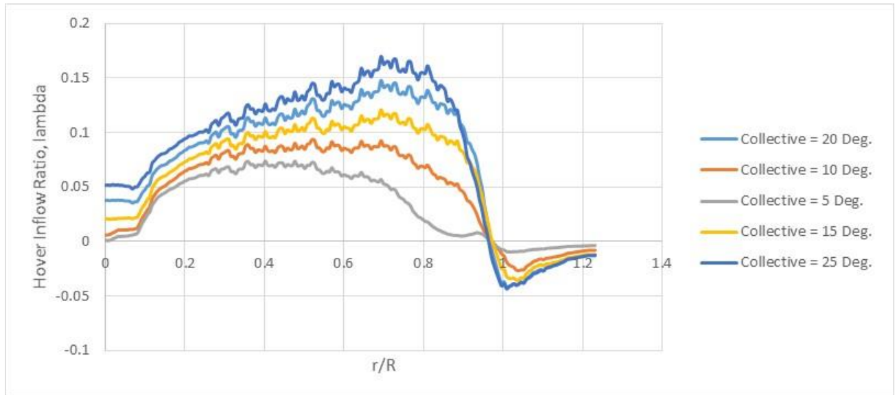
Figure 9. Collective sweep showing CFD rotor inflow results for \Delta\theta_{\text{Tip}} = 0 degrees with untwisted tip outer-span.
