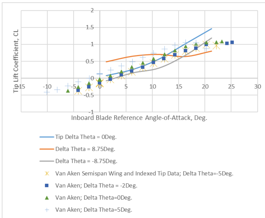
Figure 32. Tip lift curve qualitative comparison.
