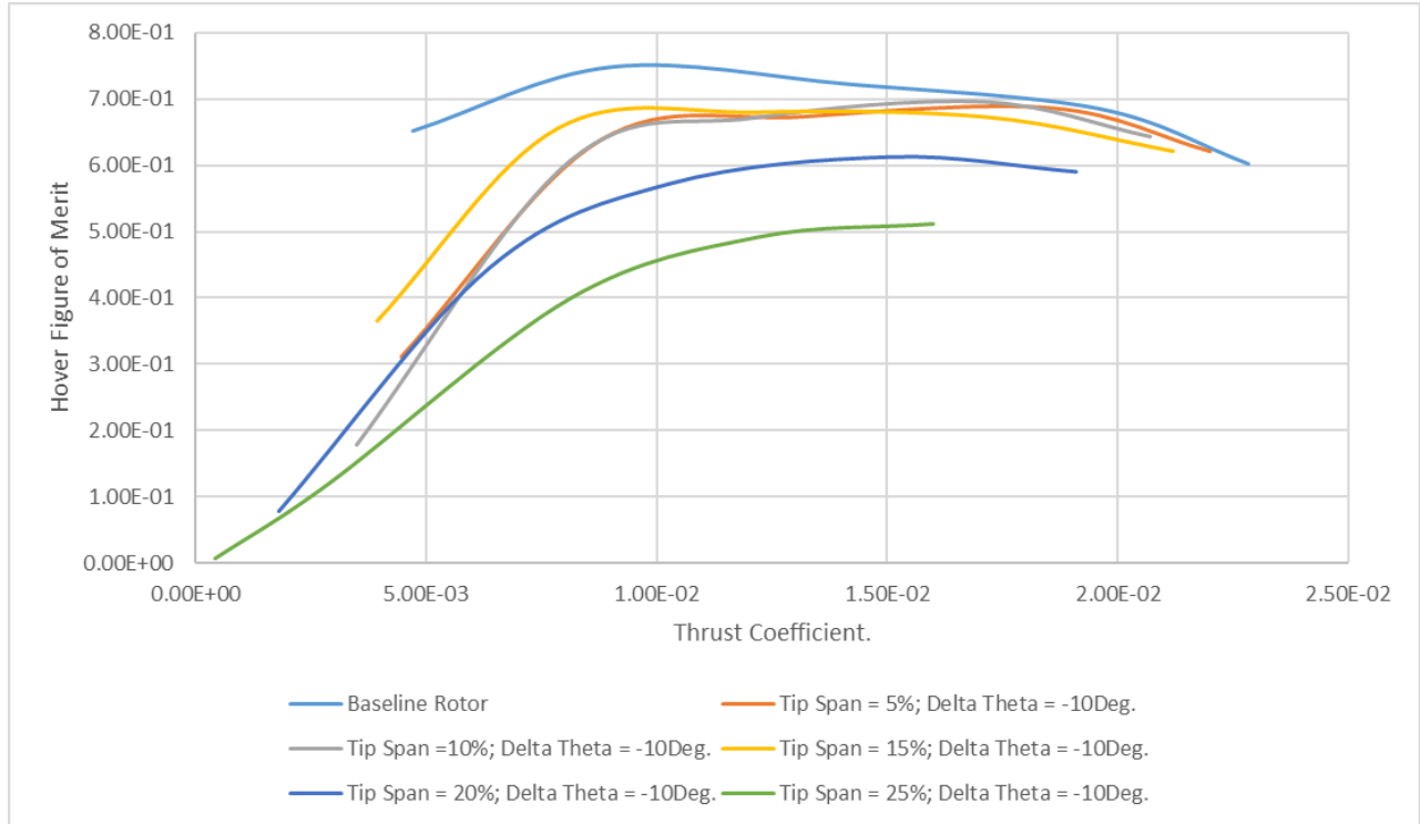
Figure 59. Hover figure of merit as a function of rotor thrust coefficient, for \Delta\theta = -10 degrees., for different tip spans (percent of rotor radius).
