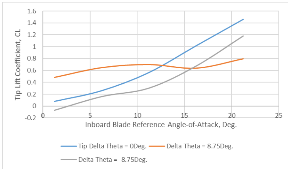
Figure 31. Indexed-tip effective lift and drag coefficient characteristics as a function of inboard-blade reference angle-of-attack hover conditions (Collective of 20 degrees).
