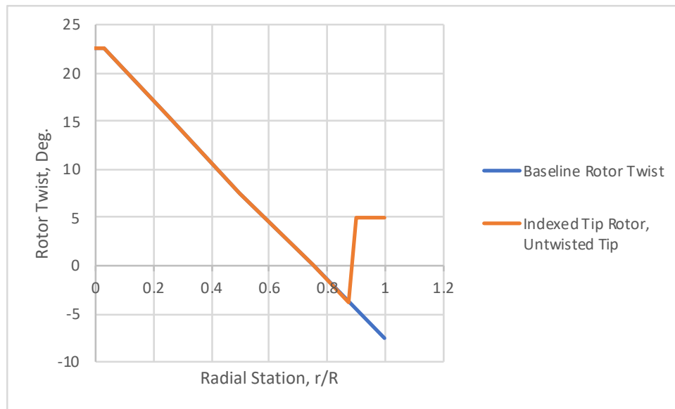
Figure 5. Representative rotor twist distribution: baseline rotor and 10-percent span indexed-tip set at 5 degrees tip-twist.
