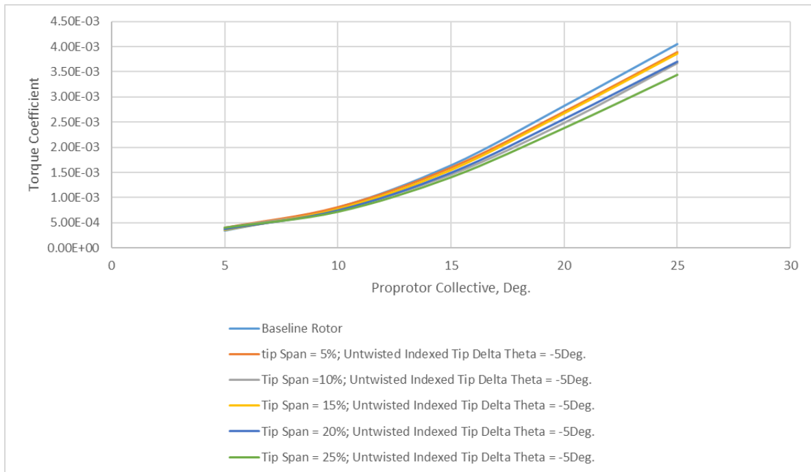
Figure 55. Rotor torque coefficient as a function of rotor collective, for \Delta\theta = -5 degrees, for different tip spans (percent of rotor radius).
