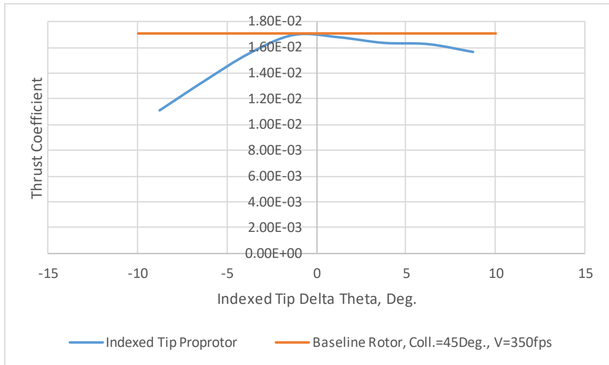
Figure 20. Cruise/axial flow thrust coefficient trend (for an untwisted indexed-tip) as a function of indexed-tip \Delta\theta (Coll. = 45 degrees and V=350 fps).
