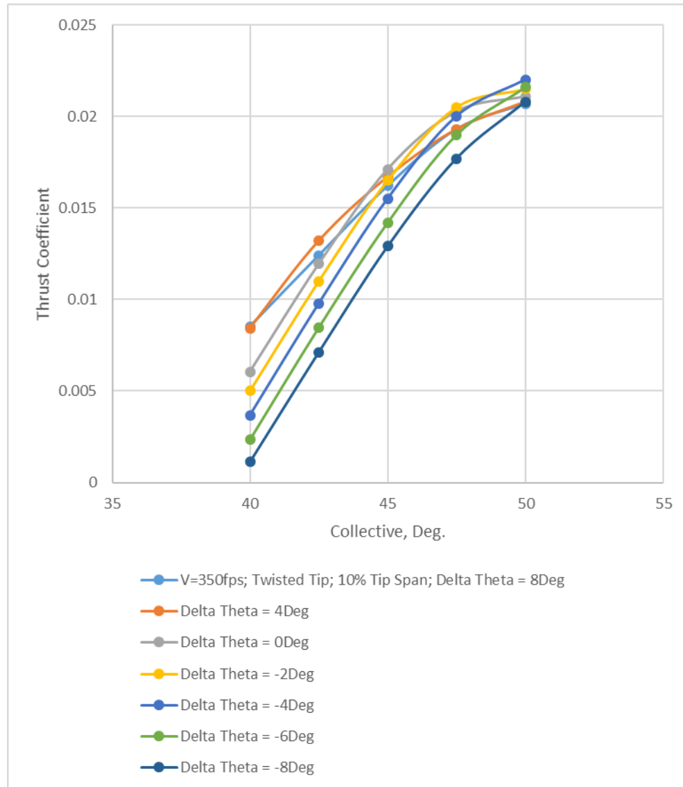
Figure 41. Thrust coefficient versus rotor collective at an axial-flow cruise speed of 350 fps for different values of \Delta\theta .
