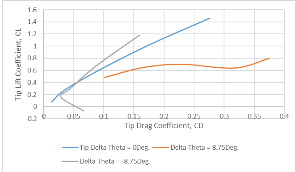
Figure 30. Tip lift-drag coefficient polar curves as a function of tip angle of attack for three different indexed-tip \Delta\theta .
