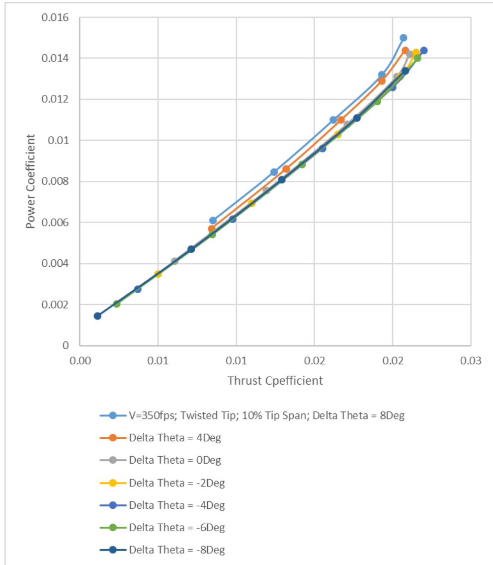
Figure 43. Power coefficient versus rotor thrust coefficient at an axial-flow cruise speed of 350 fps for different values of \Delta\theta .
