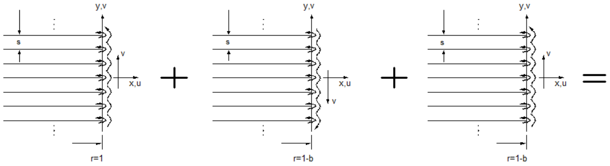
Figure 3. Extended Prandtl two-dimensional vortex sheet model.
