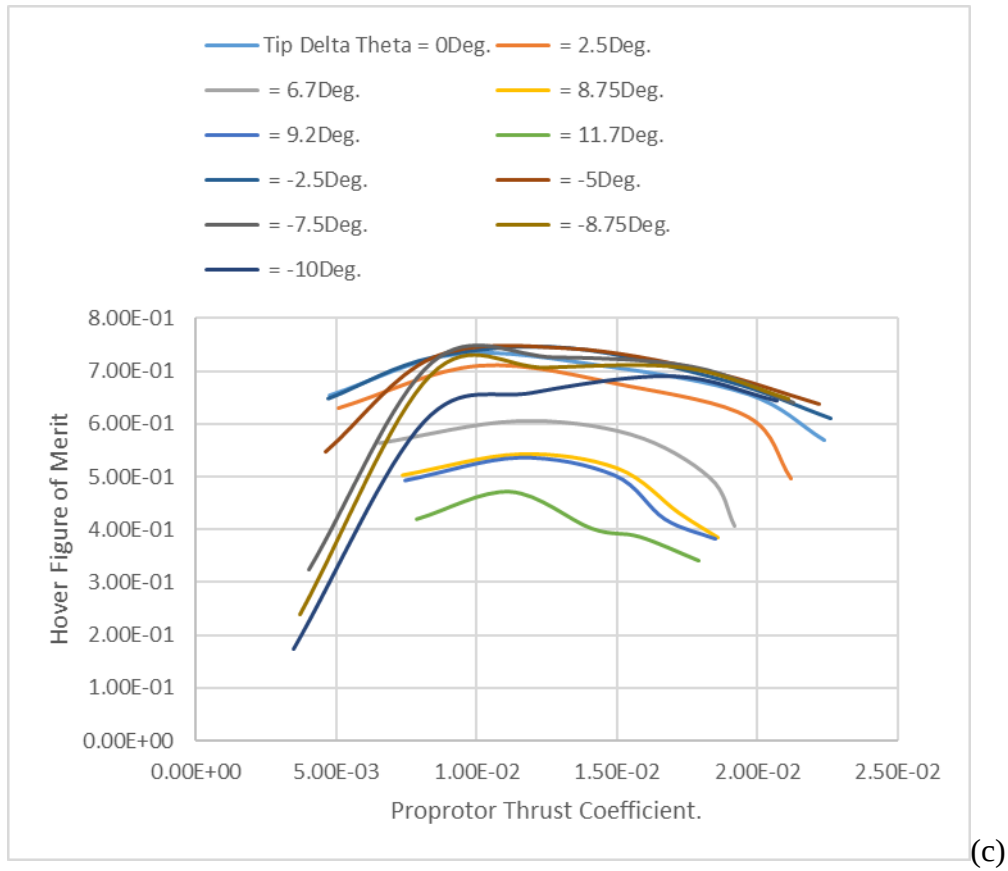
Figure 36. Hover performance curves for various different indexed-tip \Delta\theta angles (untwisted tip) against the baseline rotor: (a) thrust coefficient vs. rotor collective, (b) torque coefficient vs. collective, and (c) figure of merit vs. thrust coefficient.
