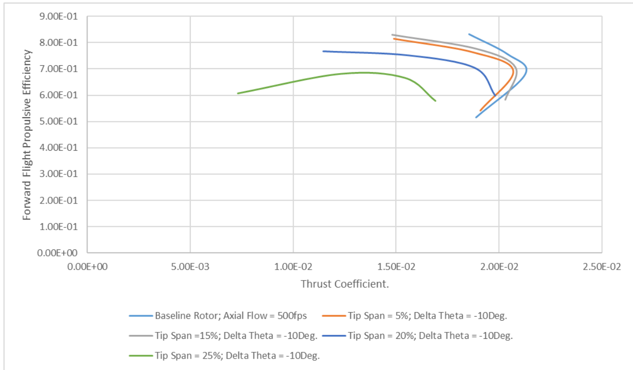
Figure 65. Cruise propulsive efficiency as a function of rotor thrust coefficient, for \Delta\theta = -10 degrees, for different tip spans (percent rotor radius) for axial-flow cruise speed of 500 fps.
