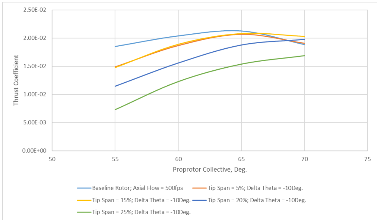
Figure 63. Thrust coefficient as a function of rotor collective, for \Delta\theta = -10 degrees, for different tip spans (percent of rotor radius) for an axial-flow cruise speed of 500 fps.
