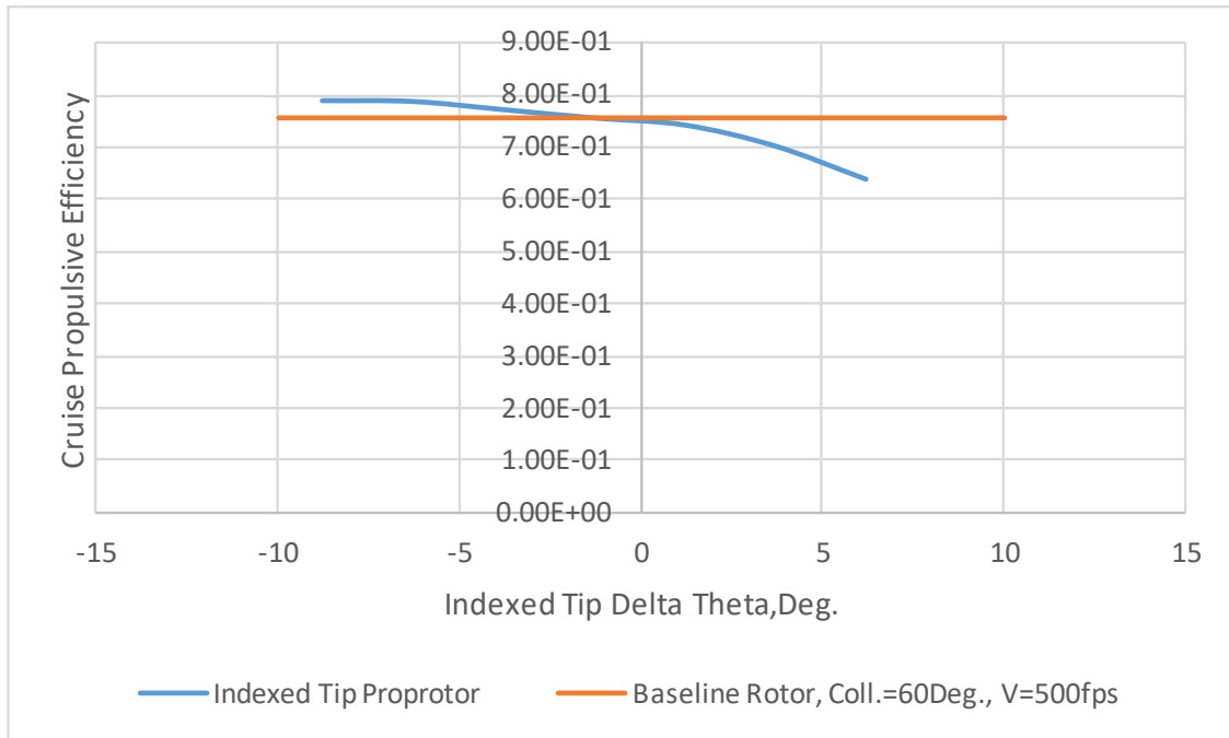
Figure 25. Cruise/axial-flow propulsive efficiency trend (for an untwisted indexed-tip) as a function of indexed-tip \Delta\theta (Coll. = 60 degrees and V=500 fps).
