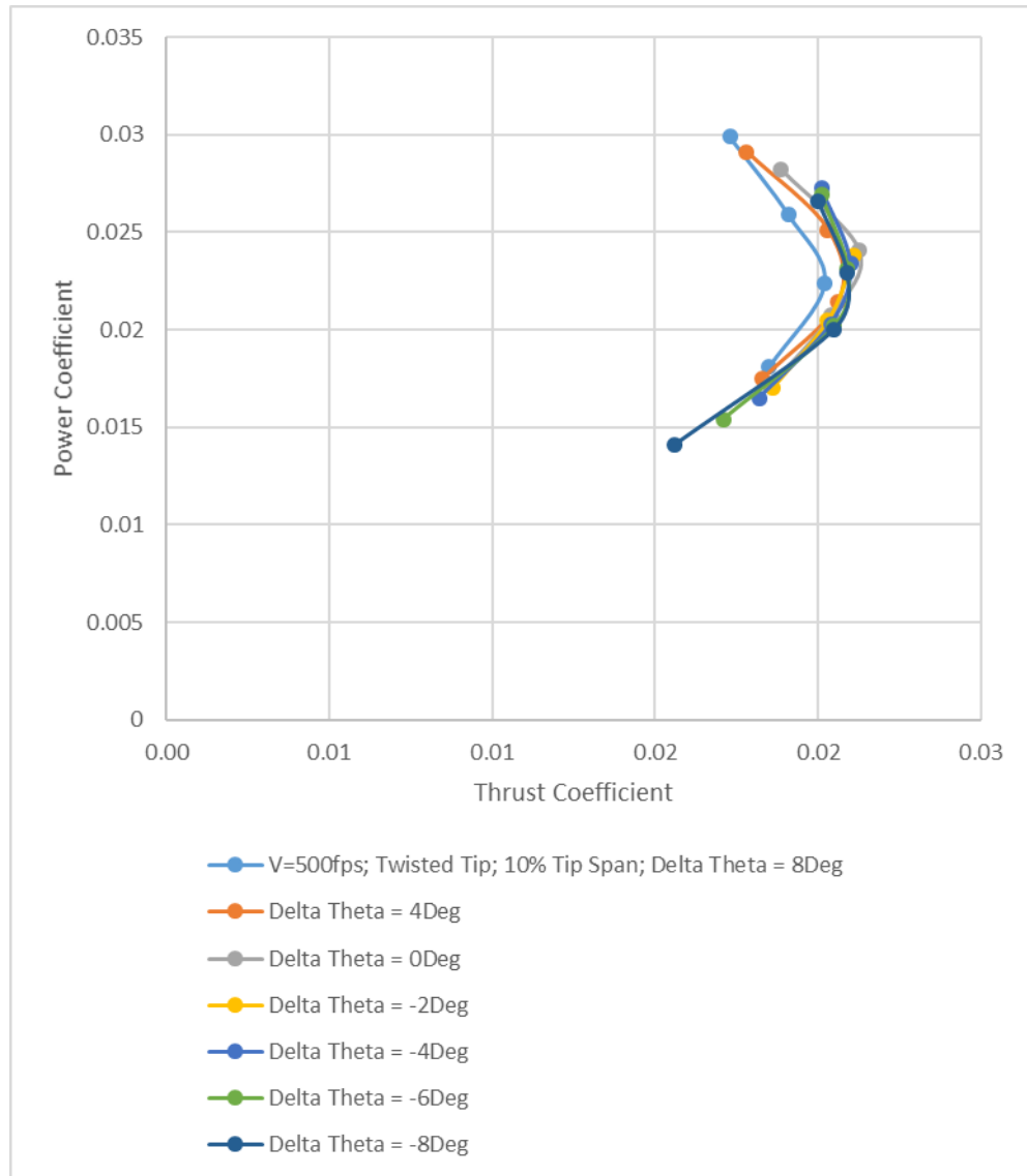
Figure 46. Power coefficient versus rotor thrust coefficient at an axial-flow cruise speed of 500 fps for different values of \Delta\theta .
