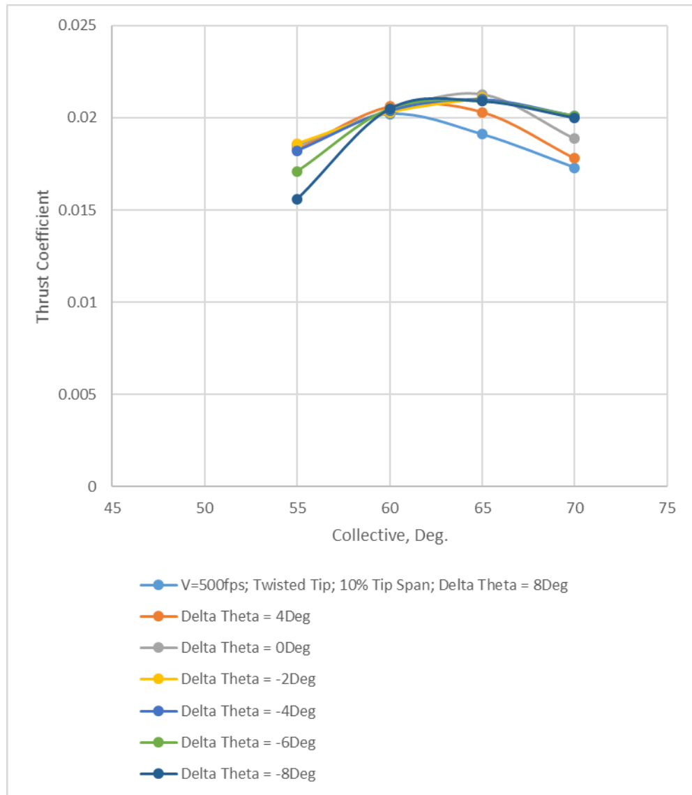
Figure 44. Thrust coefficient versus rotor collective at an axial-flow cruise speed of 500 fps for different values of \Delta\theta .
