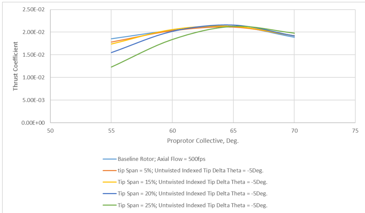
Figure 60. Thrust coefficient as a function of rotor collective, for \Delta\theta = -5 degrees, for different tip spans (percent of rotor radius) for an axial-flow cruise speed of 500 fps.
