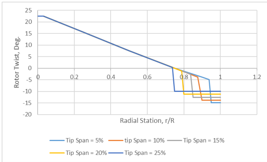
Figure 51. Rotor twist distributions for various (untwisted) indexed-tip tip-spans (constant \Delta\theta = -10 degrees for all twist distributions).
