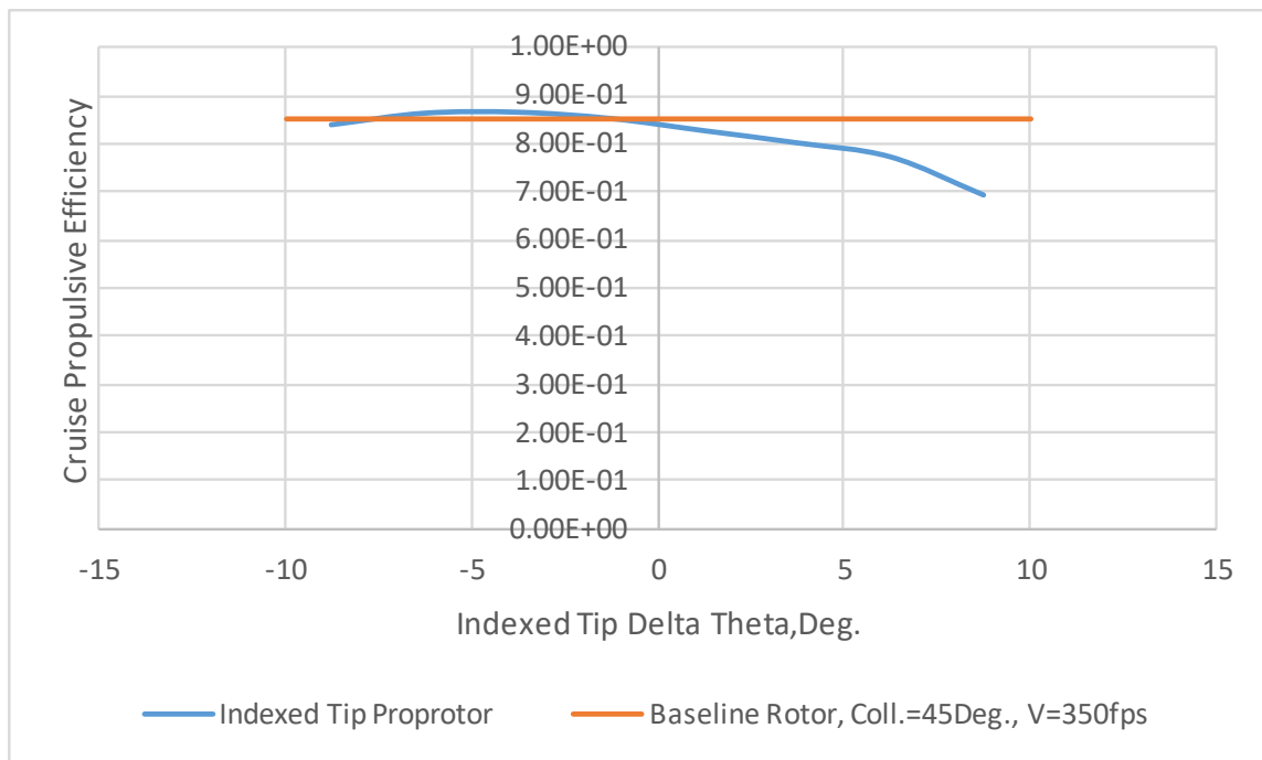
Figure 22. Cruise propulsive efficiency trends as a function of indexed-tip \Delta\theta against the baseline rotor ( V=350 fps).
