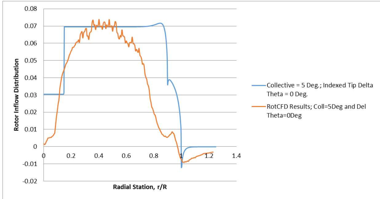
Figure 11. RotCFD and Prandtl-type superposition analysis for hover inflow radial distribution at \theta=5 and \Delta\theta_{Tip}=0 .
