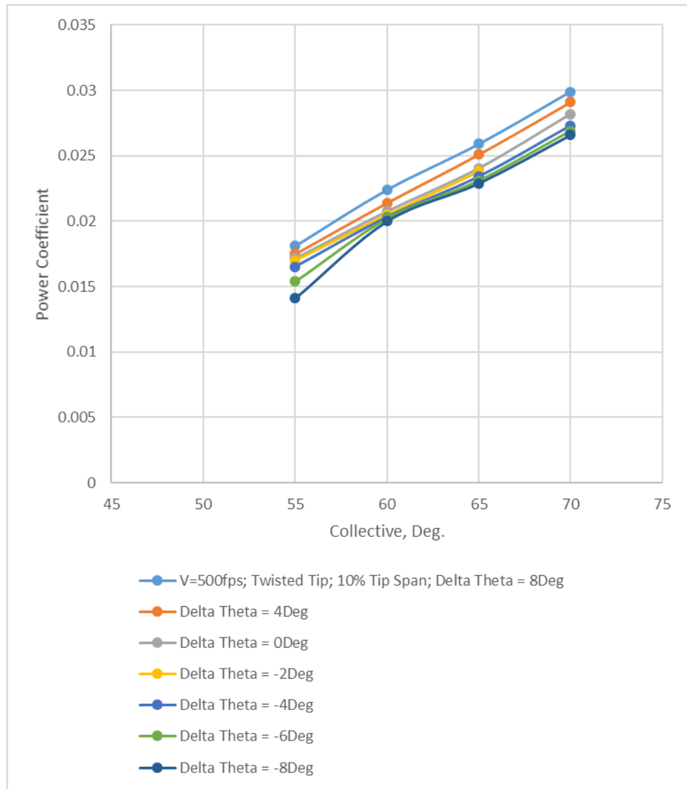
Figure 45. Power coefficient versus rotor collective at an axial-flow cruise speed of 500 fps for different values of \Delta\theta .
