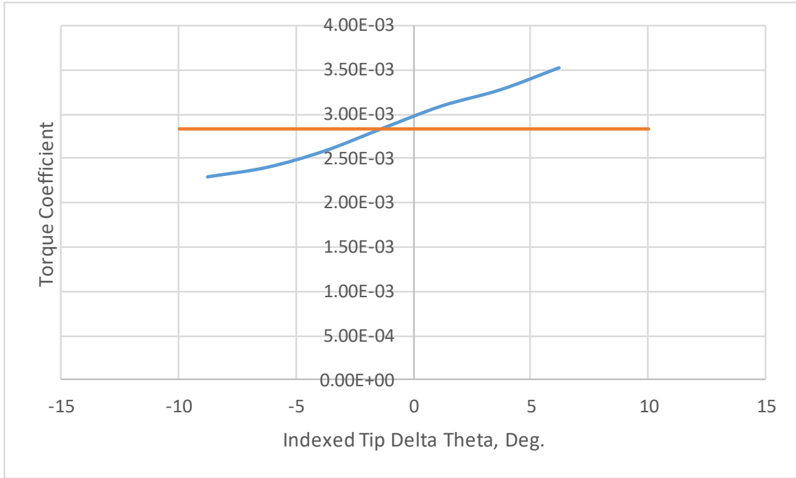
Figure 15. Torque coefficient trend (for an untwisted indexed-tip) as a function of indexed-tip \Delta\theta .
