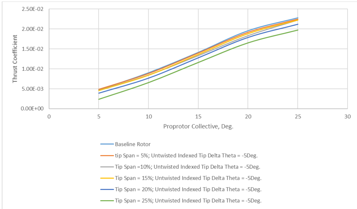
Figure 54. Thrust coefficient as a function of rotor collective, for \Delta\theta = -5 degrees, for different tip spans (percent of rotor radius).
