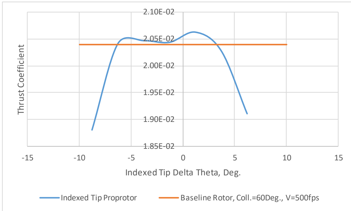
Figure 23. Cruise/axial-flow thrust coefficient trend (for an untwisted indexed-tip) as a function of indexed-tip \Delta\theta (Coll. = 60 degrees and V=500 fps).
