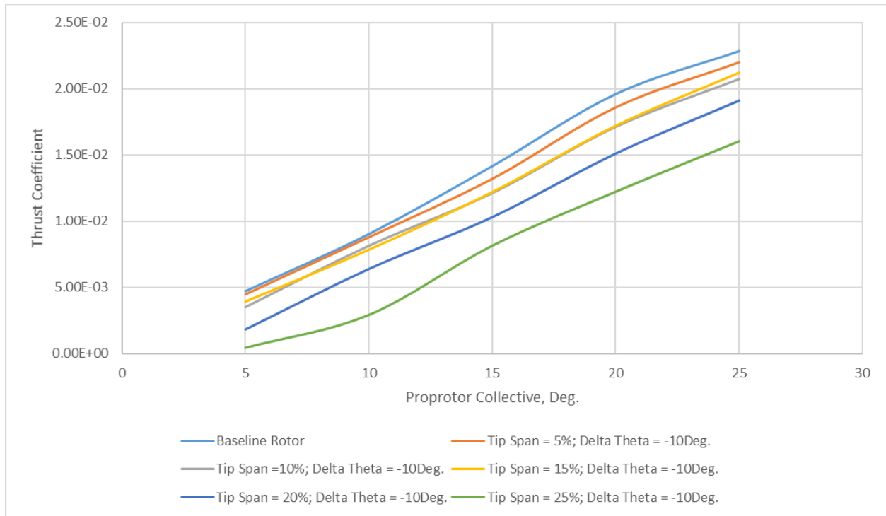
Figure 57. Thrust coefficient as a function of rotor collective, for \Delta\theta = -10 degrees, for different tip spans (percent of rotor radius).
