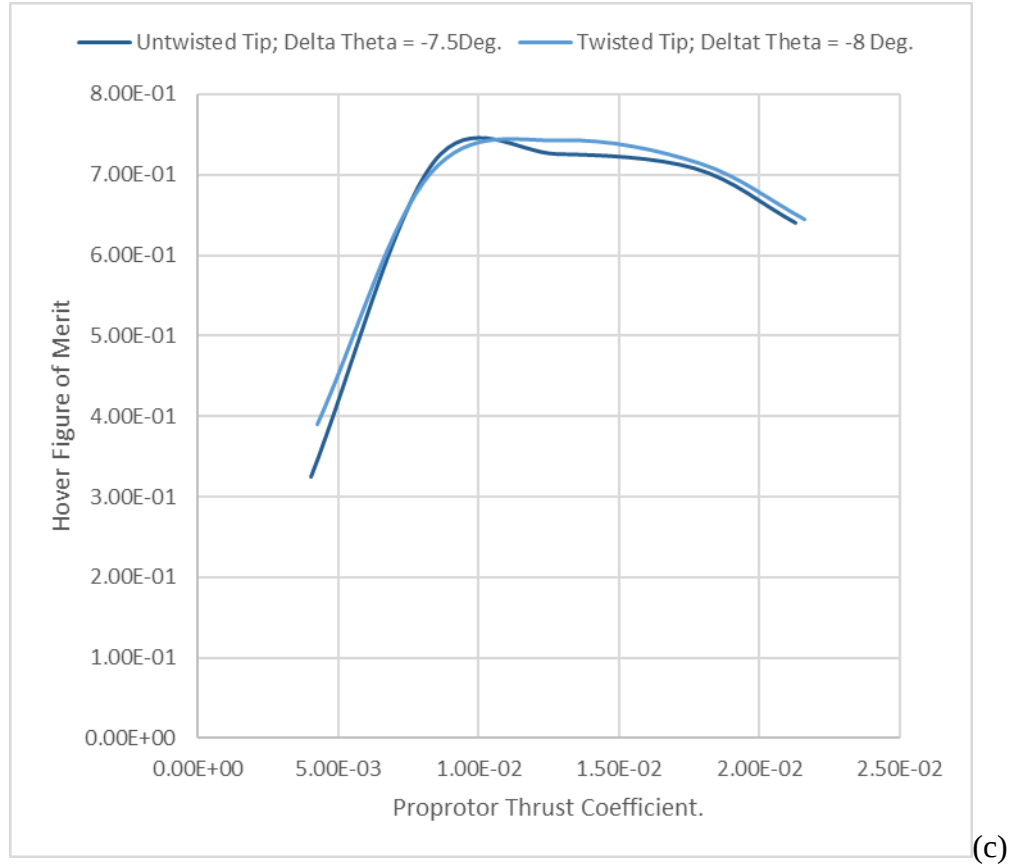
Figure 38. Hover performance comparison between twisted versus untwisted indexed-tips (at \Delta\theta \sim -7.5 to -8 degrees): (a) thrust coefficient vs. collective, (b) torque coefficient vs. collective, and (c) figure of merit vs. thrust coefficient.
