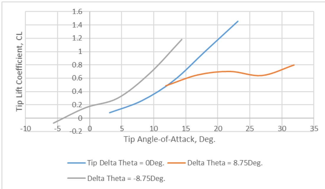
Figure 29. Tip lift coefficient curve as a function of tip angle of attack for three different indexed-tip \Delta\theta .
