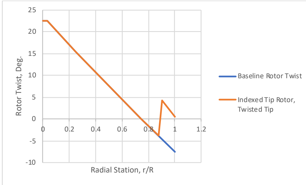
Figure 34. Alternative rotor twist distribution: baseline rotor and 10-percent span indexed-tip (with continuation of linear twist rate across tip) set at 4.16 degrees tip-twist ( \Delta\theta Tip = +8 degrees).
