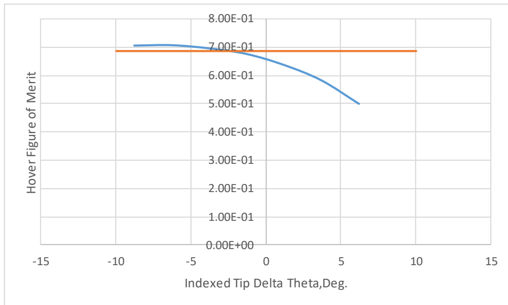
Figure 16. Figure of merit (for an untwisted indexed-tip) as a function of indexed-tip \Delta\theta .
