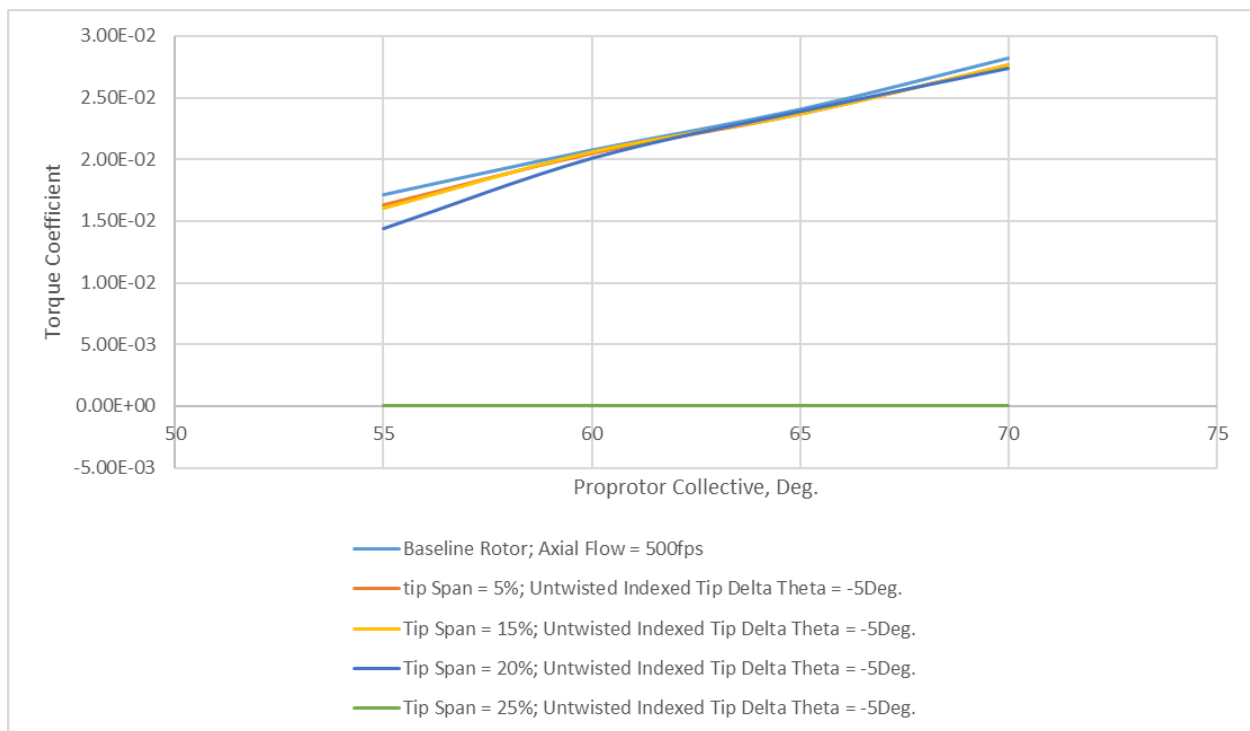
Figure 61. Torque coefficient as a function of rotor collective, for \Delta\theta = -5 degrees, for different tip spans (percent of rotor radius) for an axial-flow cruise speed of 500 fps.
