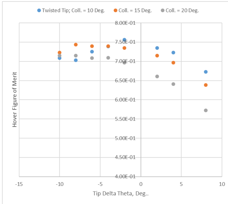
Figure 39. Influence of \Delta\theta on indexed-tip proprotor hover figure of merit for various rotor collectives (for twisted indexed-tips).
