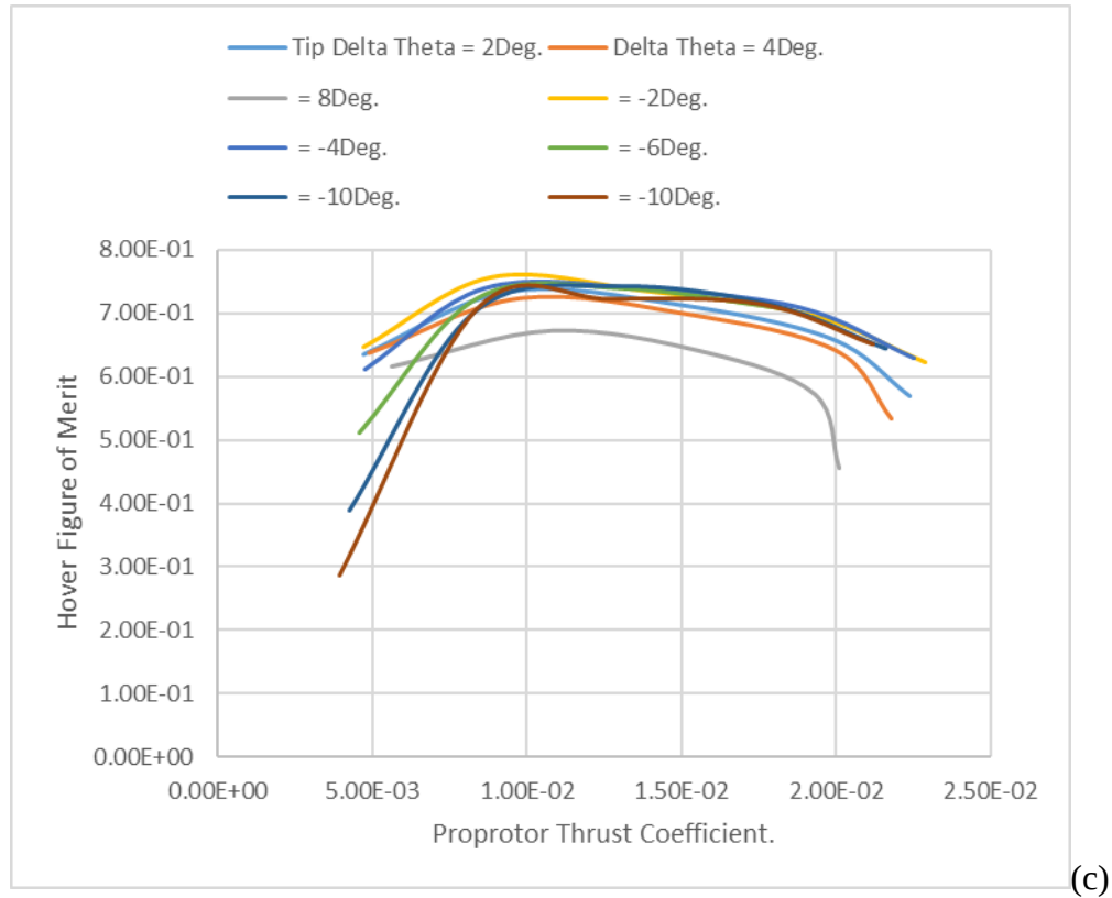
Figure 35. Hover performance curves for various indexed-tip \Delta\theta angles (twisted tip): (a) thrust coefficient vs. rotor collective, (b) torque coefficient vs. collective, and (c) figure of merit vs. thrust coefficient.
