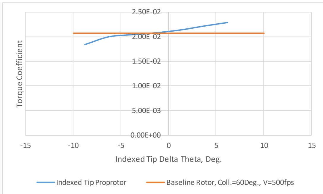
Figure 24. Cruise/axial-flow torque coefficient trend (for an untwisted indexed-tip) as a function of indexed-tip \Delta\theta (Coll. = 60 degrees and V=500 fps).
