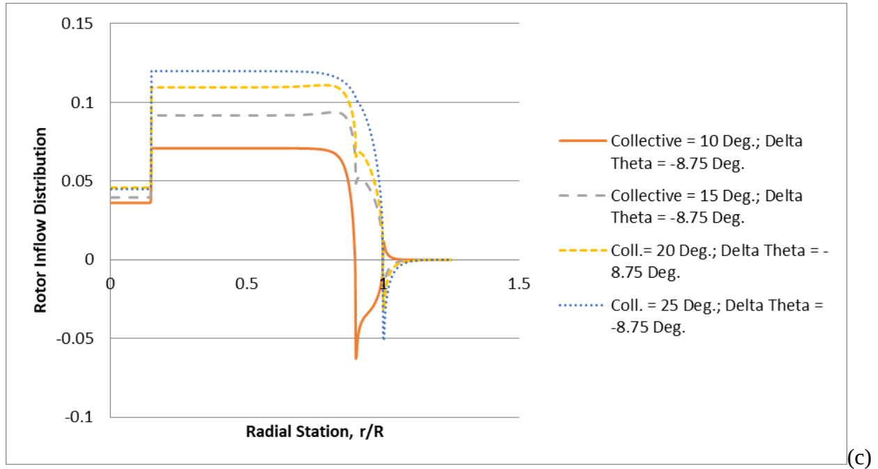
Figure 4. Inflow distributions for various indexed-tip \Delta\theta and rotor collectives: (a) \Delta\theta = 0 degree, (b) \Delta\theta = 8.75 degrees, and (c) \Delta\theta = -8.75 degrees.
