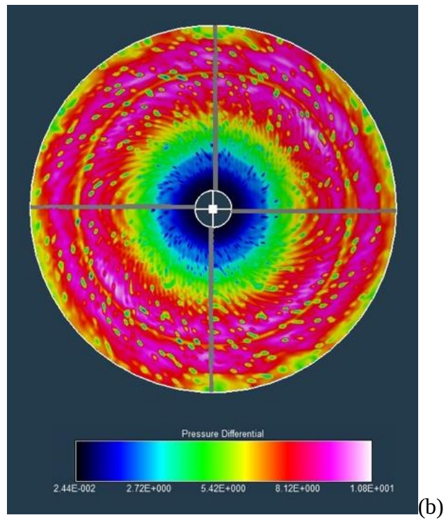
Figure 6. Representative hover results (differential-pressure across the rotor disk, collective = 20 degrees) for LCTR2 proprotor (Ref. 14): (a) baseline rotor and (b) 10-percent span indexed-tip set at 5 degrees tip-twist.
