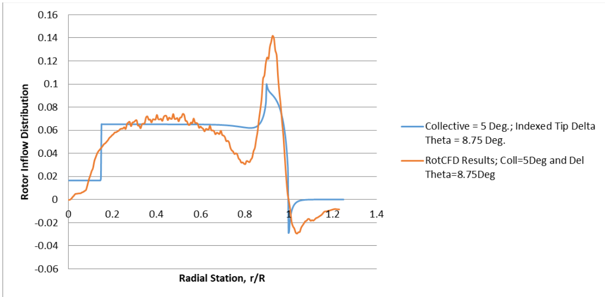
Figure 12. RotCFD and Prandtl-type superposition analysis for hover inflow radial distribution at \theta=5 and \Delta\theta_{Tip} = 8.75 .
