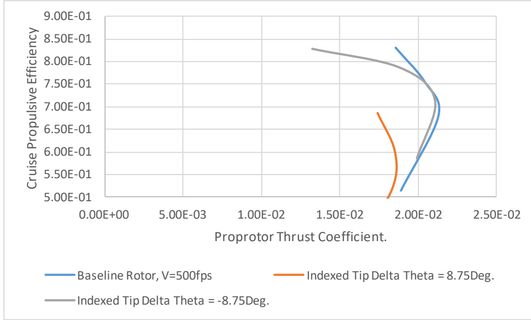
Figure 28. Cruise/axial-flow propulsive efficiency trends for two different \Delta\theta values as compared to baseline rotor results ( V=500 fps).
