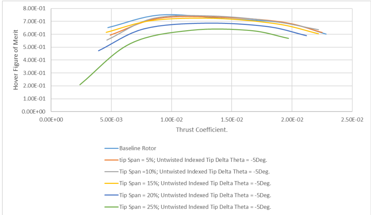
Figure 56. Hover figure of merit as a function of rotor thrust coefficient, for \Delta\theta = -5 degrees, for different tip spans (percent of rotor radius).
