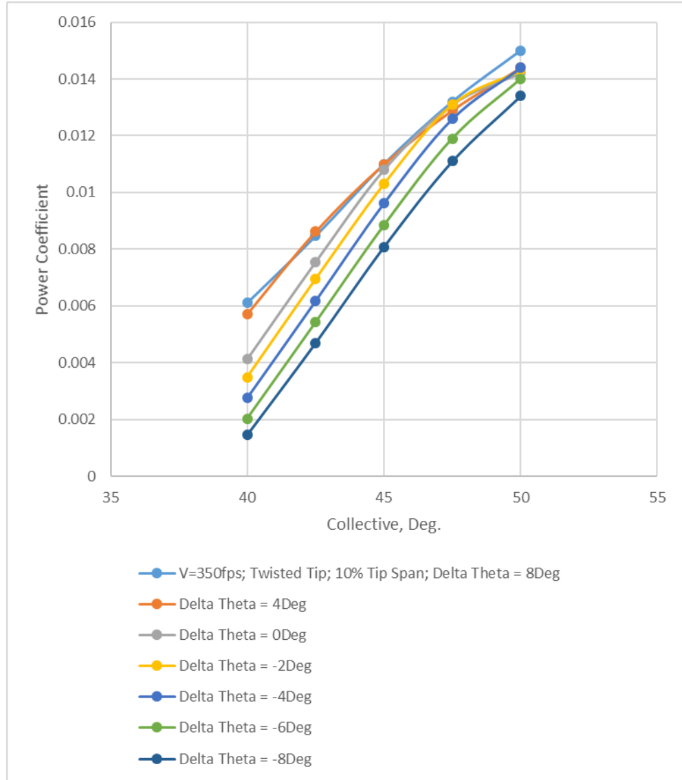
Figure 42. Power coefficient versus rotor collective at an axial-flow cruise speed of 350 fps for different values of \Delta\theta .
