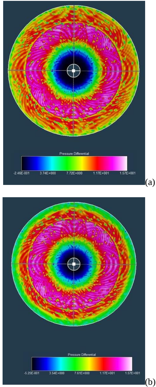
Figure 7. Representative cruise axial-flow results (differential-pressure across the rotor disk, collective = 60 degrees at V=500 fps) for LCTR2 proprotor (Ref. 14): (a) baseline rotor and (b) 10-percent span indexed-tip set at 5 degrees tip-twist.
