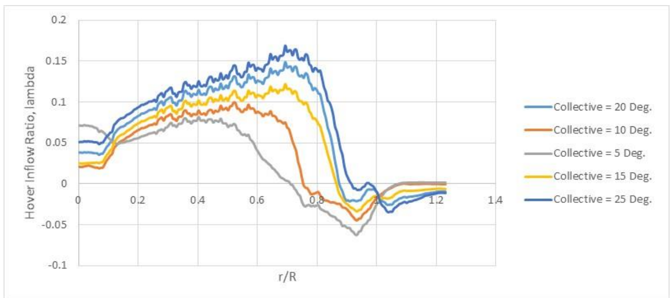
Figure 10. Collective sweep showing CFD rotor inflow results for \Delta\theta_{\text{Tip}} = -8.75 degrees with untwisted tip outer-span.
