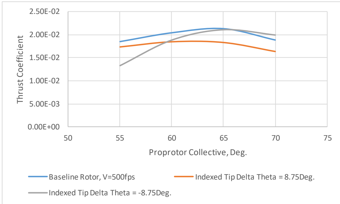
Figure 26. Cruise/axial-flow thrust coefficient trends for two different \Delta\theta values as compared to baseline rotor results ( V=500 fps).
