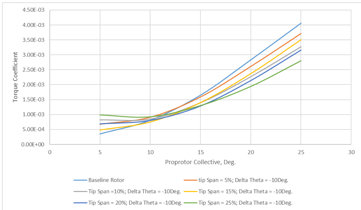
Figure 58. Rotor torque coefficient as a function of rotor collective, for \Delta\theta = -10 degrees, for different tip spans (percent of rotor radius).
