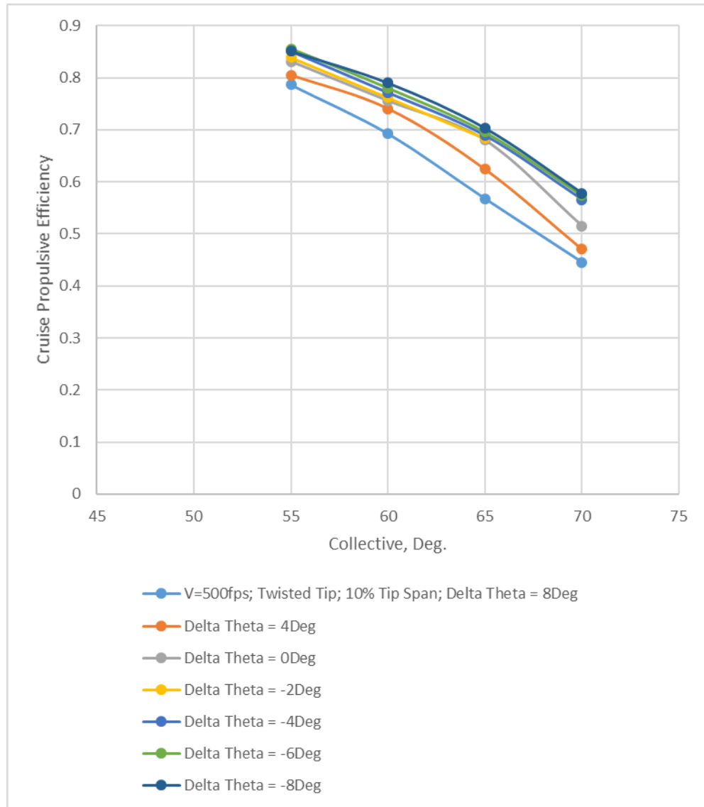
Figure 49. Cruise propulsive efficiency as a function of rotor collective for twisted indexed-tips (10-percent span) for axial-flow cruise speed of 500 fps for different \Delta\theta .
