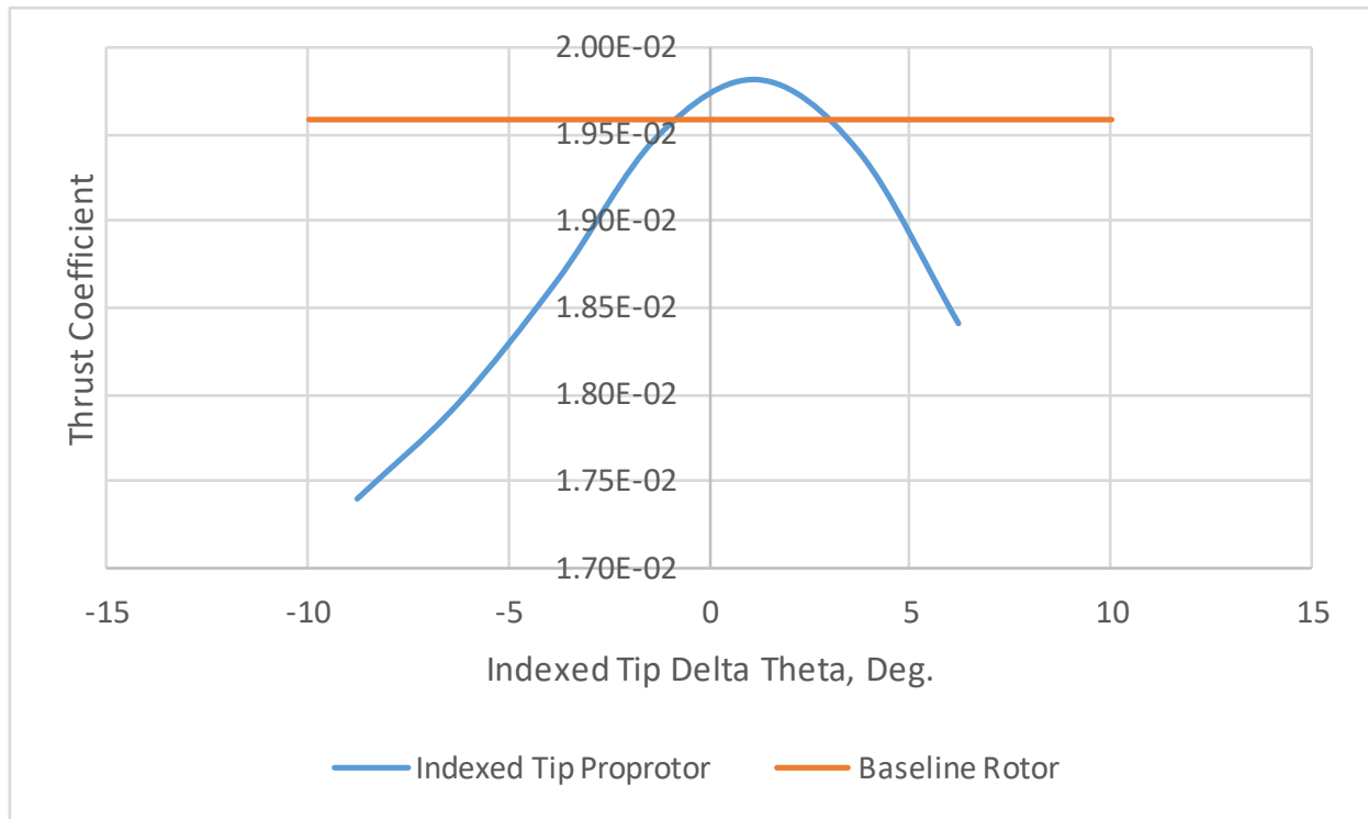
Figure 14. Thrust coefficient trend comparison between indexed tip proprotor as a function of indexed-tip \Delta\theta and a baseline rotor.
