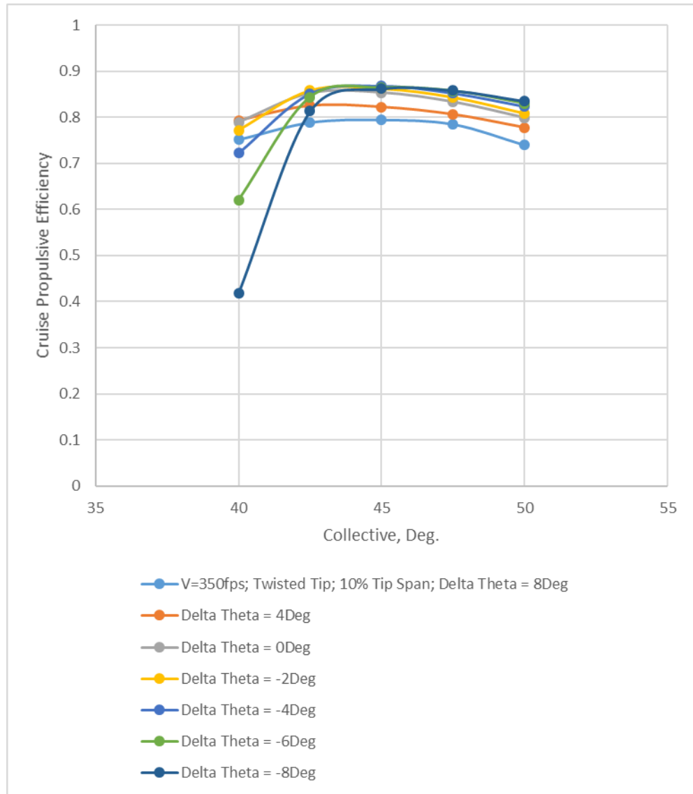
Figure 47. Cruise propulsive efficiency as a function of rotor collective, for axial-flow cruise speed of 350 fps, for twisted indexed-tips (for 10-percent span) for different \Delta\theta .
