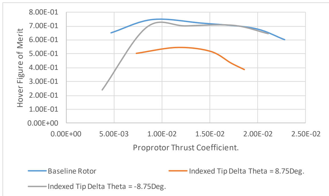
Figure 19. Hover figure-of-merit curves for various different indexed-tip \Delta\theta angles against the baseline rotor.
