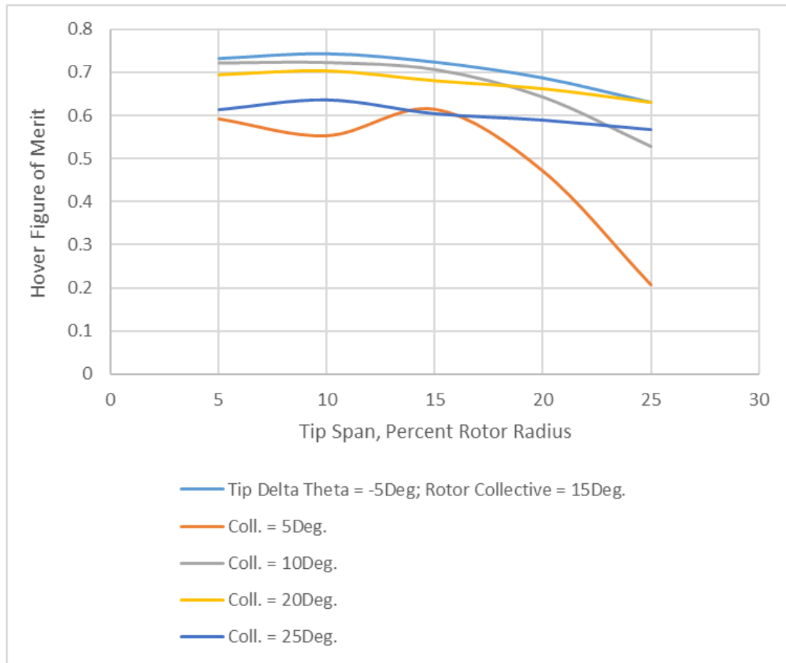
Figure 52. Effect of untwisted tip span for a \Delta\theta = -5 degrees for different rotor collectives for hover.
