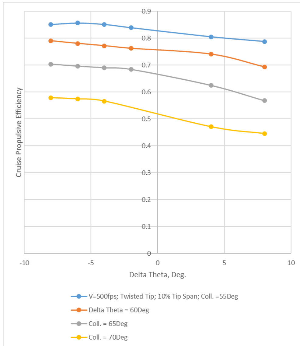
Figure 50. Cruise propulsive efficiency as a function of \Delta\theta for twisted indexed-tips (10-percent span) for axial-flow cruise speed of 500 fps for different rotor collectives.
