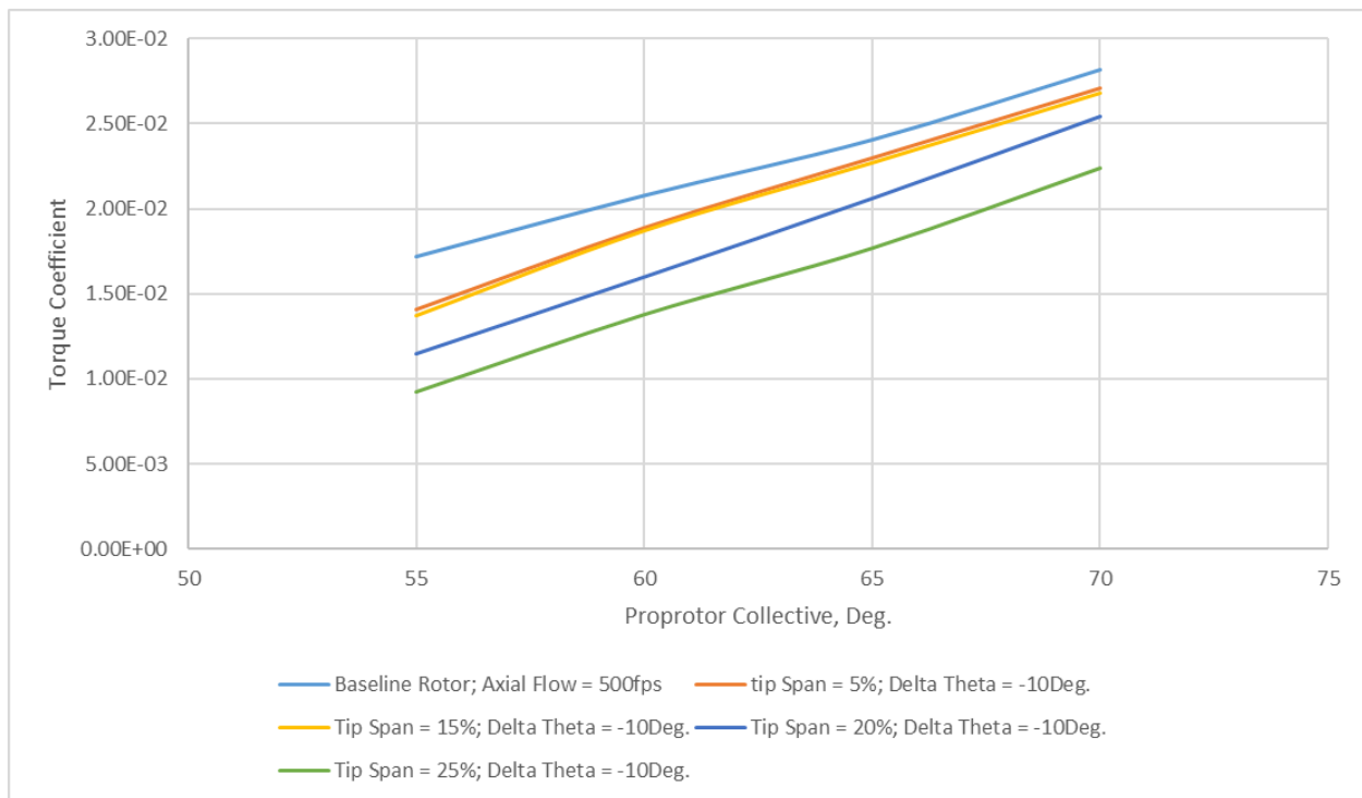
Figure 64. Torque coefficient as a function of rotor collective, for \Delta\theta = -10 degrees, for different tip spans (percent of rotor radius) for an axial-flow cruise speed of 500 fps.
