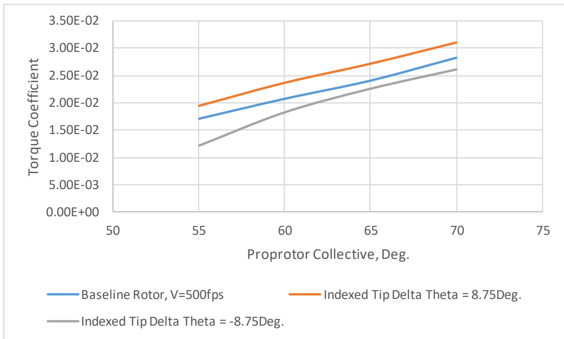
Figure 27. Cruise/axial-flow torque coefficient trends for two different \Delta\theta values as compared to baseline rotor results ( V=500 fps).
