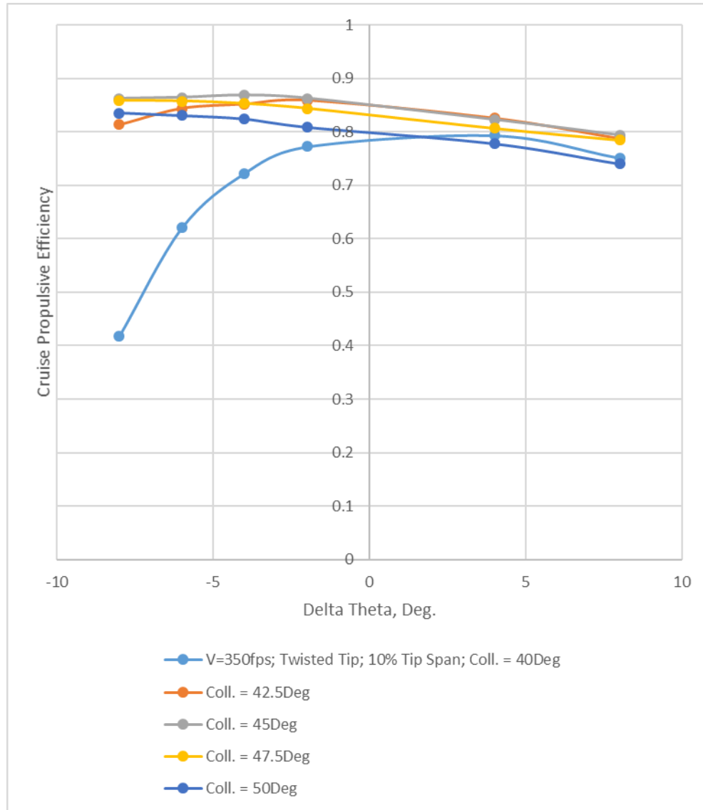
Figure 48. Cruise propulsive efficiency as a function of \Delta\theta for twisted indexed-tips (10-percent span) for axial-flow cruise speed of 350 fps for different rotor collectives.
