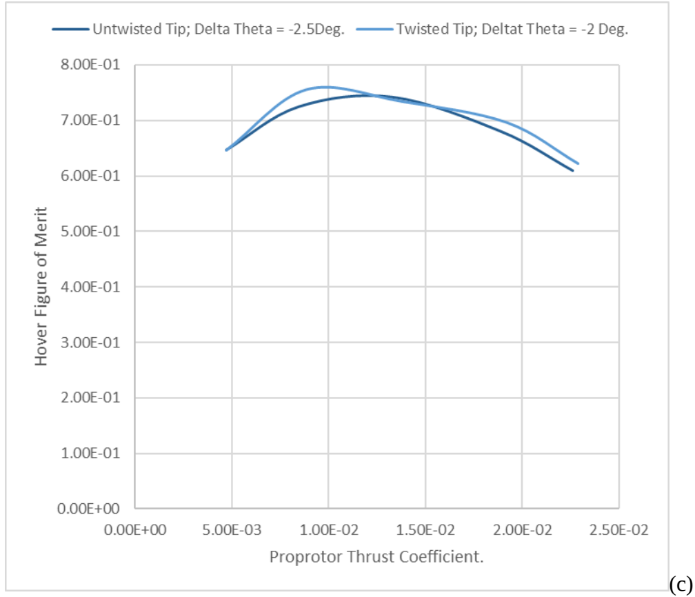
Figure 37. Hover performance comparison between twisted versus untwisted indexed-tips (at \Delta\theta \sim -2 to -2.5 degrees): (a) thrust coefficient vs. collective, (b) torque coefficient vs. collective, and (c) figure of merit vs. thrust coefficient.
