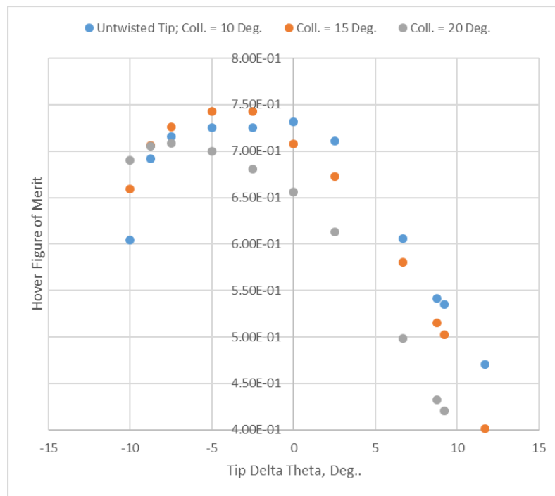
Figure 40. Influence of \Delta\theta on indexed-tip proprotor hover figure of merit for various rotor collectives (for untwisted indexed-tips).
