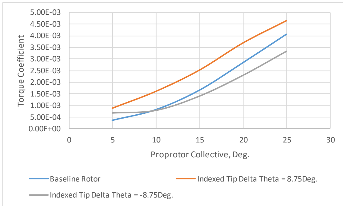
Figure 18. Hover power coefficient trends with collective at two different indexed-tip \Delta\theta .
