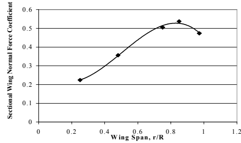
Fig. 26 – Representative Sectional Normal Force Coefficient Spanwise Distribution
