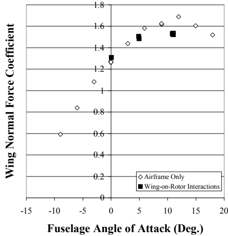
Fig. 21 – Effect of Rotor-on-Wing Interactions on Wing Normal Force Coefficients
