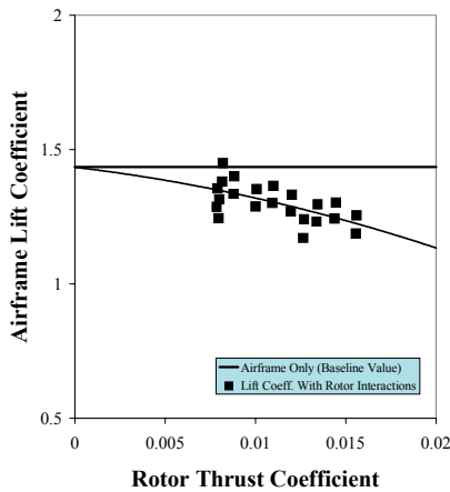
Fig. 19 – Influence of Rotor Thrust on Tiltrotor Airframe Lift
