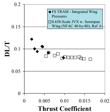
Fig. 10 – Qualitative Data Comparison Between Tiltrotor Hover Download Tests/Configurations
