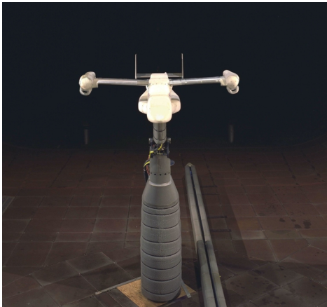
Fig. 22 – Full-Span TRAM in Airplane-Mode (Rotors Off)
