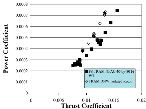
Fig. 16 -- Wing/Airframe on Rotor Interactions in Helicopter Mode Forward Flight ( M_{Tip} = 0.63 , \mu=0.15 , \alpha_F = +11 deg., and \alpha_S = +6 deg.)
