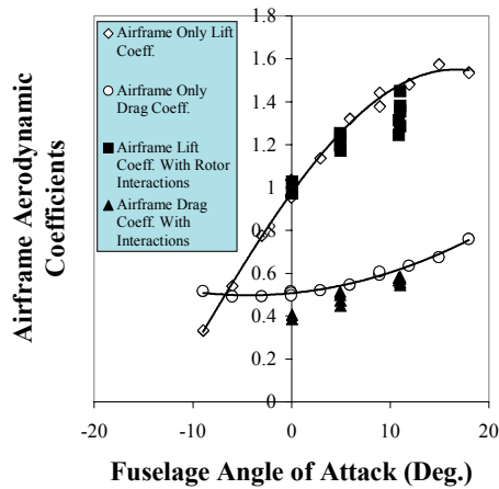
Fig. 18 – Influence of Rotor on Wing/Airframe Interactions on Airframe Lift and Drag
