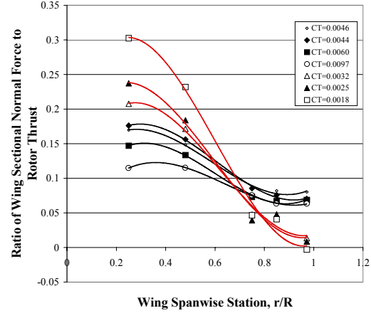
Fig. 12– Wing Sectional Download Distribution as a Function of Rotor Thrust Coefficient
