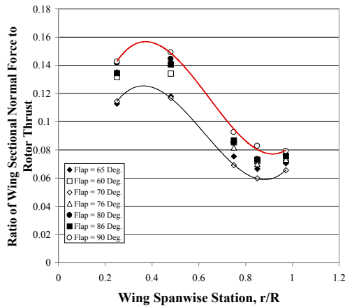
Fig. 14—Wing Download Distribution as a Function of Wing Flaperon Angle (CT=0.008)
