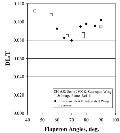
Fig. 13 – Tiltrotor Download as a Function of Flaperon Angles
