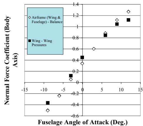
Fig. 27 – Airframe Versus Wing Normal Force Coefficient Contribution ( i_N = 0 deg., \delta_f = 0 deg., \delta_e = -17 deg., V = 104 knots, Re = 2.3 \times 10^6 )
