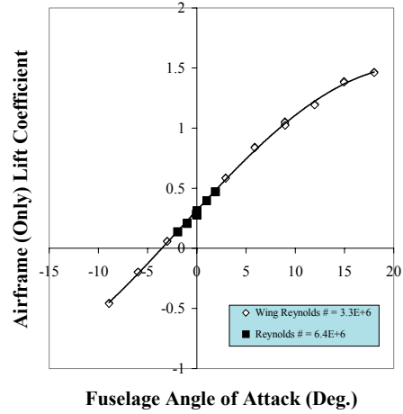
Fig. 23 – TRAM Airframe-Only Airplane-Mode Lift Curves
