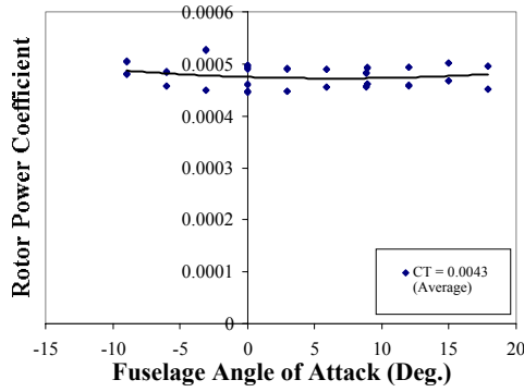
Fig. 6 – Influence of Wind Tunnel Test Section Interactions in Hover
