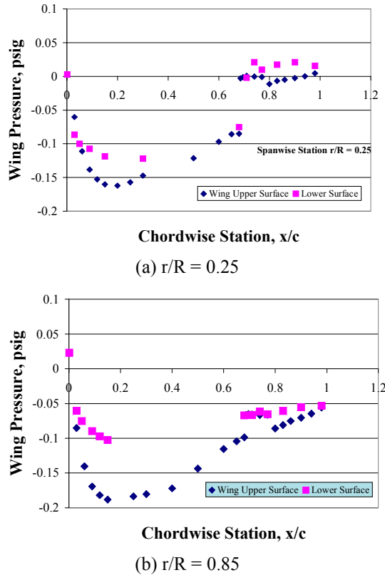
Fig. 25a-b – Representative Airplane-Mode Forward-Flight (Rotors-Off) Wing Pressure Distributions
