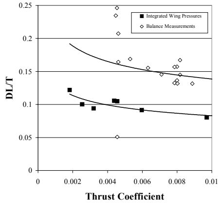
Fig. 11 – Hover Download as a Function of Thrust Coefficient
