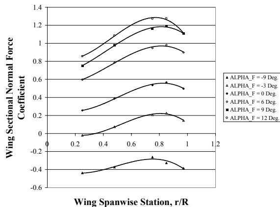
Fig. 28 – Influence of Fuselage Angle of Attack on Wing Spanwise Distributions
