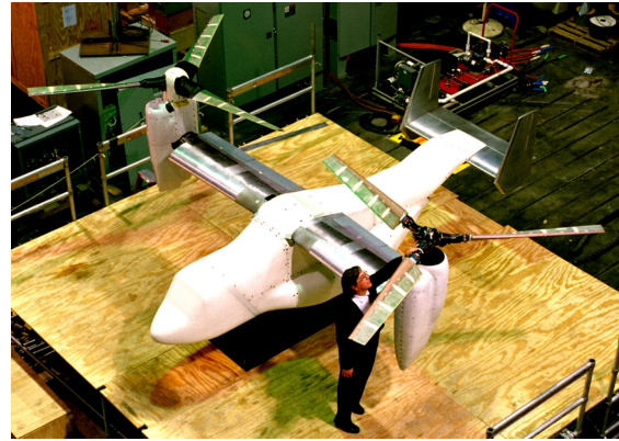
Fig. 2 -- Full-span TRAM configuration (Prior to NFAC Tunnel Entry)
