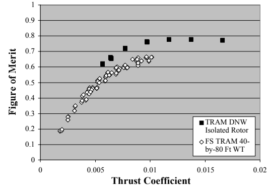
Fig. 7 – Influence of Wing/Airframe on Rotor Hover Performance
