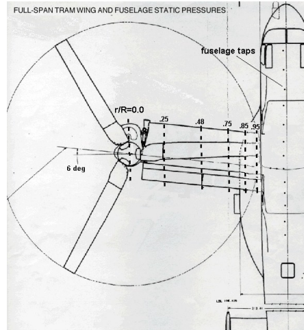
Fig. 3 – Planform View of TRAM Wing and Spanwise Location of Static Pressure Taps
