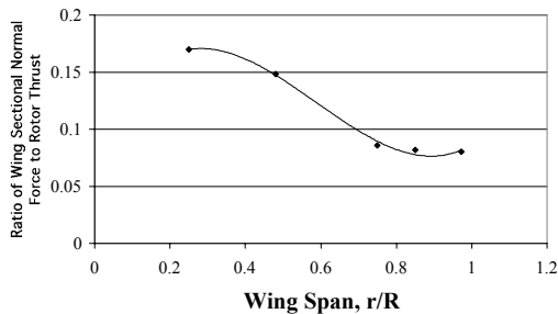
Fig. 9 – Representative Wing Integrated Sectional Download Results ( C_T=0.0046 )
