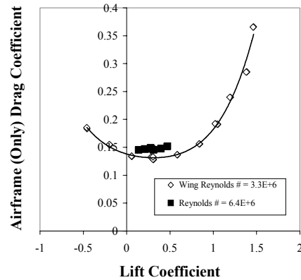
Fig. 24 – TRAM Airframe-Only Airplane-Mode Lift/Drag Polar
