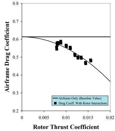
Fig. 20 -- Influence of Rotor Thrust on Tiltrotor Airframe Drag
