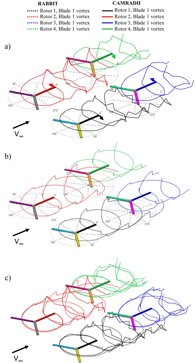
Figure 14. Quadrotor shed tip vortex comparison for one blade for a) CAMRADII, b) RABBIT, and c) CAMRADII and RABBIT ( \mu = 0.169 , \alpha_{TPP} = -2.49^\circ , and C_T = 0.0063 , 0.0063 , 0.0058 , 0.0058 ).
