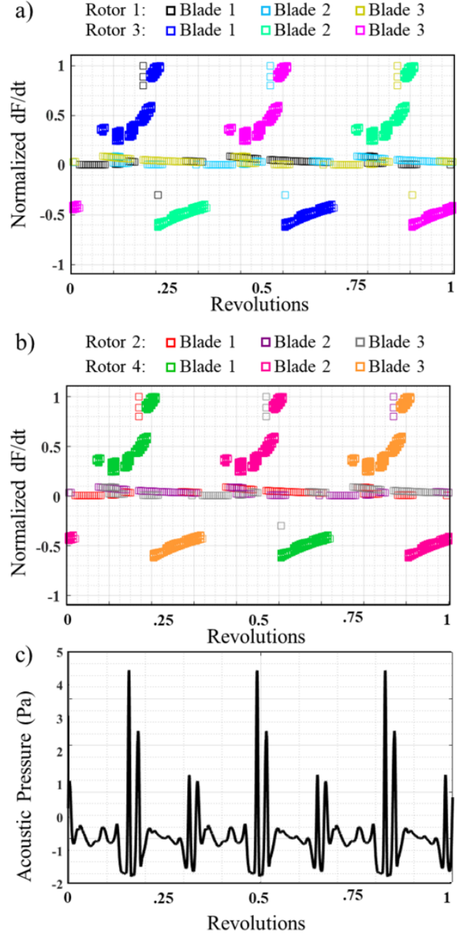
Figure 16. a) RABBIT normalized time rate change of loading for Rotors 1 and 3; b) RABBIT normalized time rate change of loading for Rotors 2 and 4; and c) ANOPP2/AARON acoustic pressure for a microphone at (10R, 0, -15R) shifted by 0.153 sec ( \mu = 0.169 , \alpha_{TPP} = -2.49^\circ , and C_T = 0.0063, 0.0063, 0.0058, 0.0058 ).
