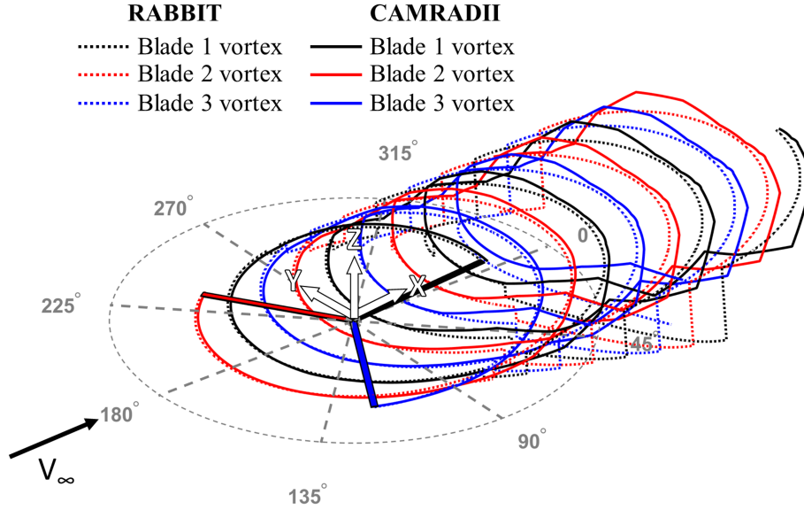
Figure 5. QSMR shed tip vortex comparison between RABBIT and CAMRADII for all blades ( \mu = 0.121 , \alpha_{TPP} = -4 , and C_T = 0.0015 ).
