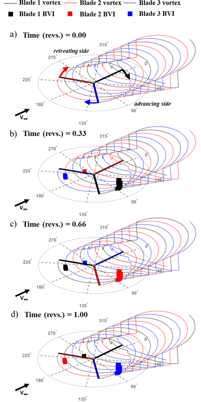
Figure 8. QSMR BVI location in RABBIT at a time (rev) of a) 0.00, b) 0.33, c) 0.66, and d) 1.00 ( \mu = 0.121 , \alpha_{TPP} = -4^\circ , and C_T = 0.0015 ).
