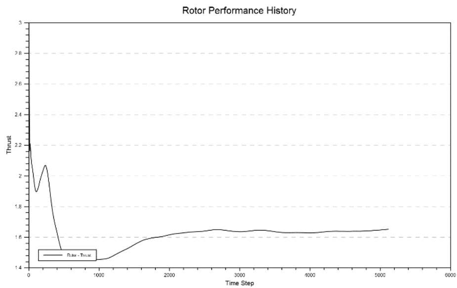
Figure C40. 14-mbar 1-Stack test 8 full thrust.
