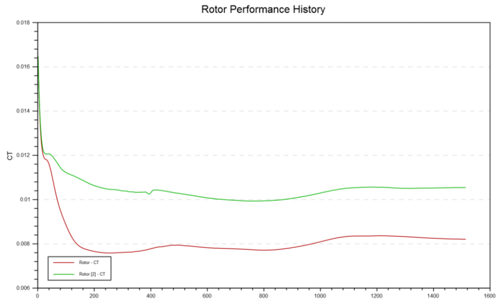
Figure C31. 1013-mbar 2-Stack test 6 isol thrust.
