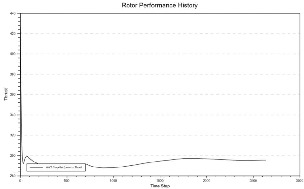
Figure C16. 1013-mbar 1-Stack test 10 full thrust.
