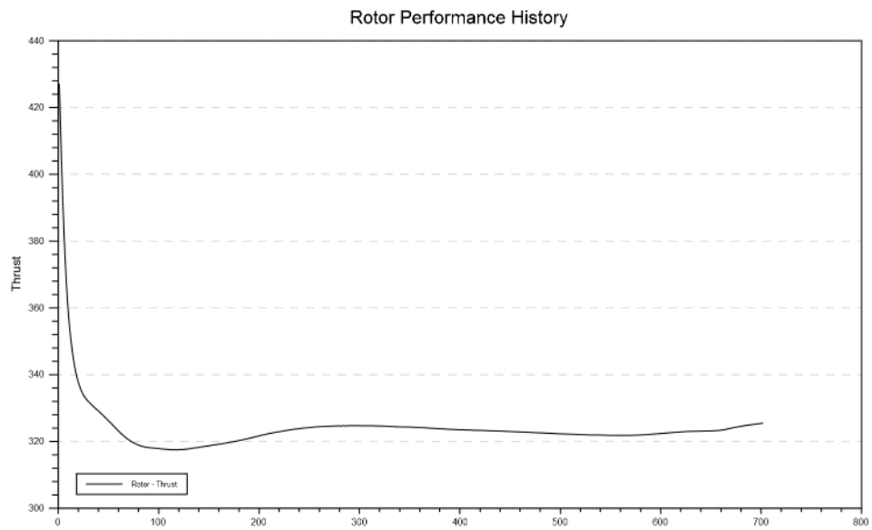
Figure C9. 1013-mbar 1-Stack test 6 isol thrust.
