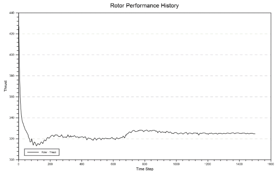
Figure C4. 1013-mbar 1-Stack test 1 isol thrust graph.
