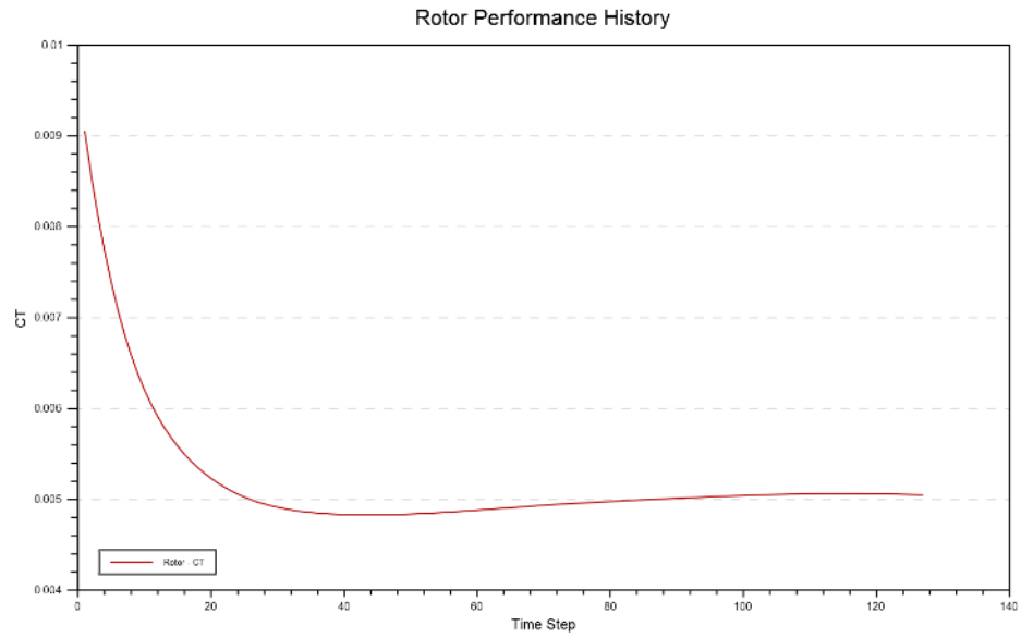
Figure C33. 14-mbar 1-Stack test 1 isol CT.
