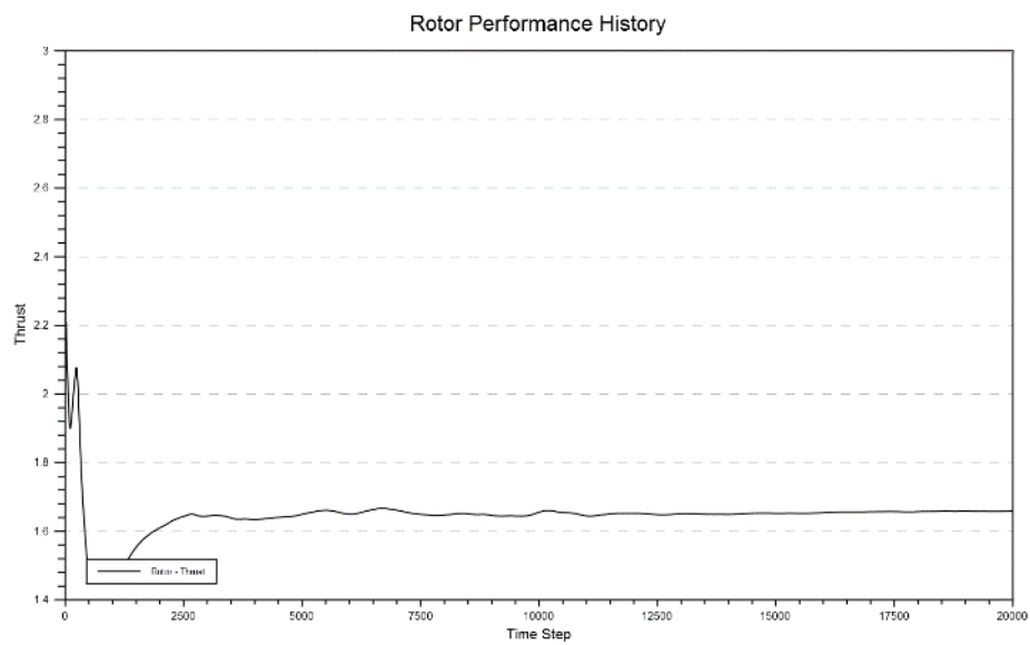
Figure C44. 14-mbar 1-Stack test 10 full thrust.
