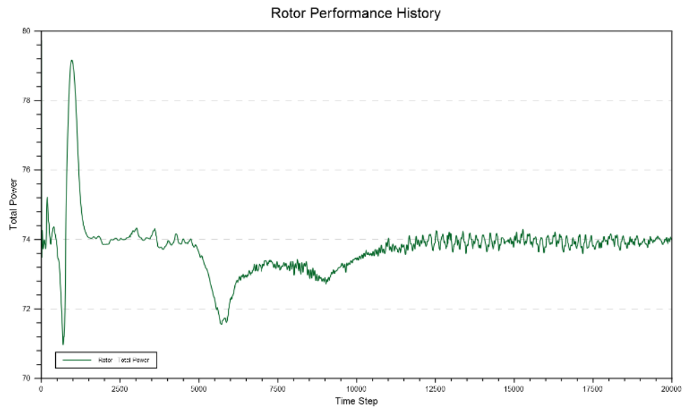
Figure C48. 14-mbar 1-Stack test 12 Laser Lab total power.
