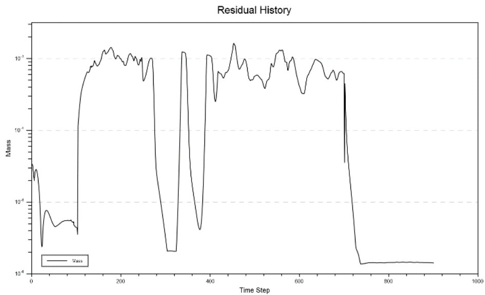
Figure C18. 1013-mbar 2-Stack test 1 isol residual.
