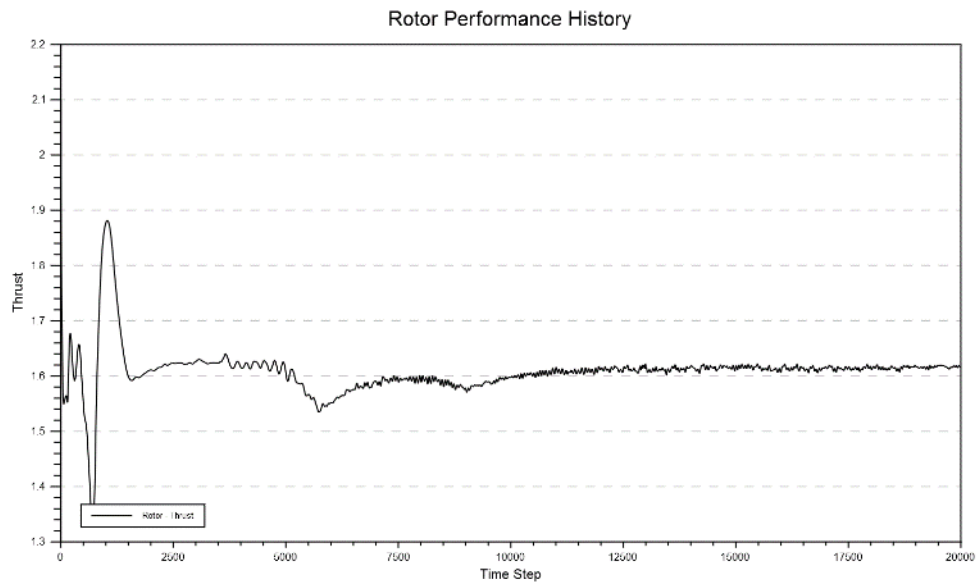
Figure C47. 14-mbar 1-Stack test 12 Laser Lab thrust.
