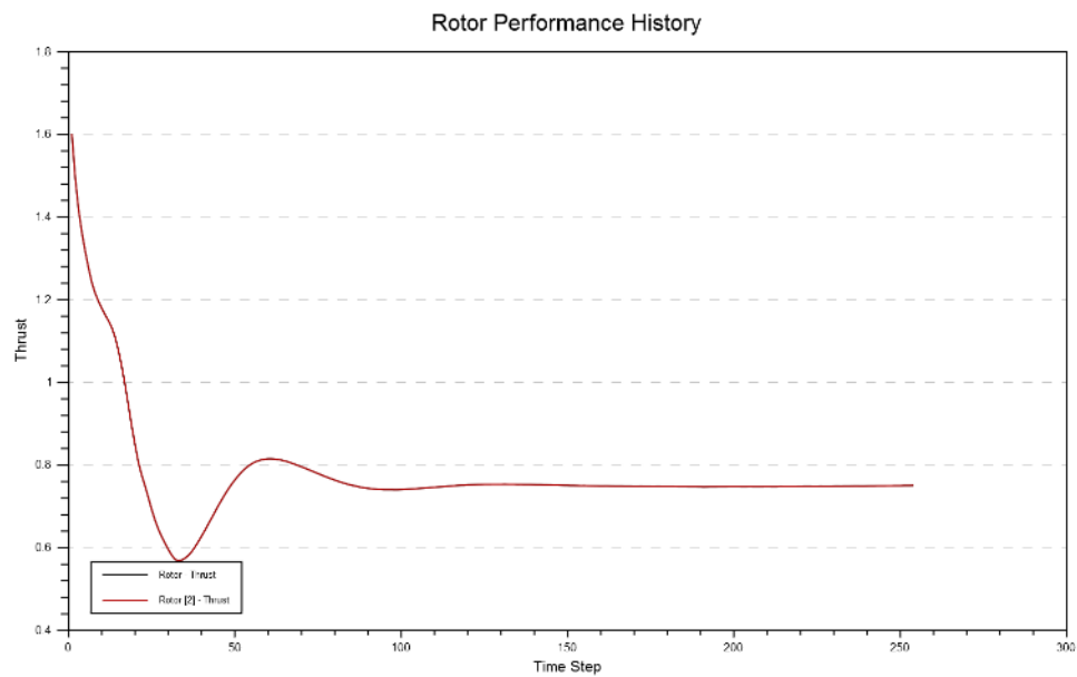
Figure C62. 14-mbar 2-Stack test 8 max velocity thrust.
