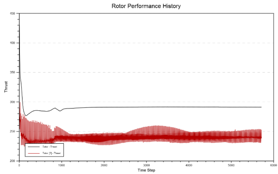
Figure C23. 1013-mbar 2-Stack test 2 isol thrust.
