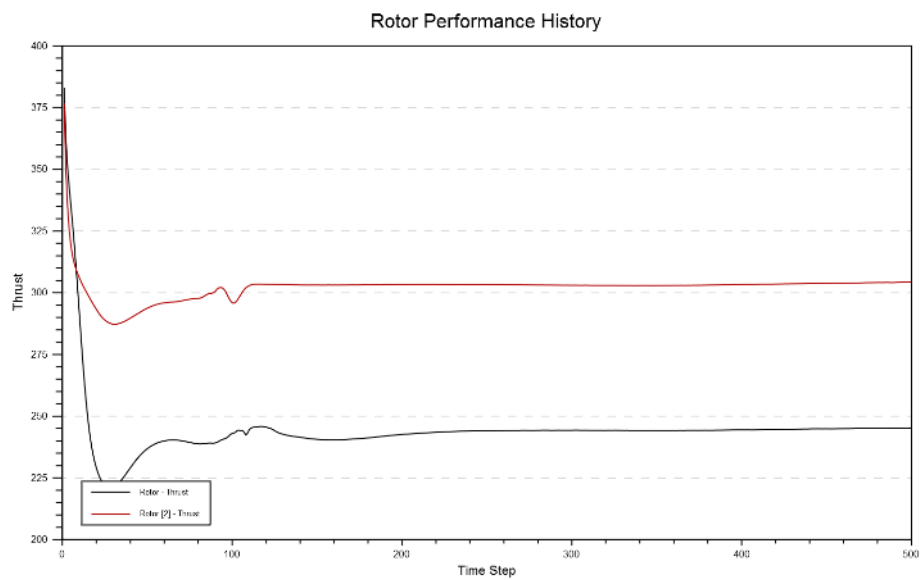
Figure C30. 1013-mbar 2-Stack test 5 isol thrust.
