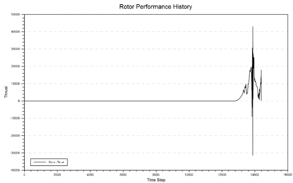
Figure C38. 14-mbar 1-Stack test 7 full thrust.
