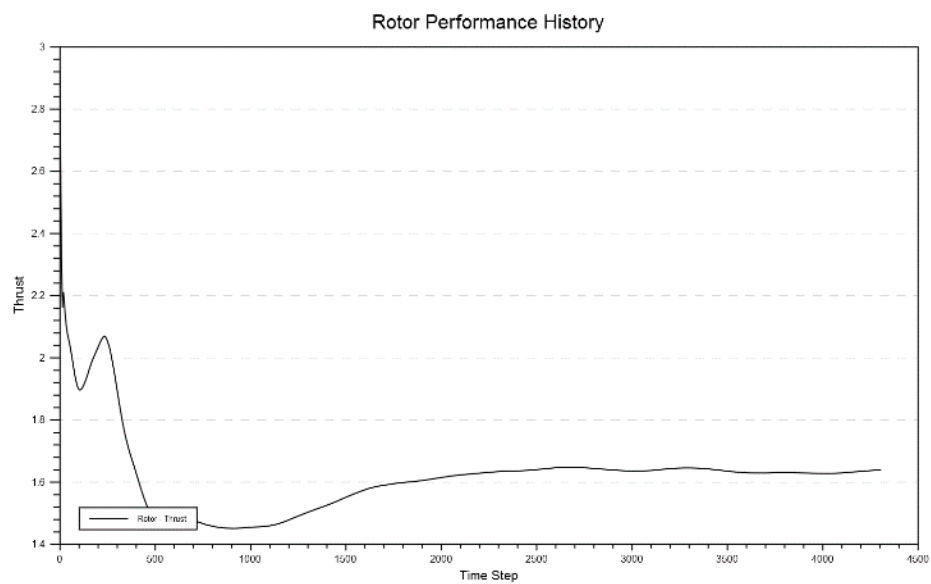
Figure C42. 14-mbar 1-Stack test 9 full thrust.
