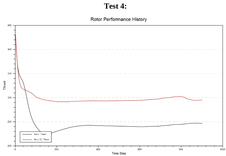
Figure C28. 1013-mbar 2-Stack test 4 isol thrust.
