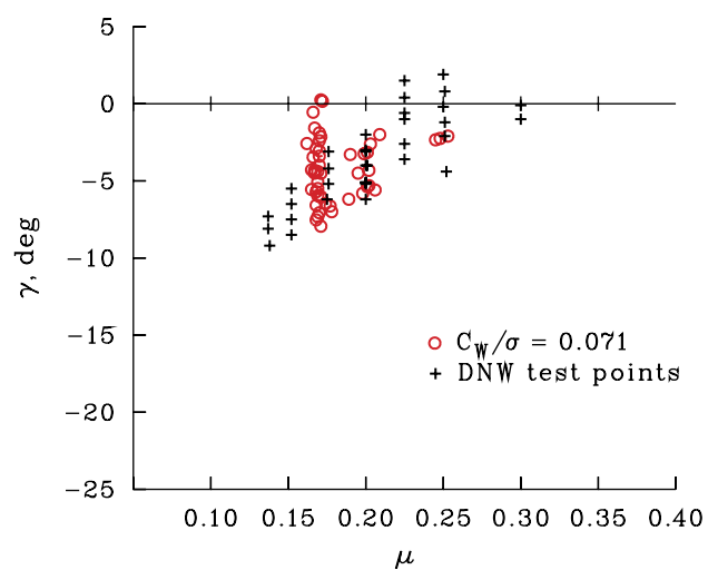
Figure 94. – IRAP flight path angles as a function of advance ratio compared with flight path angles from testing of a model-scale rotor in the DNW (Ref. 35).
