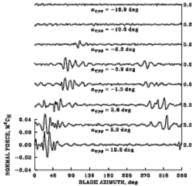
Figure 84. – Filtered time histories of normal force at 0.865R at an advance ratio of 0.2 shown as a function of tip-path-plane angle; 17–120 harmonics.
