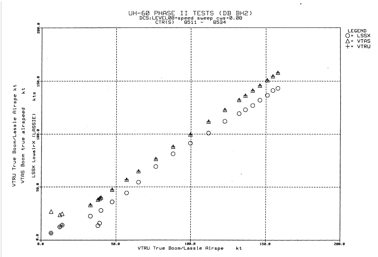
Figure 10.— Comparison of airspeed measurements for Flight 85.
