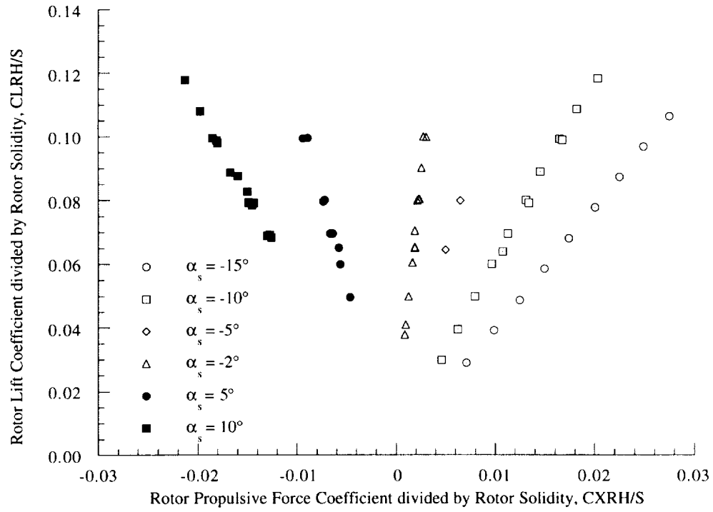
Figure 9(a). Rotor lift coefficient as a function of rotor propulsive force coefficient, 40 knots ( \mu = 0.10 ).
