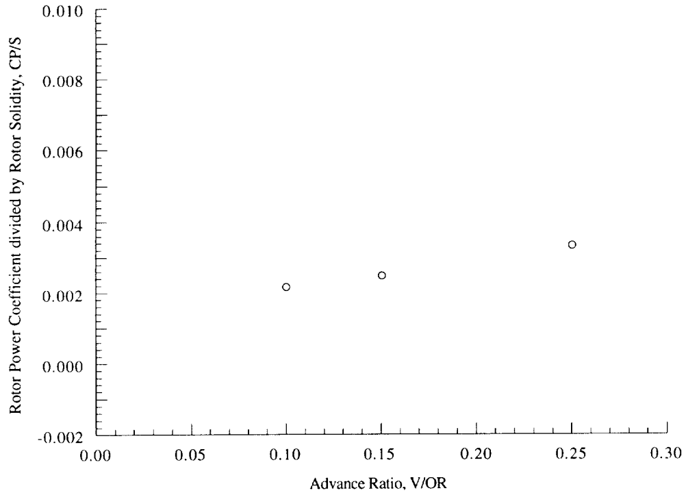
Figure 14(a). Rotor power coefficient as a function of advance ratio, \alpha_S = -15 deg, C_T/\sigma = 0.030 .
