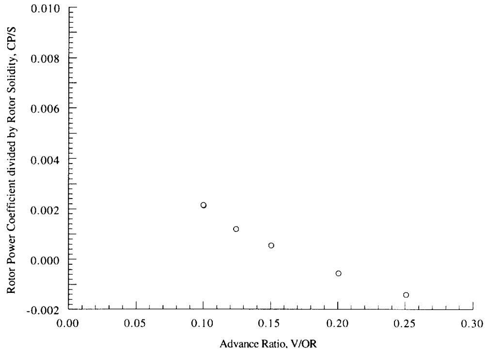
Figure 20(c). Rotor power coefficient as a function of advance ratio, \alpha_S = 10 deg, CT/\sigma = 0.090 .
