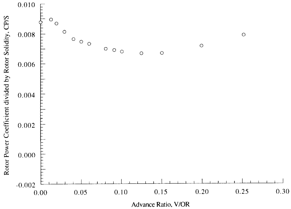
Figure 15(i). Rotor power coefficient as a function of advance ratio, \alpha_S = -10 deg, C_T/\sigma = 0.100 .
