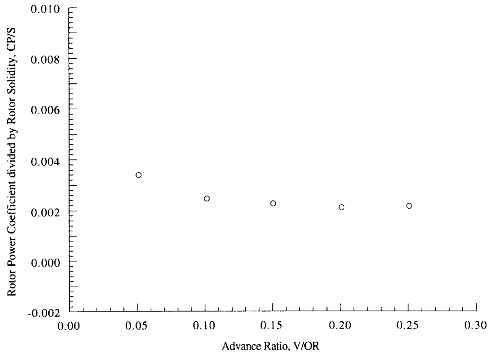
Figure 17(c). Rotor power coefficient as a function of advance ratio, \alpha_S = -2 deg, C_T/\sigma = 0.060 .
