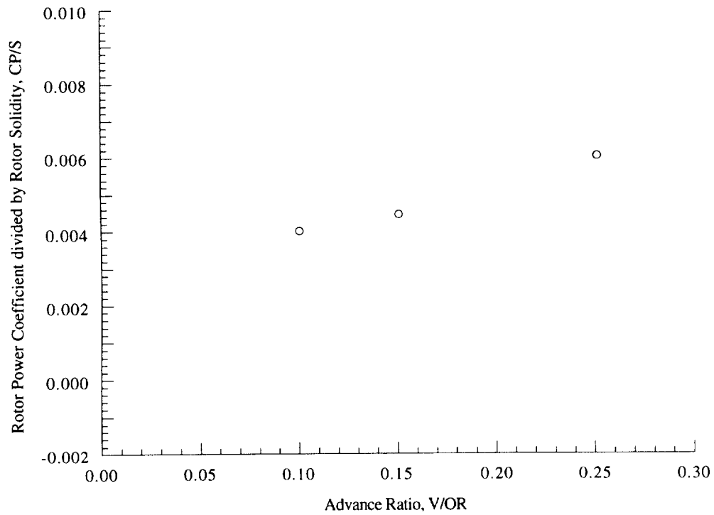
Figure 14(d). Rotor power coefficient as a function of advance ratio, \alpha_S = -15 deg, C_T/\sigma = 0.060 .
