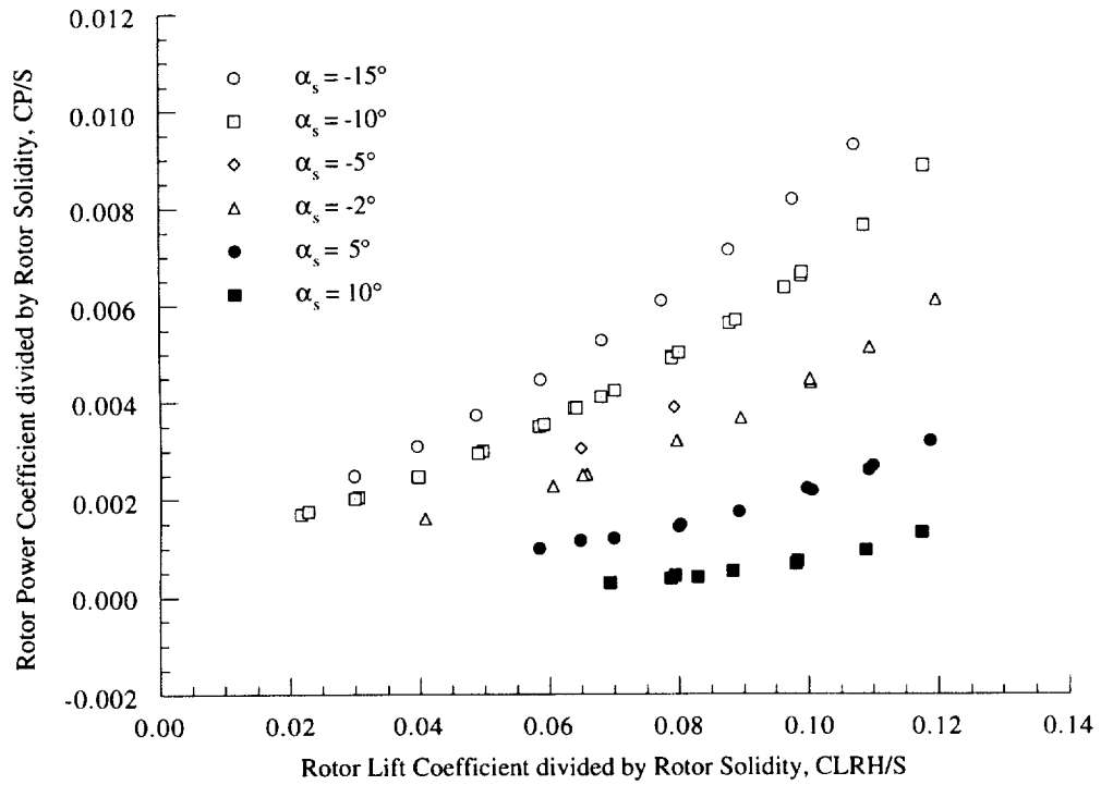
Figure 11(b). Rotor power coefficient as a function of rotor lift coefficient, 60 knots ( \mu = 0.15 ).
