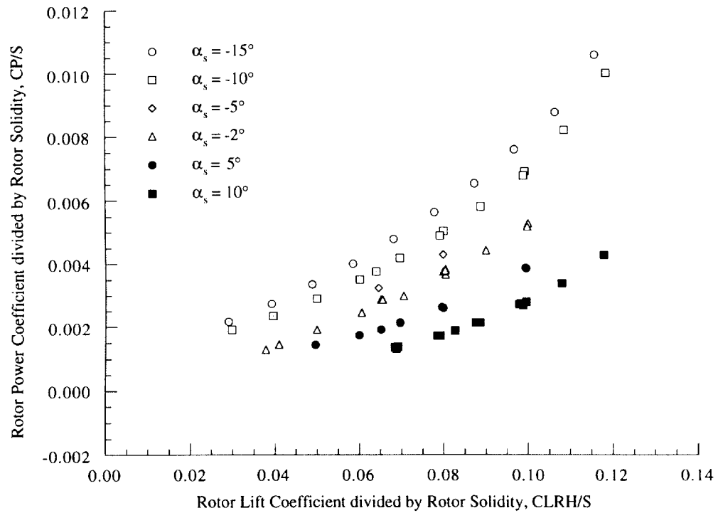
Figure 9(b). Rotor power coefficient as a function of rotor lift coefficient, 40 knots ( \mu = 0.10 ).
