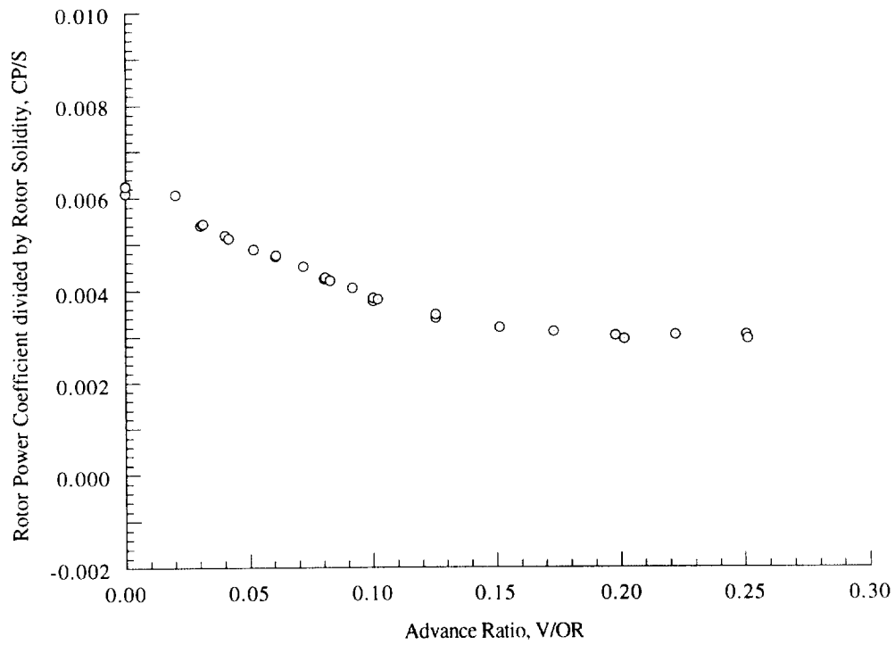
Figure 17(f). Rotor power coefficient as a function of advance ratio, \alpha_S = -2 deg, C_T/\sigma = 0.080 .
