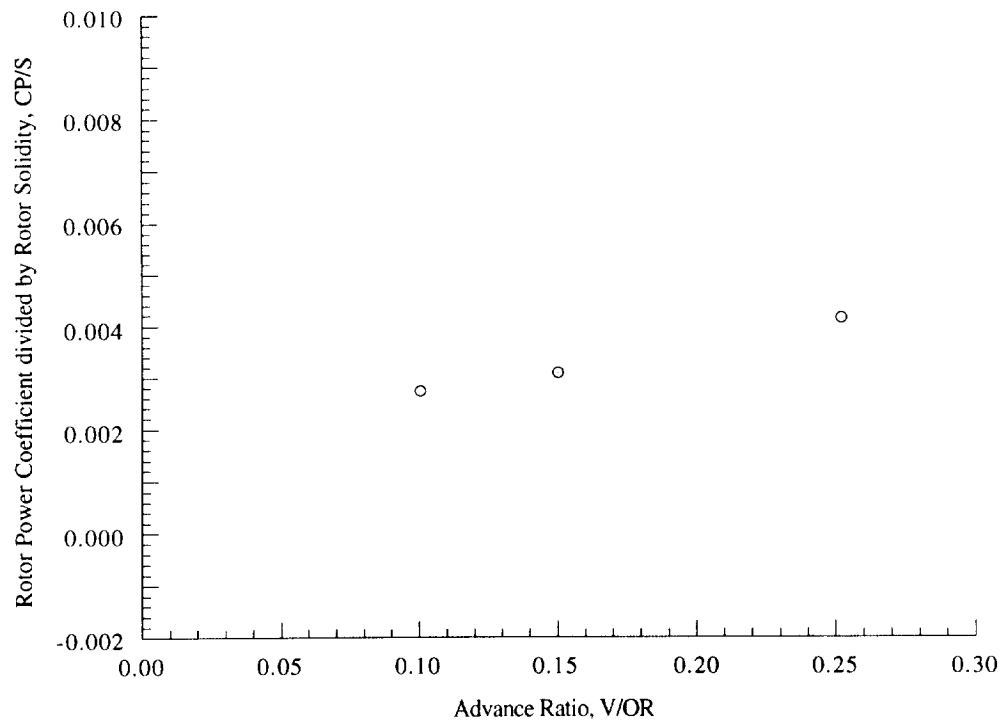
Figure 14(b). Rotor power coefficient as a function of advance ratio, \alpha_S = -15 deg, C_T/\sigma = 0.040 .
