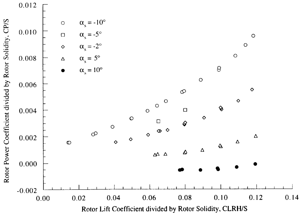
Figure 12(b). Rotor power coefficient as a function of rotor lift coefficient, 80 knots ( \mu = 0.20 ).
