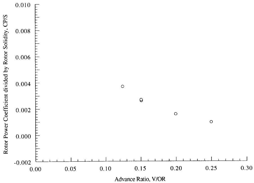
Figure 19(g). Rotor power coefficient as a function of advance ratio, \alpha_S = 5 deg, C_T/\sigma = 0.110 .
