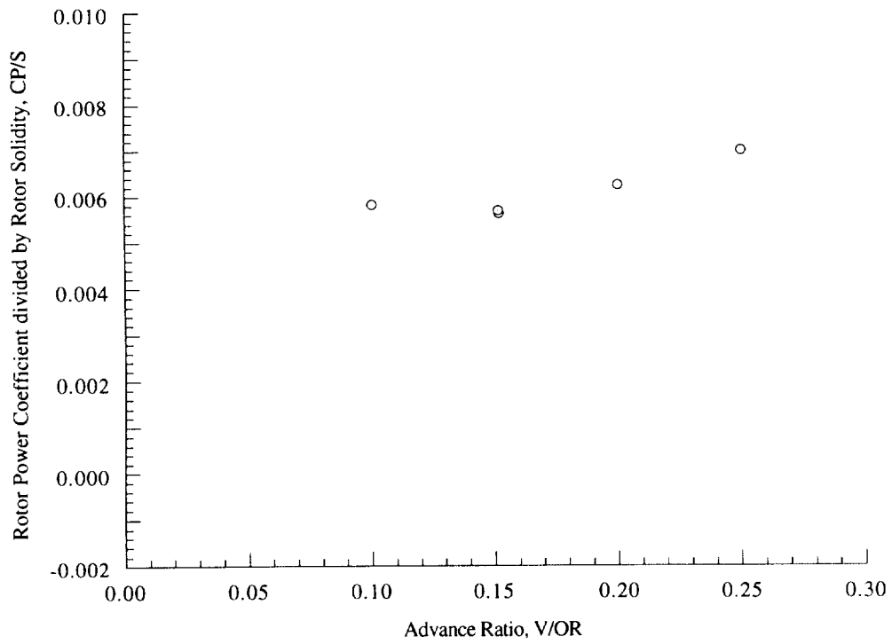
Figure 15(h). Rotor power coefficient as a function of advance ratio, \alpha_S = -10 deg, C_T/\sigma = 0.090 .
