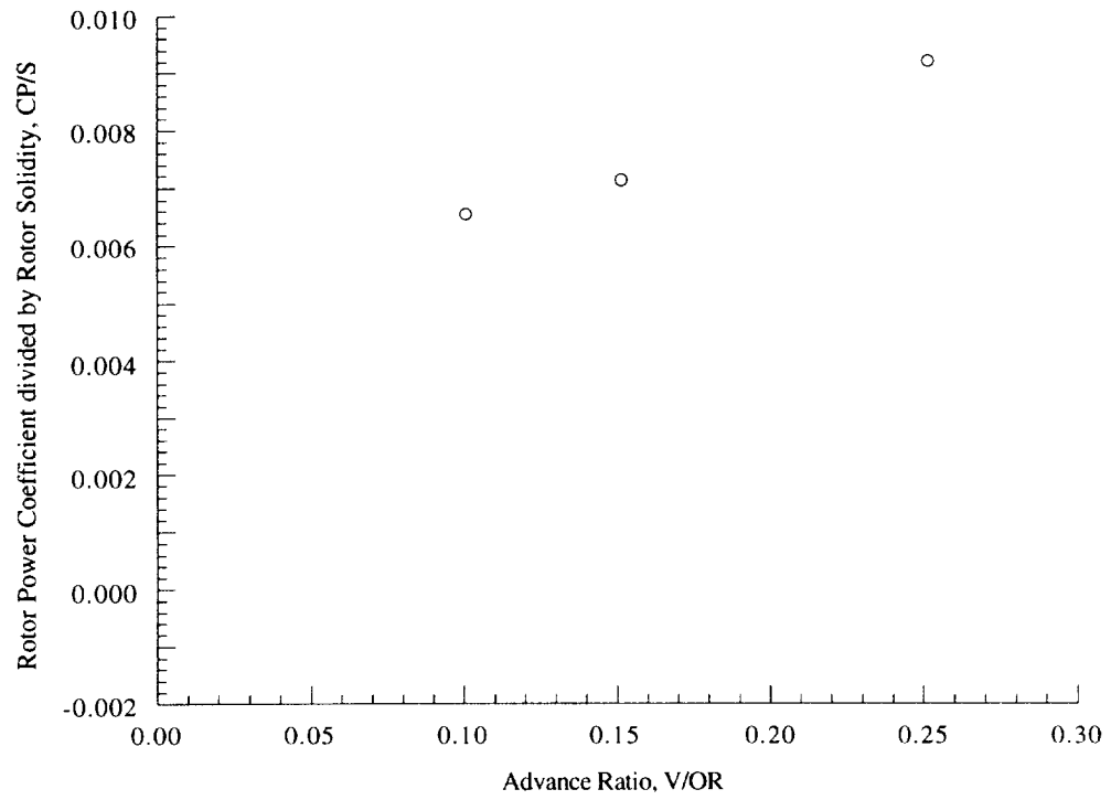
Figure 14(g). Rotor power coefficient as a function of advance ratio, \alpha_S = -15 deg, C_T/\sigma = 0.090 .
