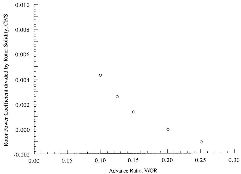
Figure 20(f). Rotor power coefficient as a function of advance ratio, \alpha_S = 10 \text{ deg} , C_T/\sigma = 0.120 .
