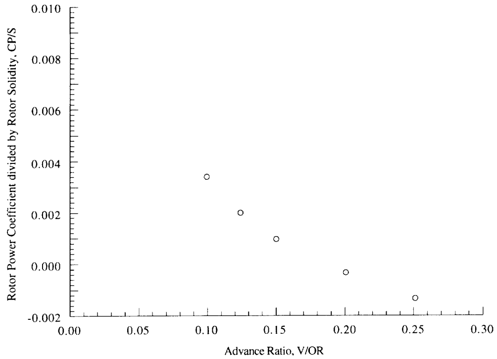
Figure 20(e). Rotor power coefficient as a function of advance ratio, \alpha_S = 10 \text{ deg} , C_T/\sigma = 0.110 .
