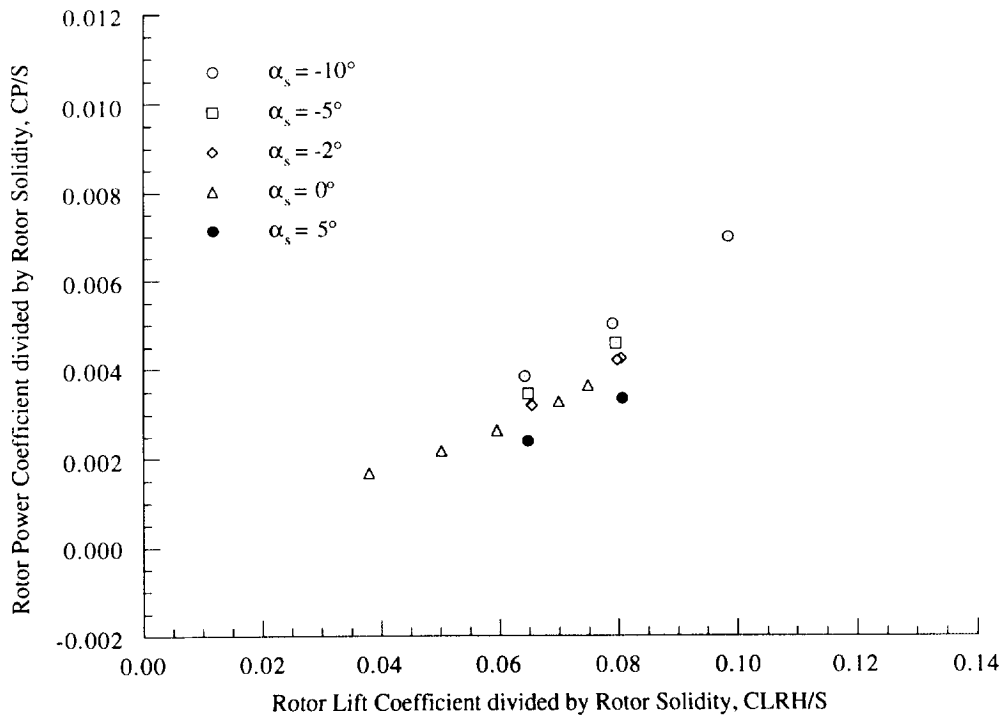
Figure 8(b). Rotor power coefficient as a function of rotor lift coefficient, 32 knots ( \mu = 0.08 ).
