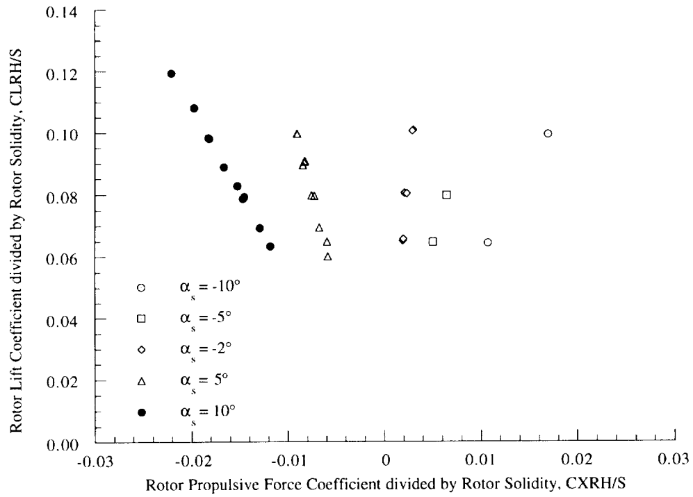
Figure 10(a). Rotor lift coefficient as a function of rotor propulsive force coefficient, 50 knots ( \mu = 0.125 ).
