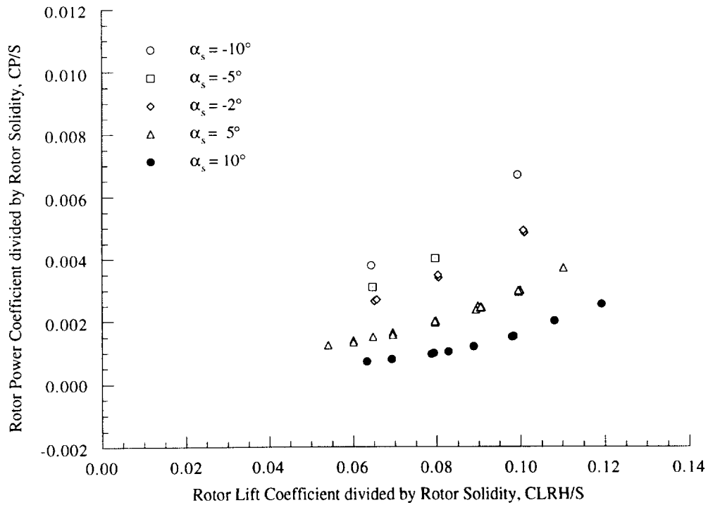
Figure 10(b). Rotor power coefficient as a function of rotor lift coefficient, 50 knots ( \mu = 0.125 ).
