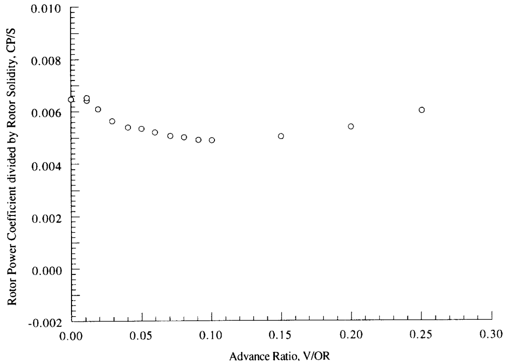
Figure 15(g). Rotor power coefficient as a function of advance ratio, \alpha_S = -10 deg, C_T/\sigma = 0.080 .
