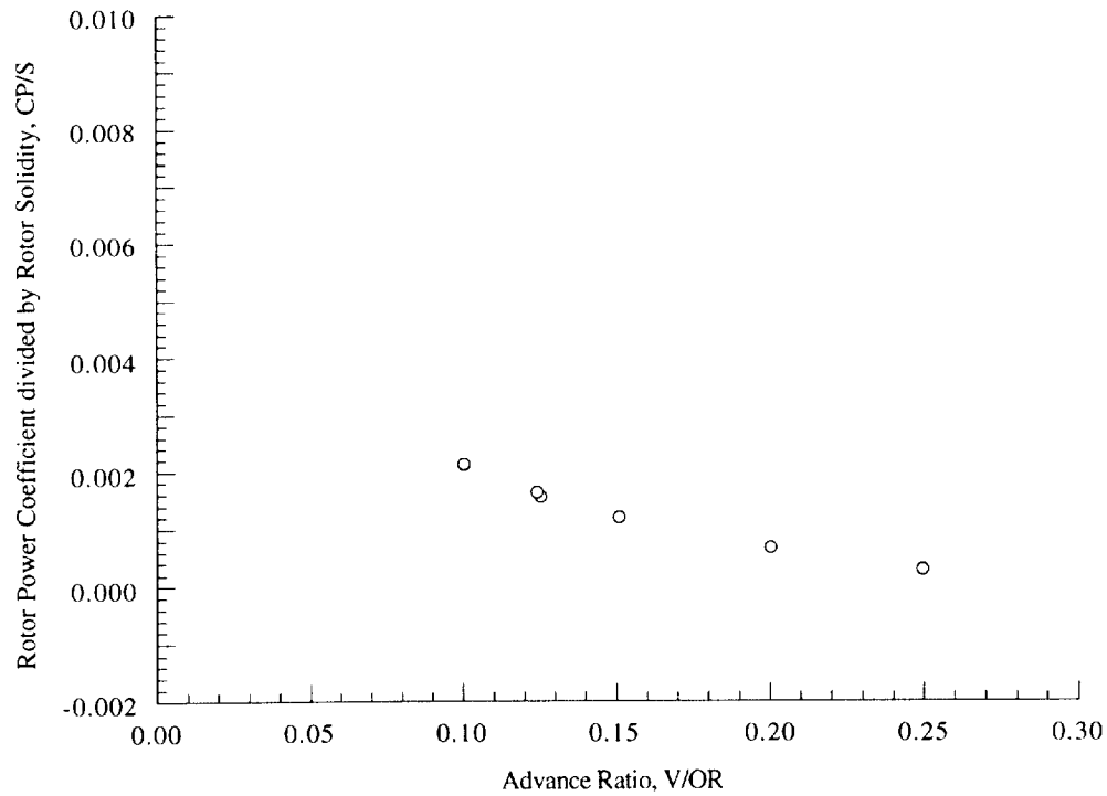
Figure 19(c). Rotor power coefficient as a function of advance ratio, \alpha_S = 5 deg, C_T/\sigma = 0.070 .
