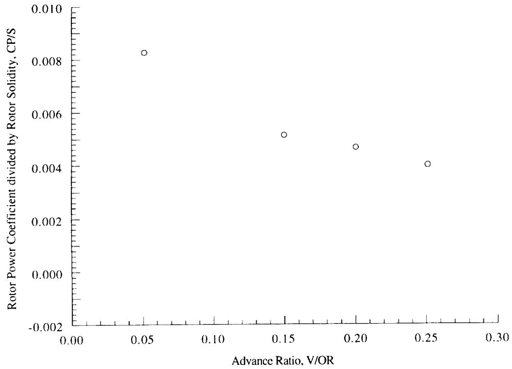
Figure 17(i). Rotor power coefficient as a function of advance ratio, \alpha_S = -2 deg, C_T/\sigma = 0.110 .
