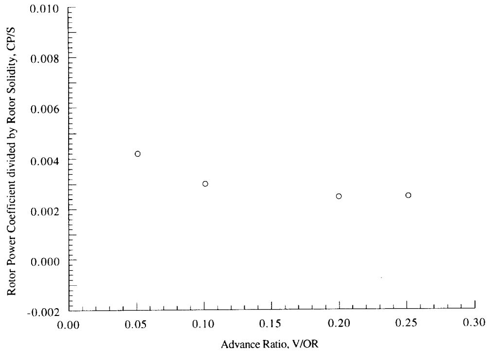
Figure 17(e). Rotor power coefficient as a function of advance ratio, \alpha_S = -2 deg, C_T/\sigma = 0.070 .
