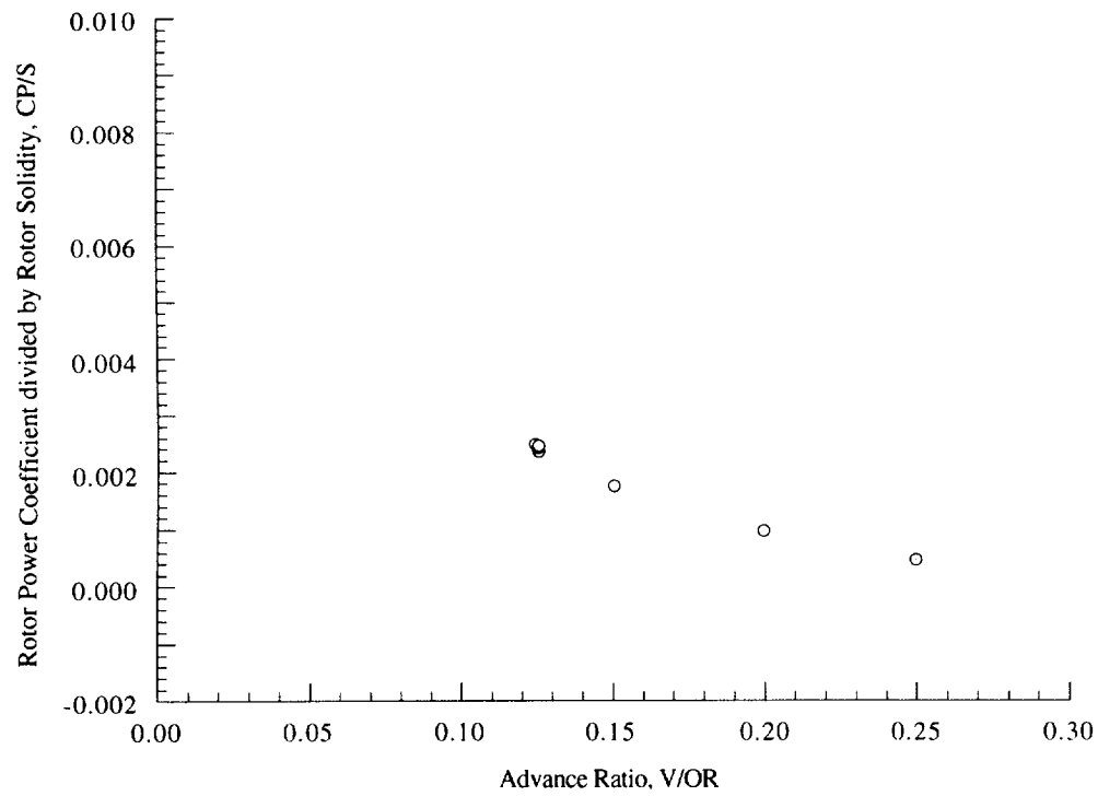
Figure 19(e). Rotor power coefficient as a function of advance ratio, \alpha_S = 5 \text{ deg} , C_T/\sigma = 0.090 .
