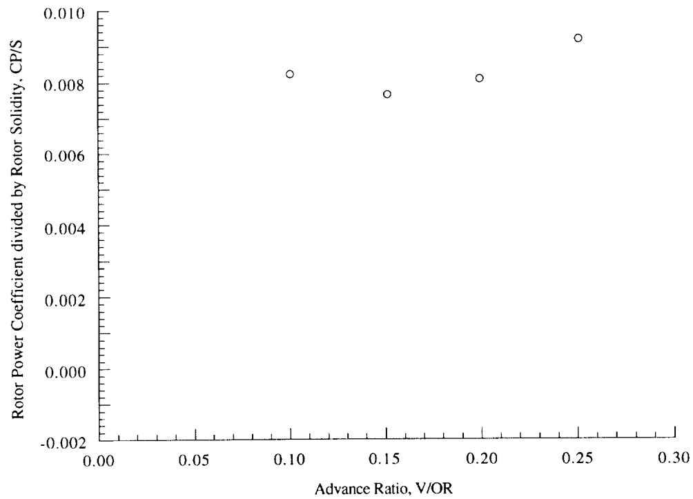
Figure 15(j). Rotor power coefficient as a function of advance ratio, \alpha_S = -10 deg, C_T/\sigma = 0.110 .
