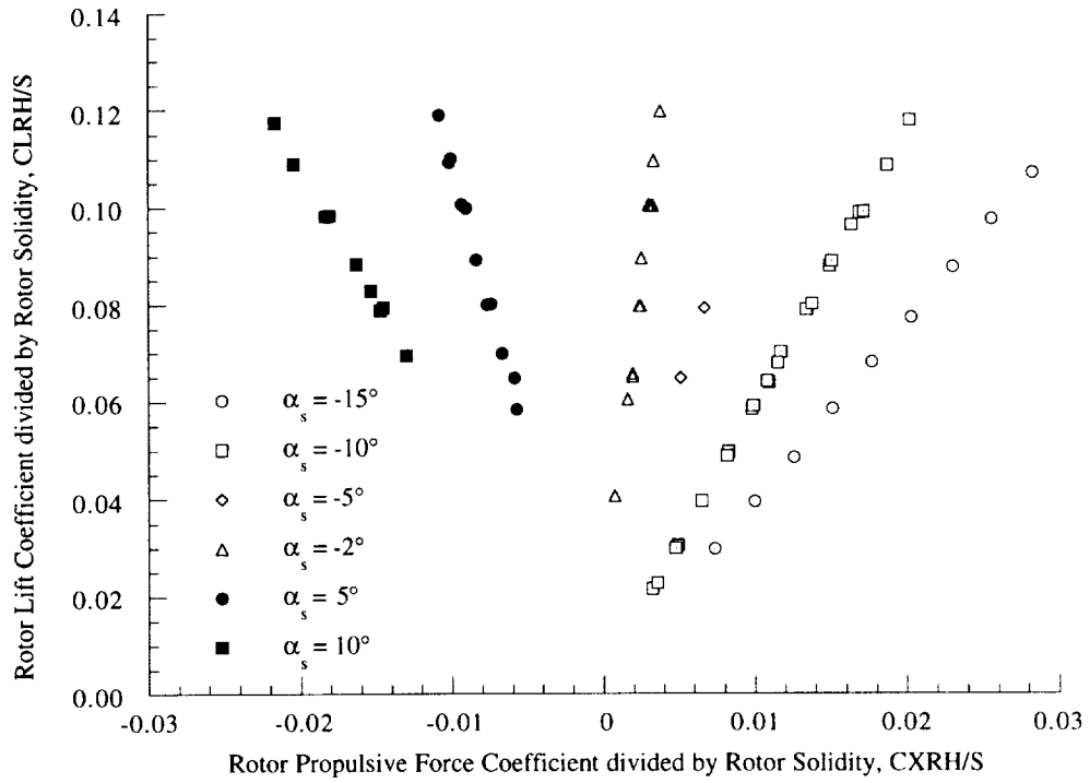
Figure 11(a). Rotor lift coefficient as a function of rotor propulsive force coefficient, 60 knots ( \mu = 0.15 ).
