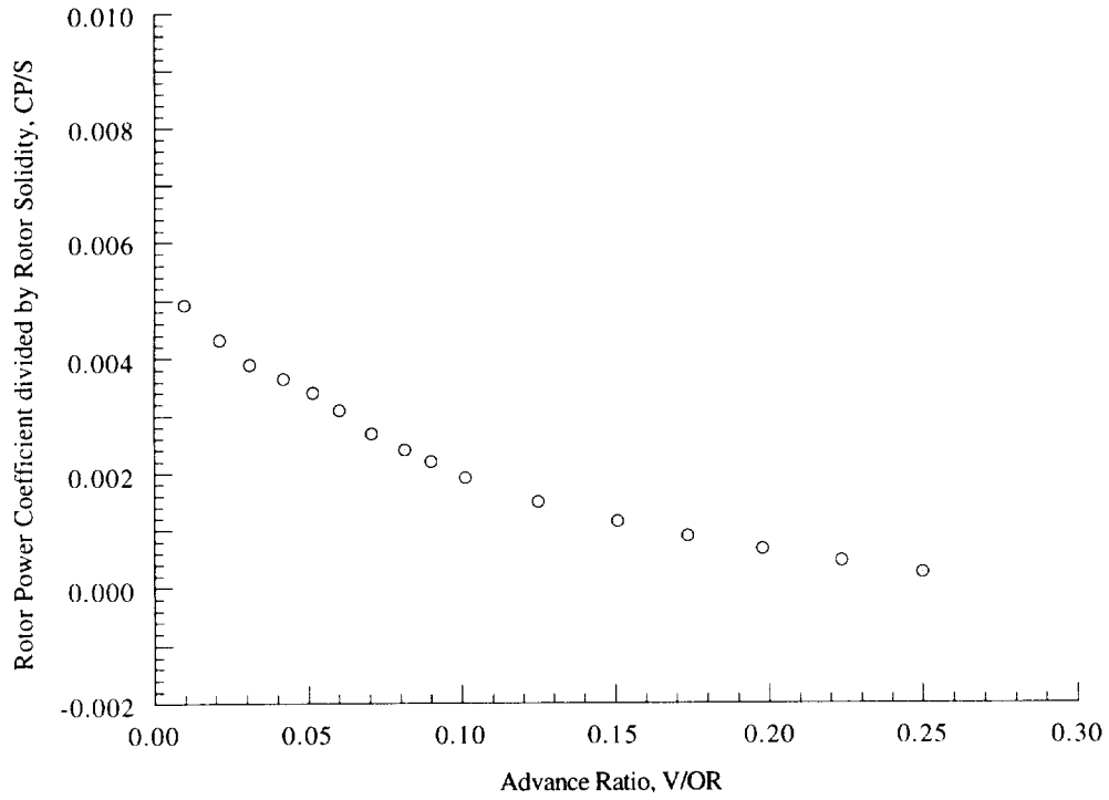
Figure 19(b). Rotor power coefficient as a function of advance ratio, \alpha_S = 5 deg, C_T/\sigma = 0.065 .
