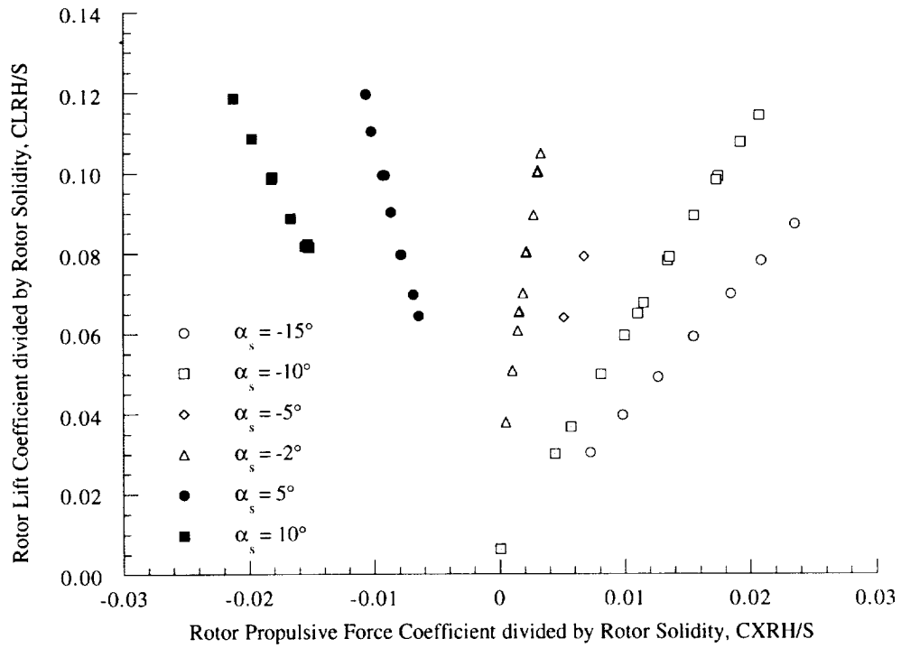
Figure 13(a). Rotor lift coefficient as a function of rotor propulsive force coefficient, 100 knots ( \mu = 0.25 ).
