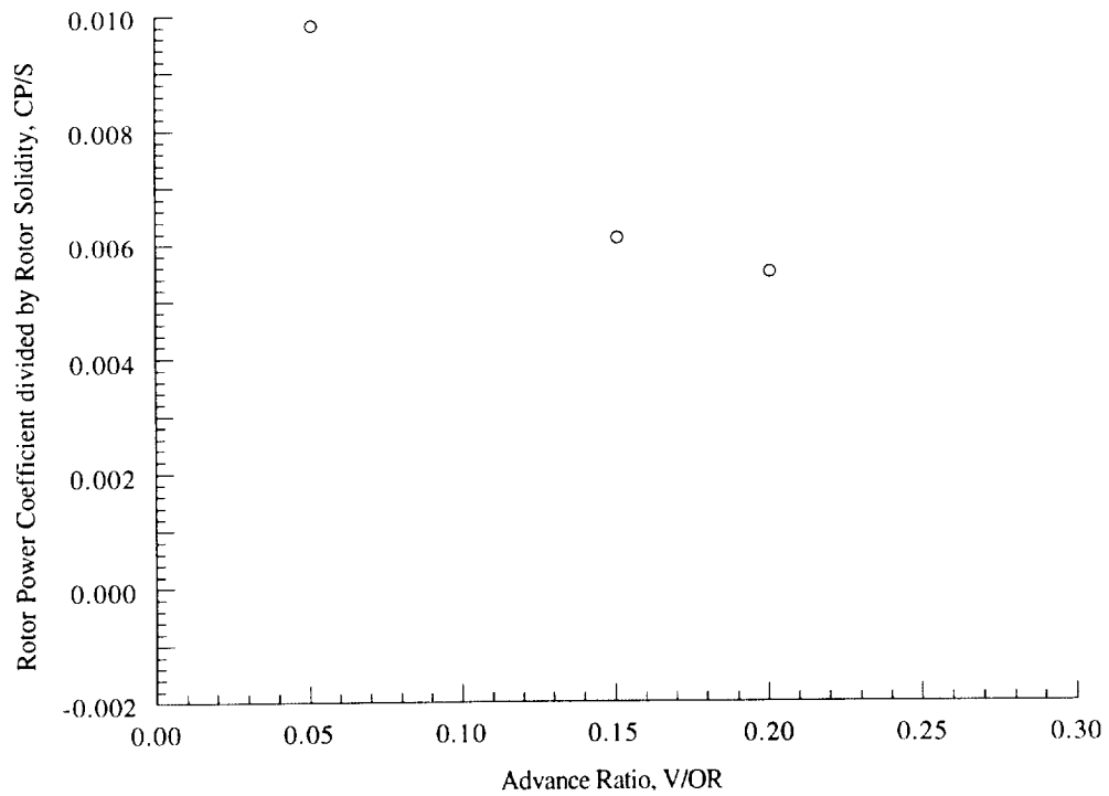
Figure 17(j). Rotor power coefficient as a function of advance ratio, \alpha_S = -2 deg, C_T/\sigma = 0.120 .
