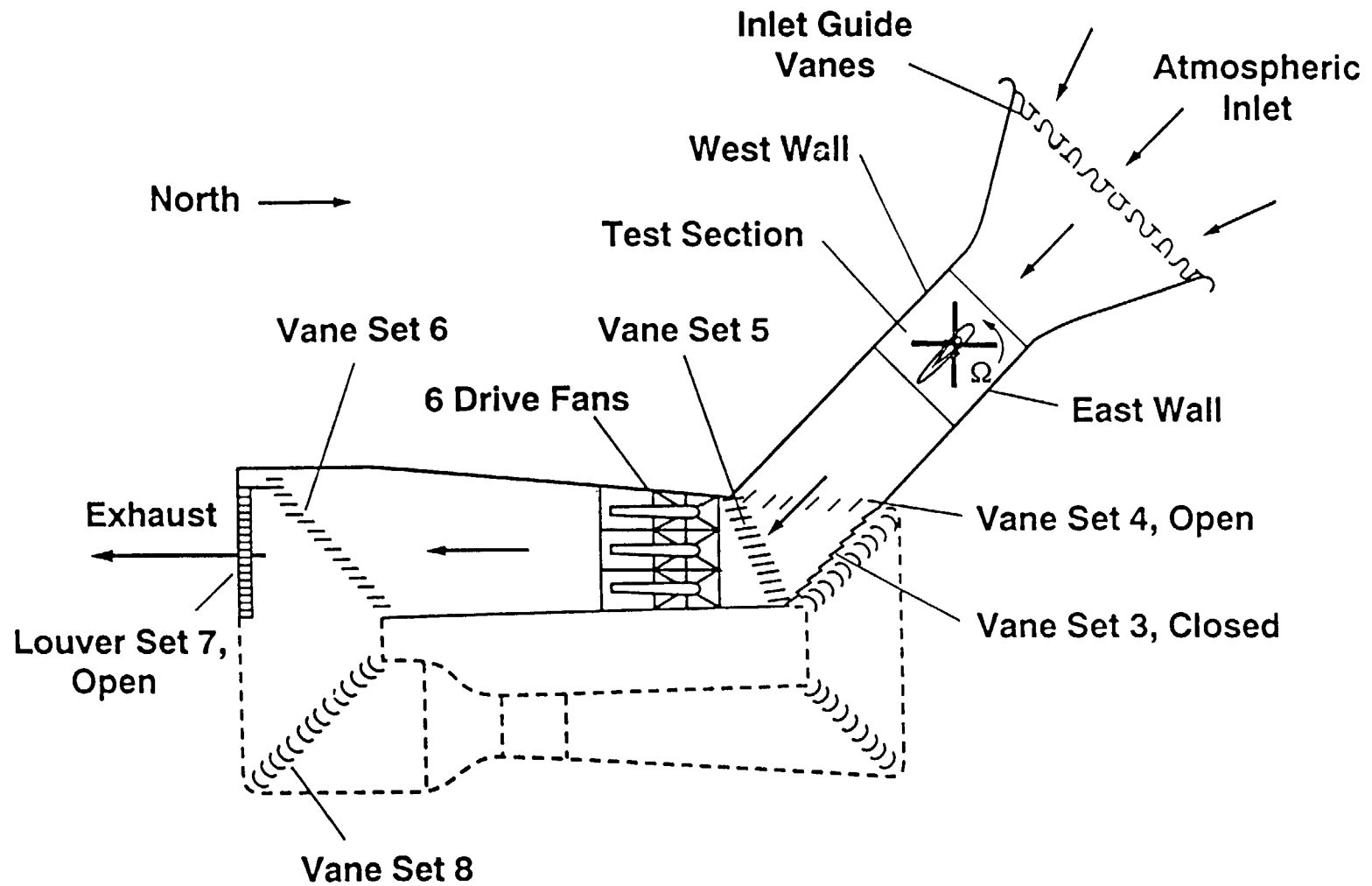
Figure 1. 80- by 120-Foot Wind Tunnel Circuit.
