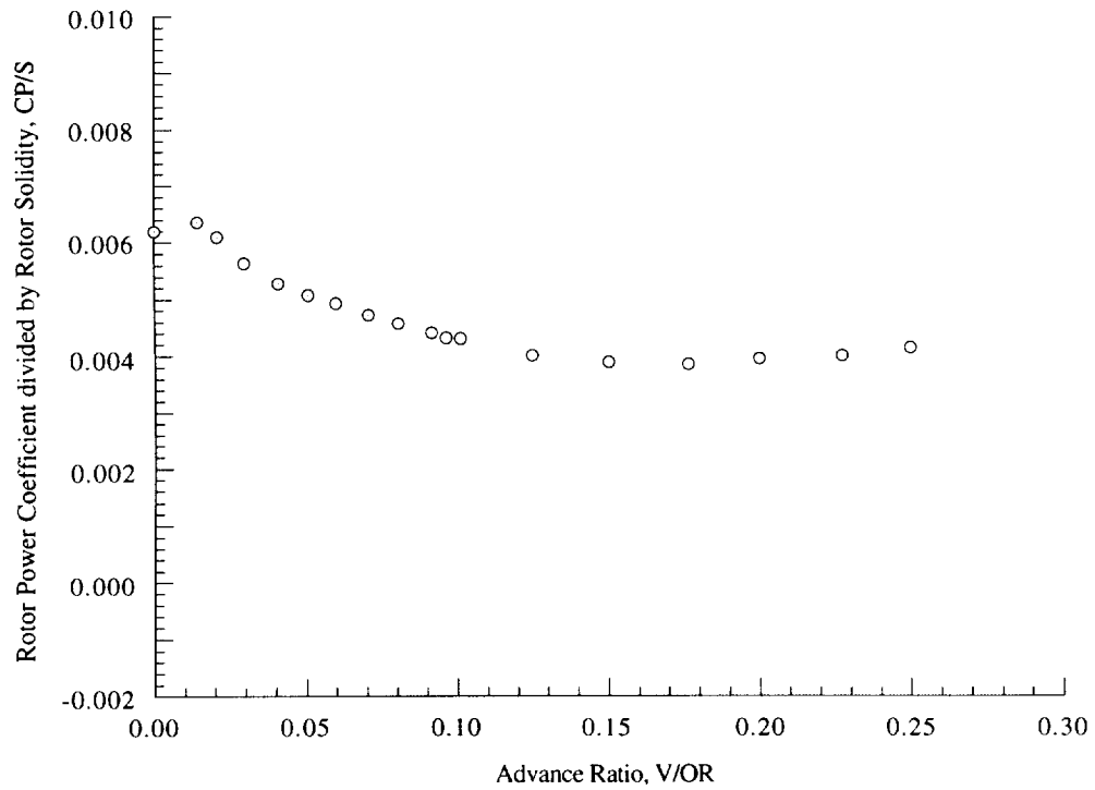
Figure 16(b). Rotor power coefficient as a function of advance ratio, \alpha_S = -5 deg, C_T/\sigma = 0.080 .
