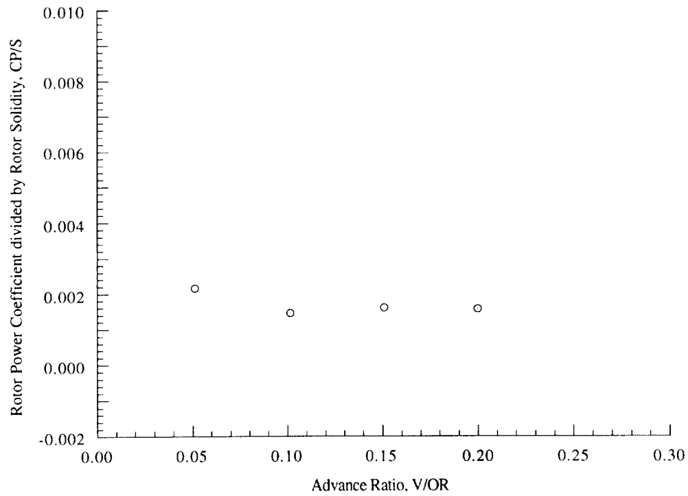
Figure 17(b). Rotor power coefficient as a function of advance ratio, \alpha_S = -2 deg, C_T/\sigma = 0.050 .
