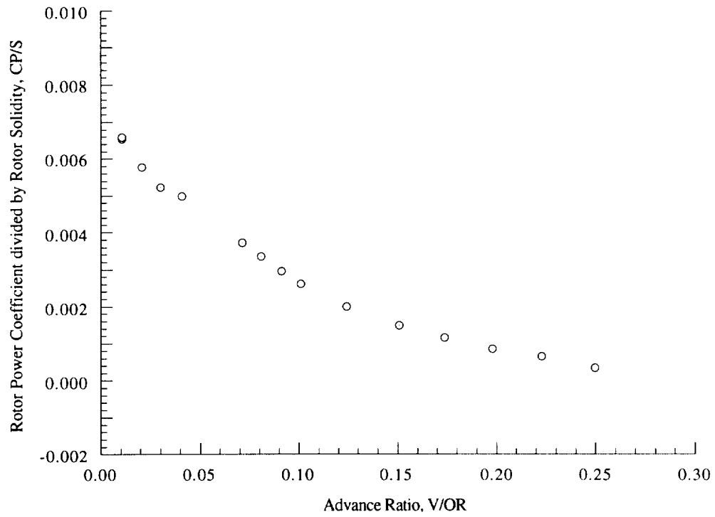
Figure 19(d). Rotor power coefficient as a function of advance ratio, \alpha_S = 5 \text{ deg} , C_T/\sigma = 0.080 .
