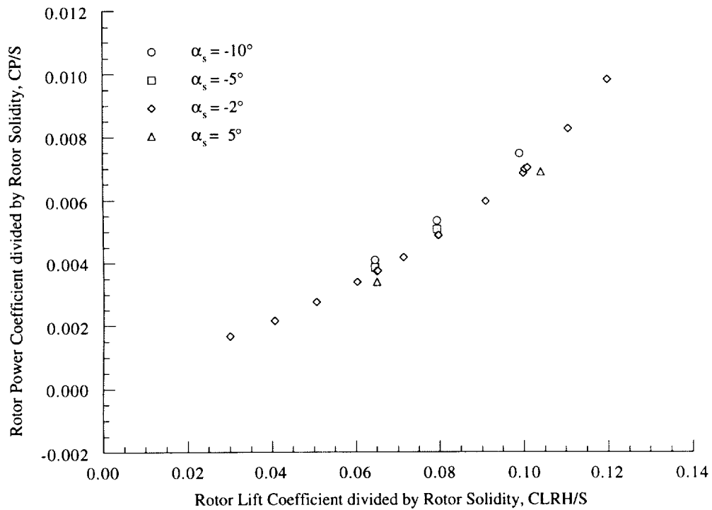
Figure 7(b). Rotor power coefficient as a function of rotor lift coefficient, 20 knots ( \mu = 0.05 ).
