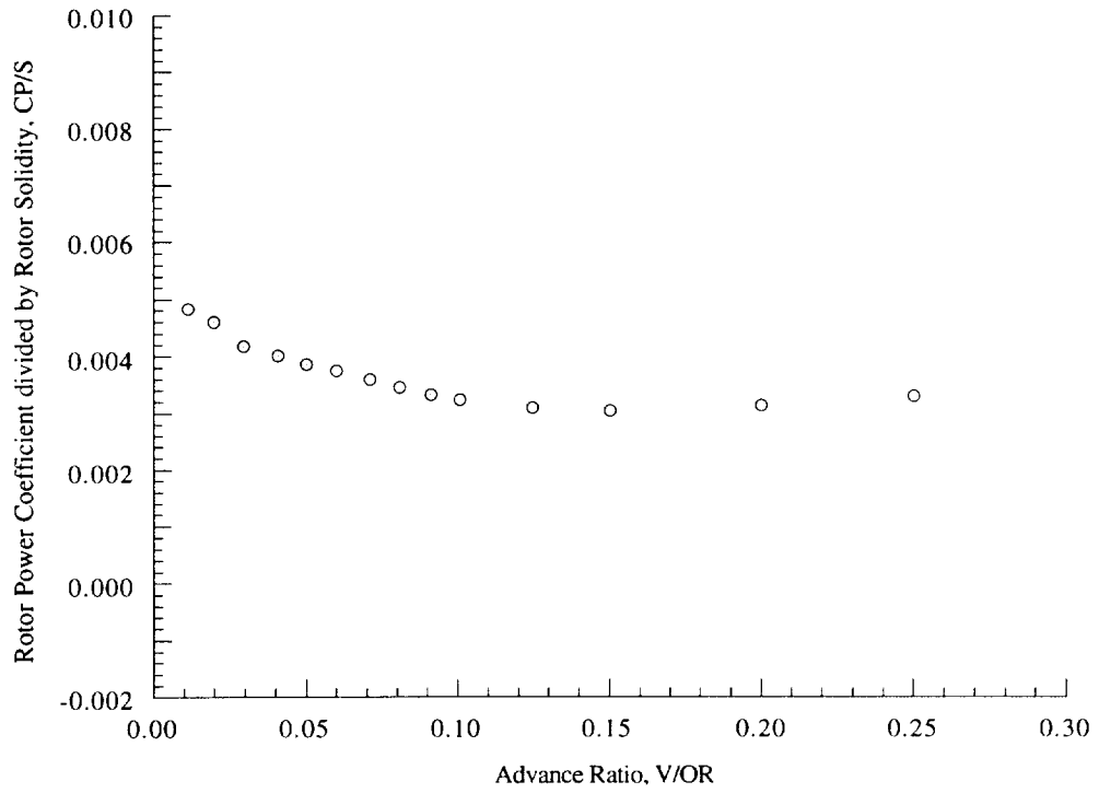
Figure 16(a). Rotor power coefficient as a function of advance ratio, \alpha_S = -5 deg, C_T/\sigma = 0.065 .
