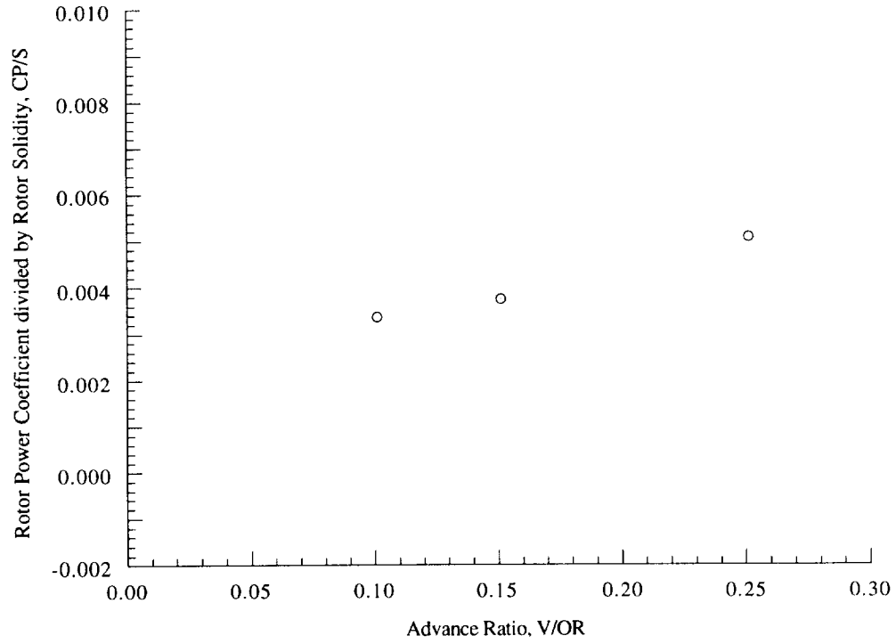
Figure 14(c). Rotor power coefficient as a function of advance ratio, \alpha_S = -15 deg, C_T/\sigma = 0.050 .
