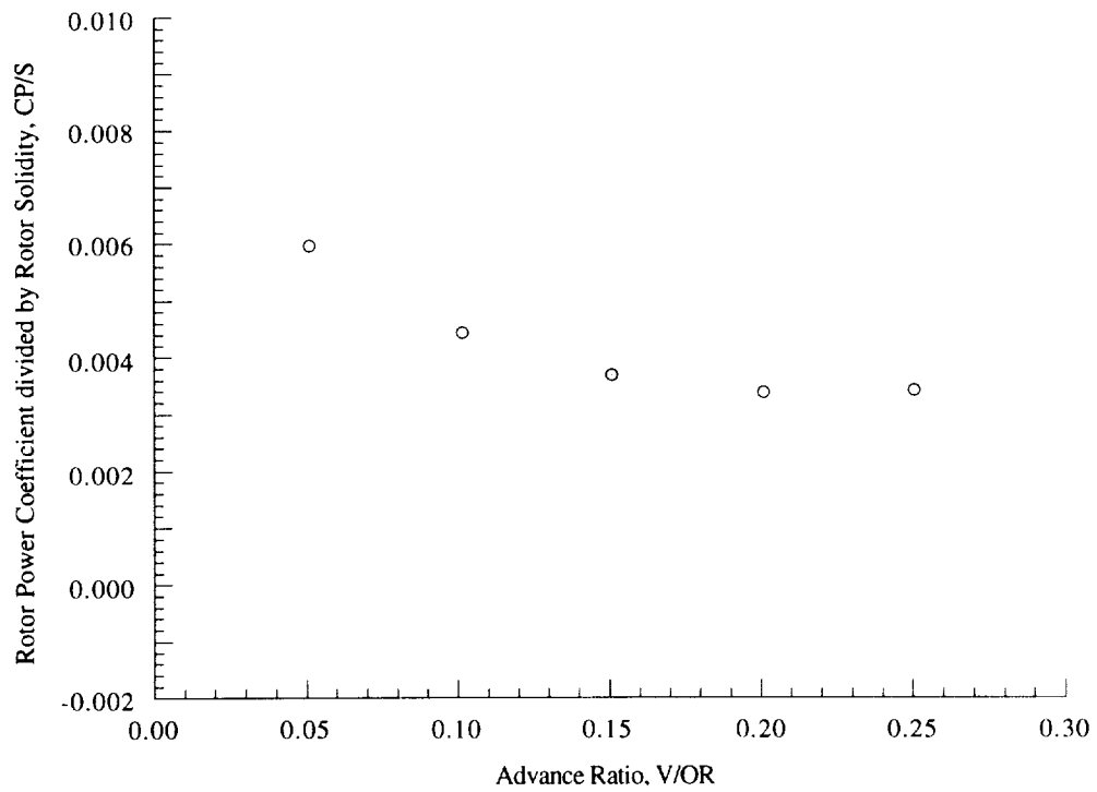
Figure 17(g). Rotor power coefficient as a function of advance ratio, \alpha_S = -2 deg, C_T/\sigma = 0.090 .
