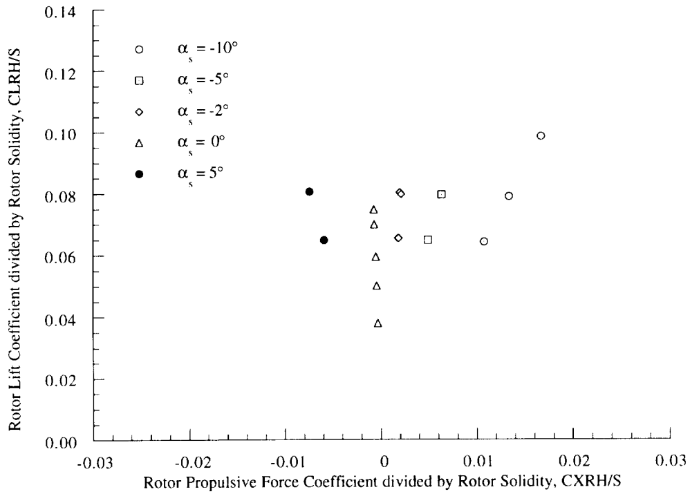
Figure 8(a). Rotor lift coefficient as a function of rotor propulsive force coefficient, 32 knots ( \mu = 0.08 ).
