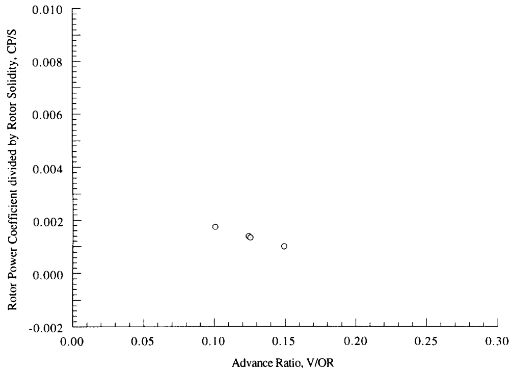
Figure 19(a). Rotor power coefficient as a function of advance ratio, \alpha_S = 5 deg, C_T/\sigma = 0.060 .
