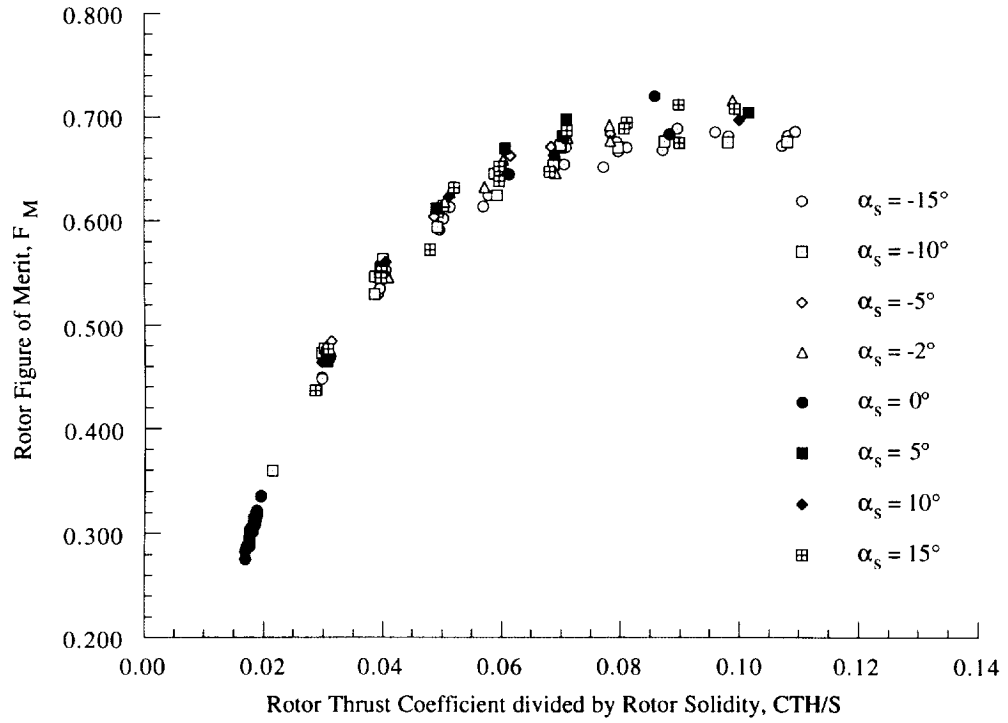
Figure 5(b). Rotor figure of merit as a function of rotor thrust coefficient, YAW = 0 deg, hover.
