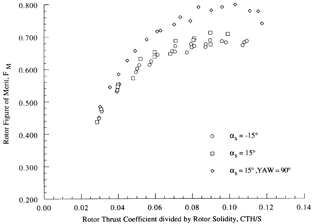
Figure 6(b). Rotor figure of merit as a function of rotor thrust coefficient at two different yaw positions, YAW = 0 deg, 90 deg, hover.
