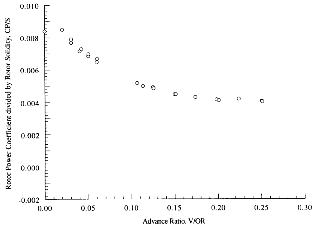
Figure 17(h). Rotor power coefficient as a function of advance ratio, \alpha_S = -2 deg, C_T/\sigma = 0.100 .
