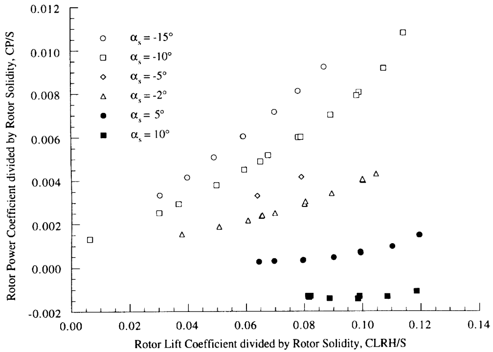
Figure 13(b). Rotor power coefficient as a function of rotor lift coefficient, 100 knots ( \mu = 0.25 ).
