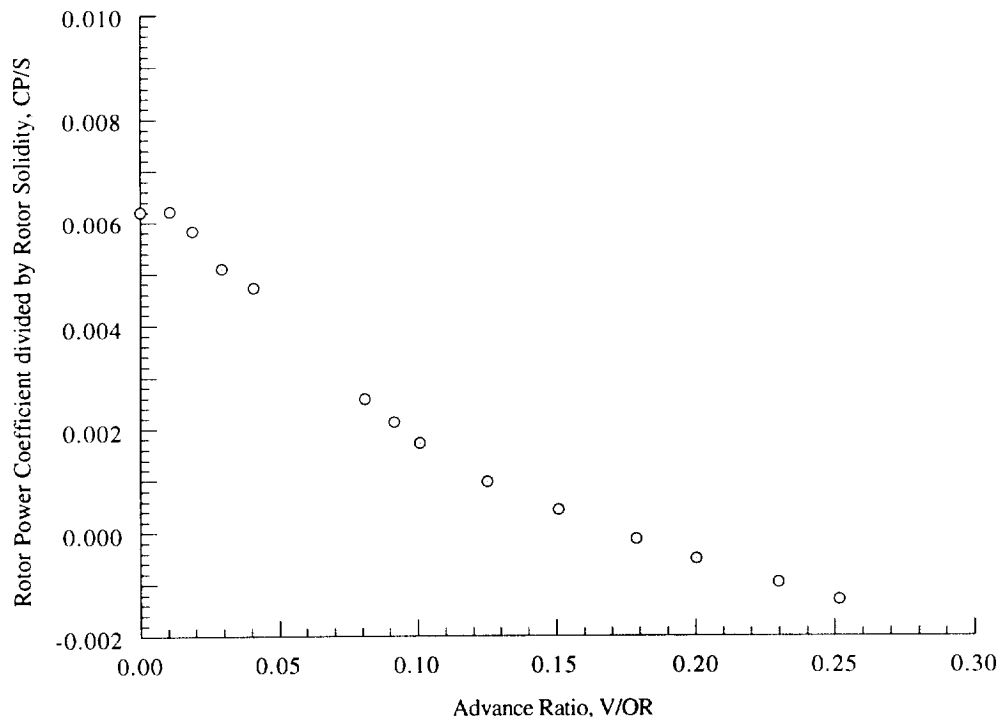
Figure 20(b). Rotor power coefficient as a function of advance ratio, \alpha_S = 10 deg, C_T/\sigma = 0.080 .
