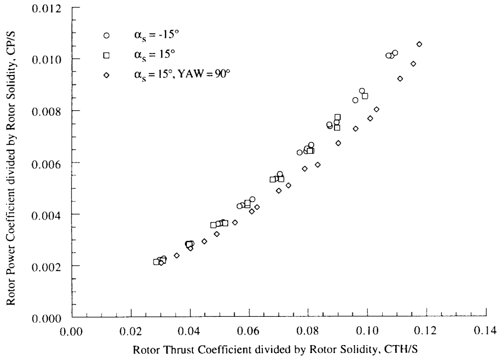
Figure 6(a). Rotor power coefficient as a function of rotor thrust coefficient at two different yaw positions, YAW = 0 deg, 90 deg, hover.
