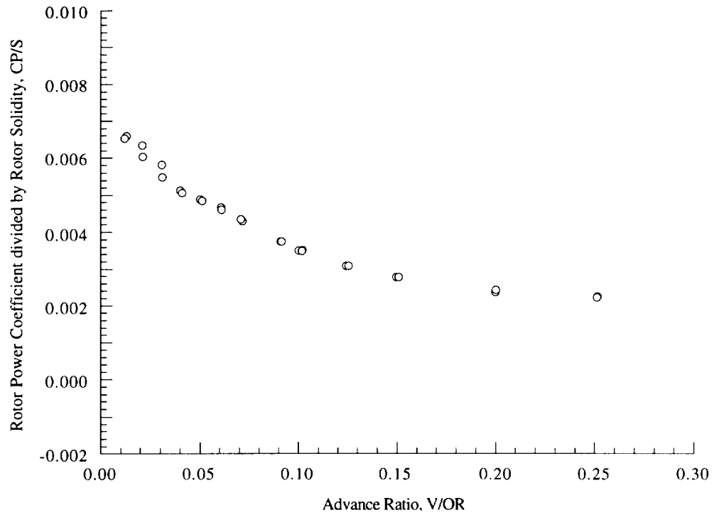
Figure 18(a). Rotor power coefficient as a function of advance ratio, \alpha_S = 0 deg, C_T/\sigma = 0.080 .
