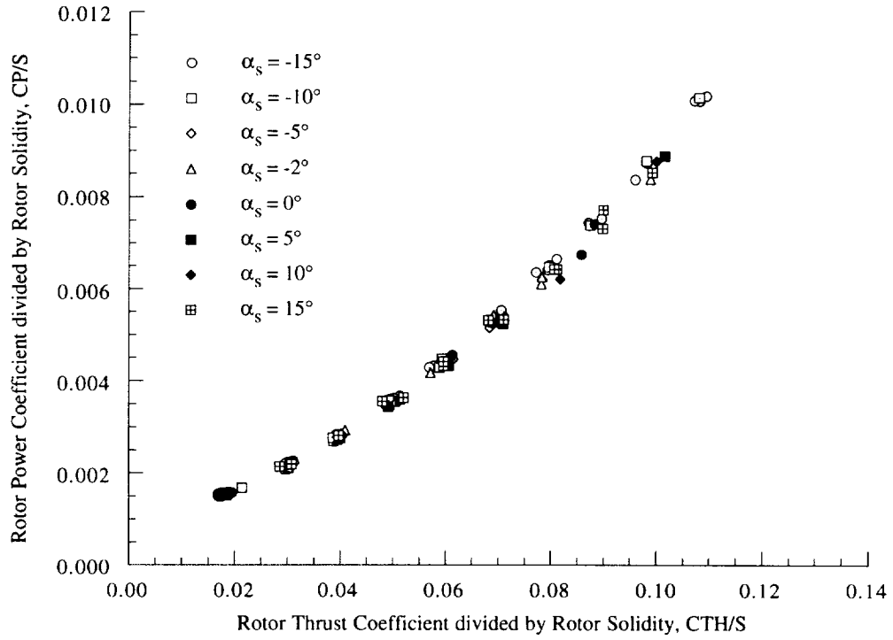
Figure 5(a). Rotor power coefficient as a function of rotor thrust coefficient, YAW = 0 deg, hover.
