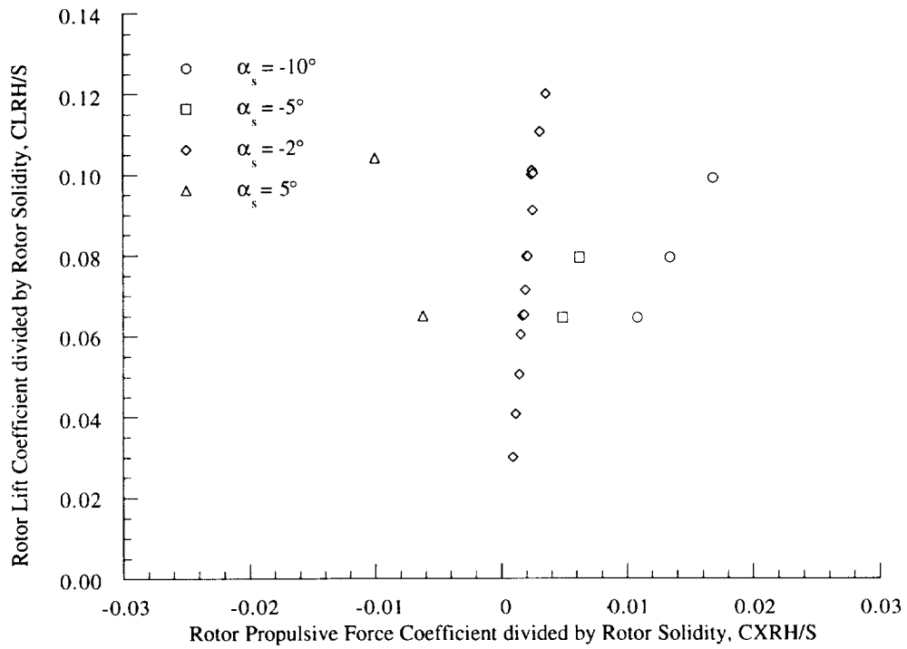
Figure 7(a). Rotor lift coefficient as a function of rotor propulsive force coefficient, 20 knots ( \mu = 0.05 ).
