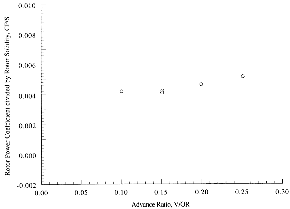
Figure 15(f). Rotor power coefficient as a function of advance ratio, \alpha_S = -10 deg, C_T/\sigma = 0.070 .
