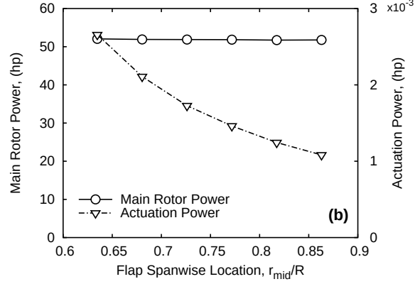
Figure 5: Effect of trailing-edge flap location on flap angles, main rotor power, and and actuation requirements at forward speed of 60 knots ( \mu = 0.16 )
