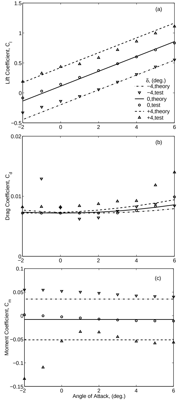
Figure 1: Measured and predicted aerodynamic coefficients of 2D HH-06 airfoil with 0.35 plain trailing-edge flap (10%c overhang, Mach = 0.45); (a) lift (b) drag and (c) pitching moment
