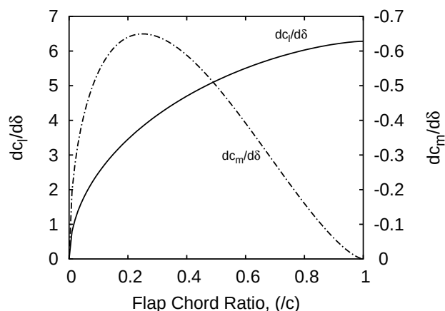
Figure 8: Theoretical lift and pitching moment characteristics of plain trailing-edge flaps
