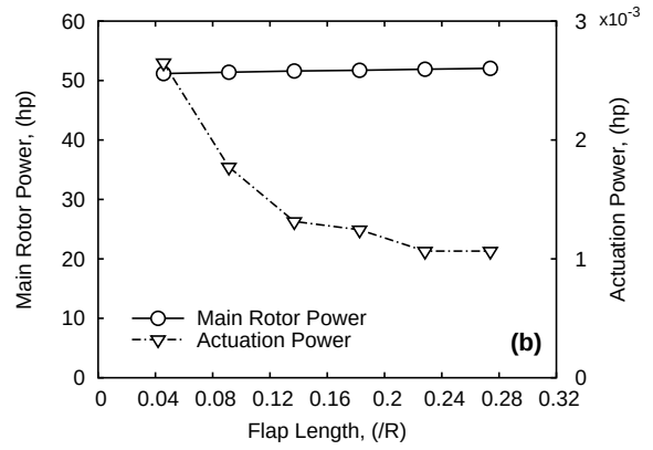
Figure 6: Effect of trailing-edge flap length on flap angles, main rotor power, and and actuation requirements at forward speed of 60 knots ( \mu = 0.16 )
