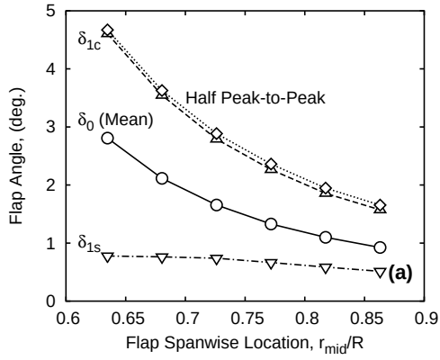
Figure 5: Effect of trailing-edge flap location on flap angles, main rotor power, and and actuation requirements at forward speed of 60 knots ( \mu = 0.16 )
