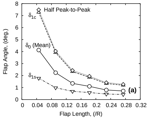
Figure 6: Effect of trailing-edge flap length on flap angles, main rotor power, and and actuation requirements at forward speed of 60 knots ( \mu = 0.16 )
