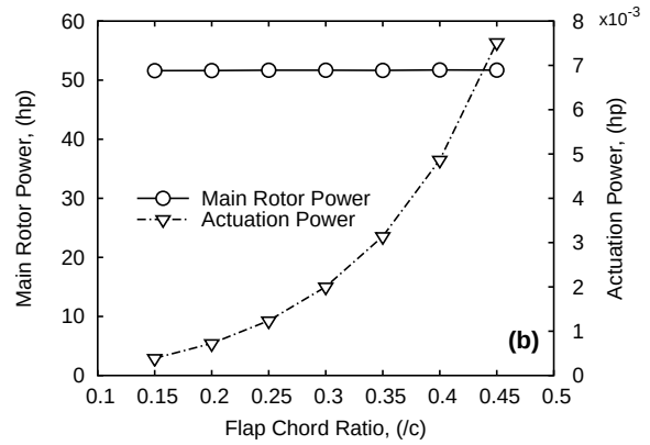
Figure 7: Effect of trailing-edge flap chord ratio on flap angles, main rotor power, and and actuation requirements at forward speed of 60 knots ( \mu = 0.16 )
