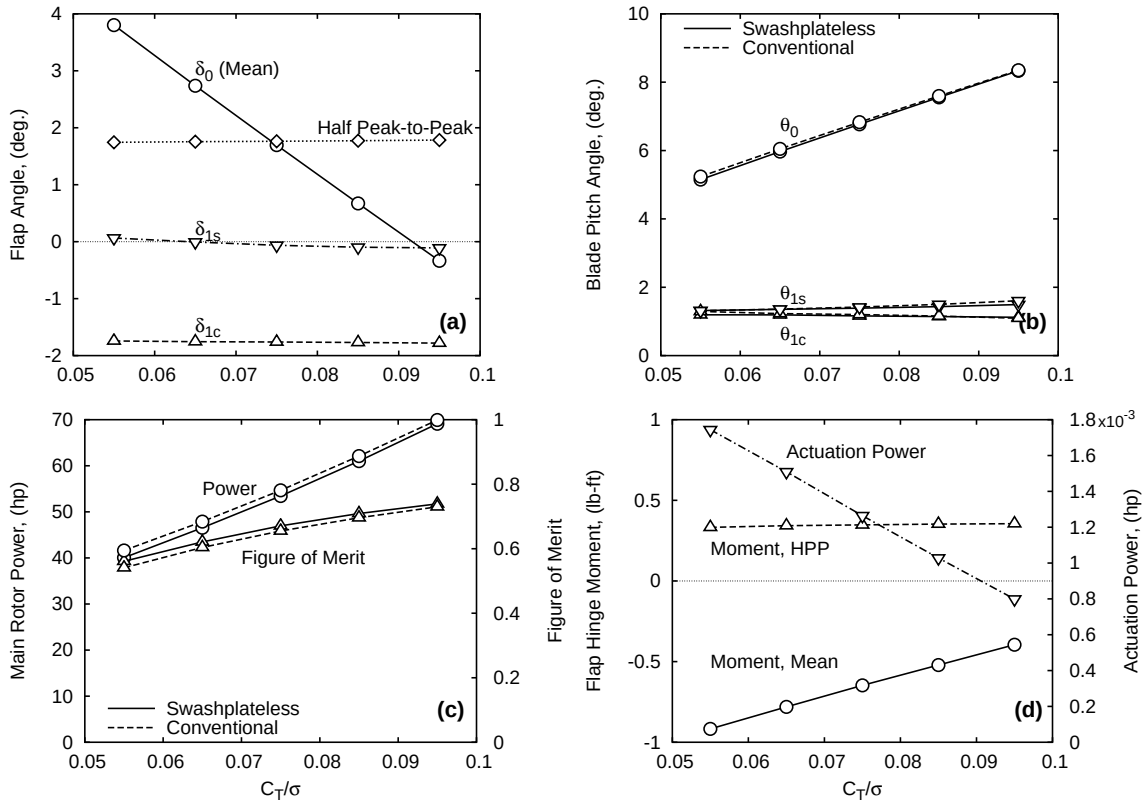
Figure 3: Comparisons of conventional and swashplateless rotors for different thrust levels at hover
