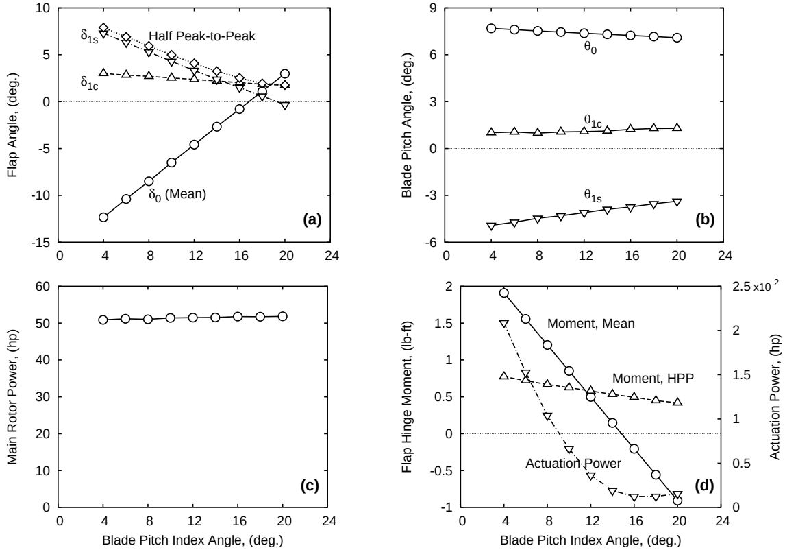
Figure 4: Effect of pitch index angle on trailing-edge flap angles, main rotor power, and and actuation requirements at forward speed of 60 knots ( \mu = 0.16 )
