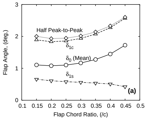
Figure 7: Effect of trailing-edge flap chord ratio on flap angles, main rotor power, and and actuation requirements at forward speed of 60 knots ( \mu = 0.16 )
