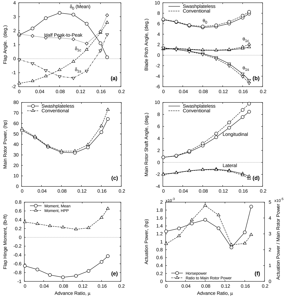
Figure 2: Comparisons of conventional and swashplateless rotor at different forward speeds
