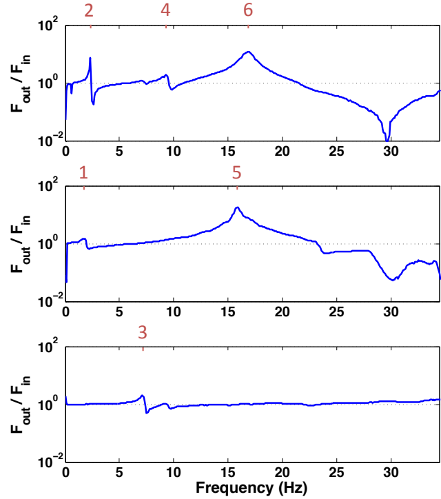
Figure 28. Mode identification for axial force, in-plane shaking at 0 deg (top); side force, in-plane shaking at 270 deg (middle); normal force, vertical shaking on-center (bottom). Note logarithmic scale on y-axis.
