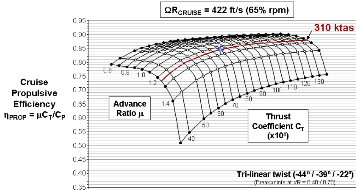
Figure 47. Rotor Cruise Propulsive Efficiency for 422 fps Cruise Tip Speed Design
