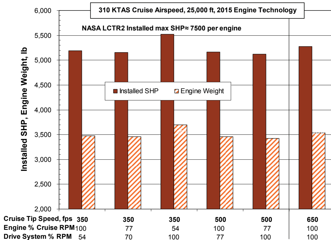
Figure 56. COTS Engine Installed SHP and Weight
