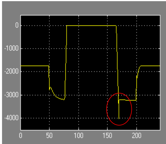
Ring Gear Torque Behavior (N*m) T=5s
