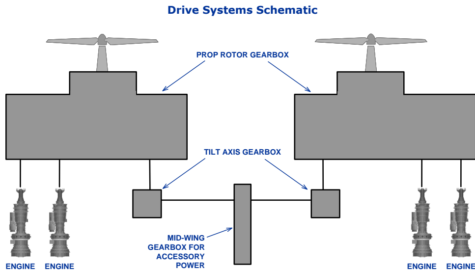
Figure 4. Drive System Block Diagram
