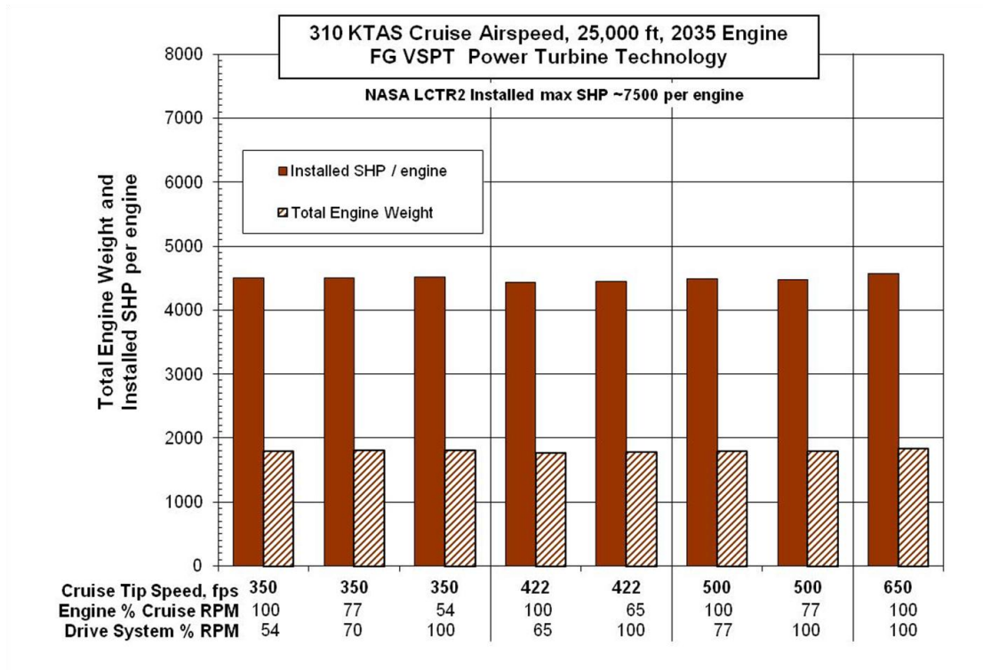
Figure 72. 2035 FG-VSPT Engine Installed SHP and Weight
