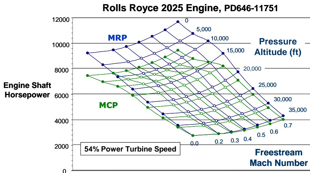
Figure 18. 2025 EIS Engine Power Available at 54% RPM
