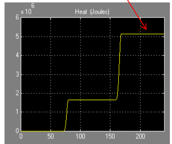
Energy Dissipation from Shifting in Joules T=10s
