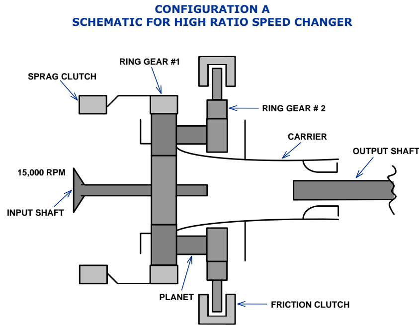
Figure 33. Speed Changing Planetary Gearbox Schematic A
