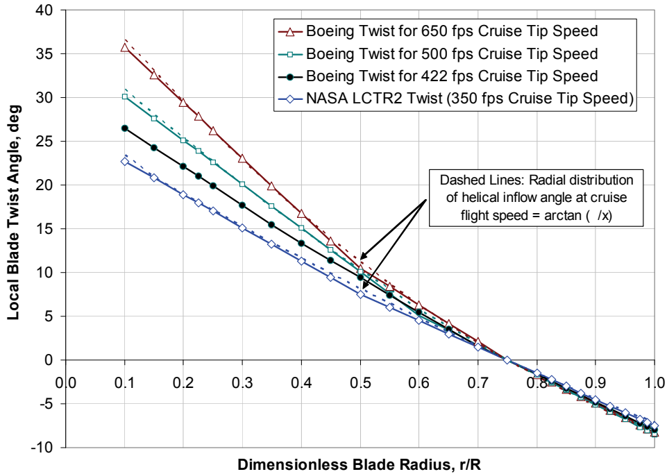
Figure 43. Comparison of Rotor Blade Twist Distributions
