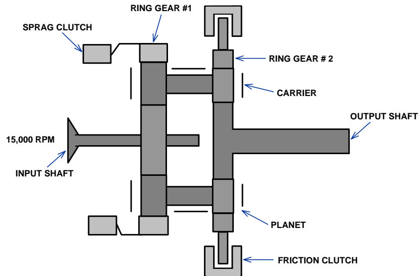
Figure 34. Speed Changing Planetary Gearbox Schematic C
