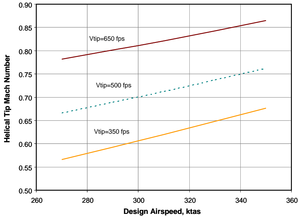
Figure 59. Rotor Blade Tip Helical Mach Number Versus Design Airspeed
