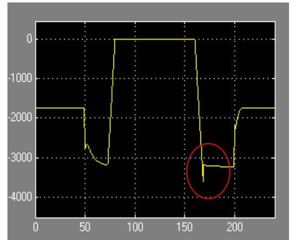
Ring Gear Torque Behavior (N*m) T=10s
