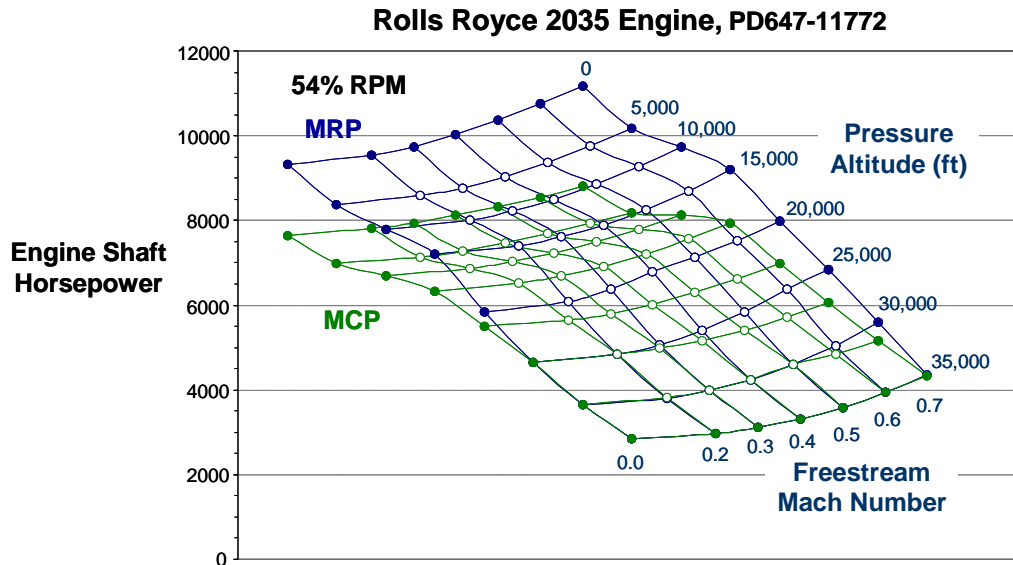
Figure 21. 2035 VG-VSPT Engine Power Available at 54% RPM
