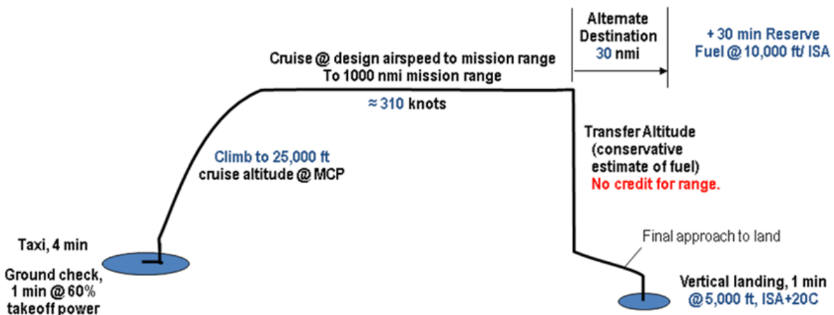
Figure 2. NASA Mission Profile for LCTR2 Study
