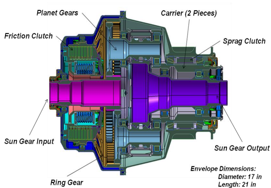
Figure 42. Speed Changer Gearbox: Section View
