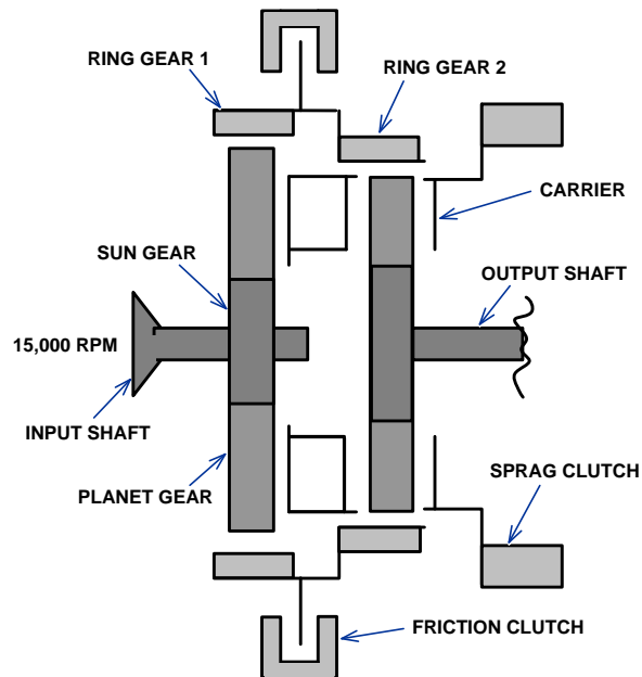
Figure 37. Speed Changing Planetary Gearbox Schematic F
