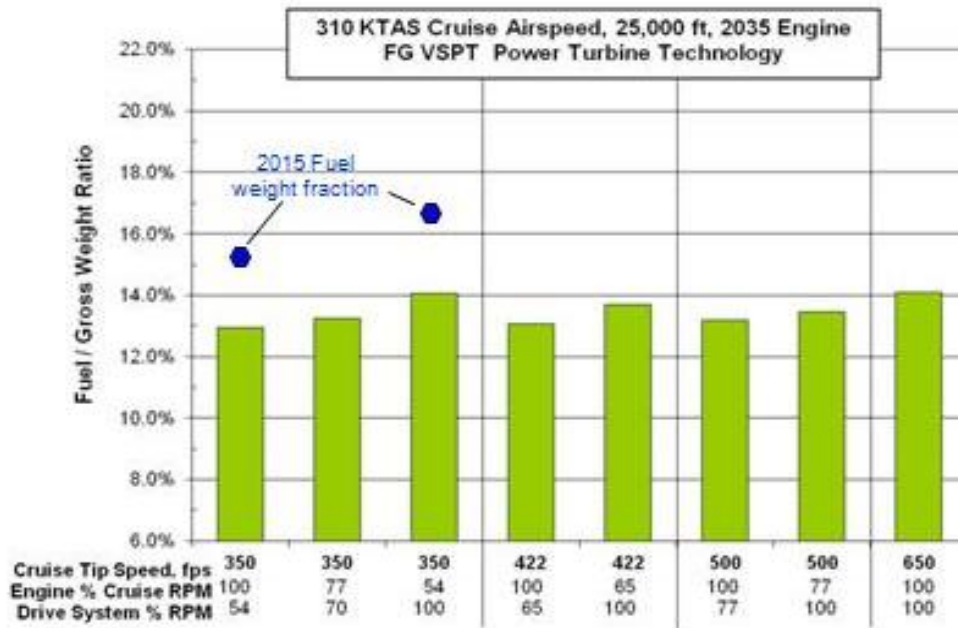
Figure 74. Mission Fuel Weight Fraction for 2035 FG-VSPT Engine
