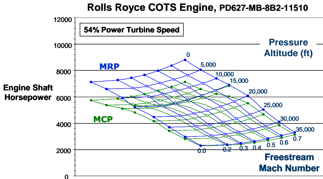
Figure 13. 2015 COTS Engine Power Available at 54% RPM
