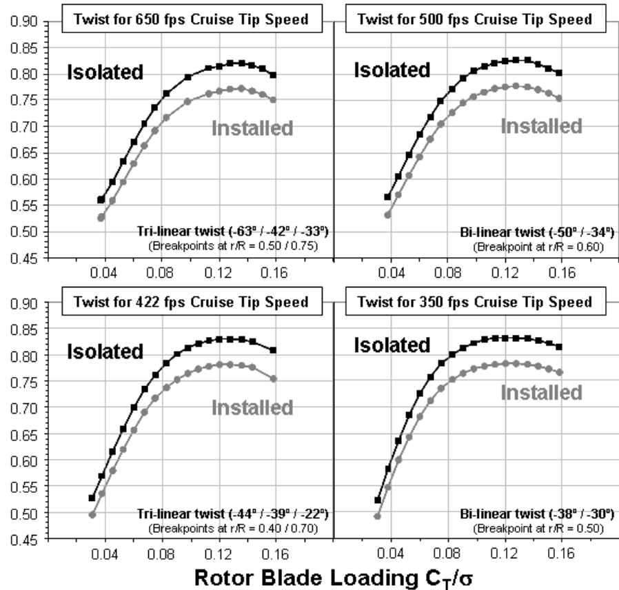
Figure 44. Rotor Hover Figure of Merit for 310 ktas cruise rotor designs
