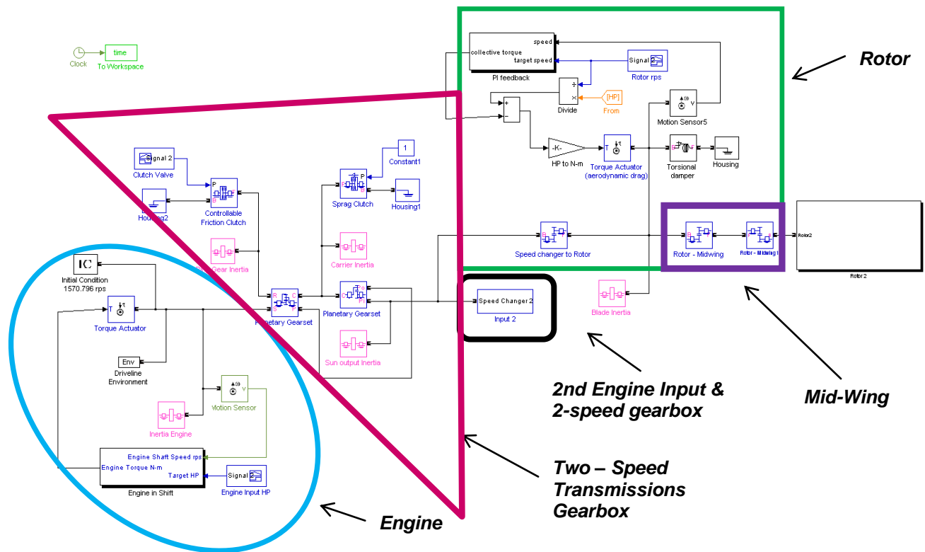
Figure 38. Matlab Model of the Drive Train
