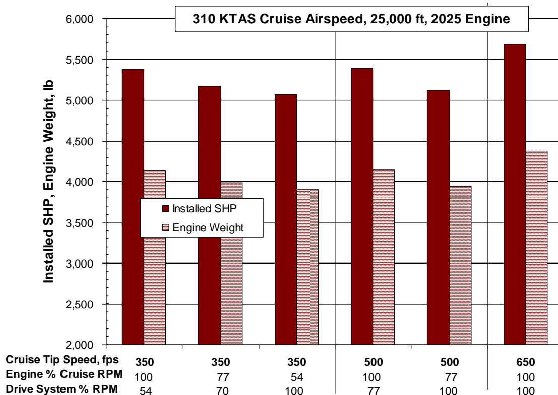
Figure 65. 2025 EIS Engine Installed SHP and Weight
