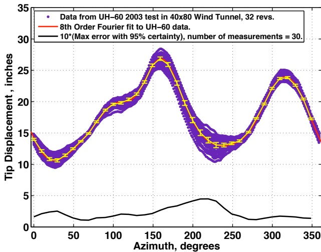
Figure 13. Assessment of the rev-to-rev variation in tip location based on non-stereo-photogrammetry measurements. Maximum error with 95% certainty, based on 30 measurements, is shown as error bars.
