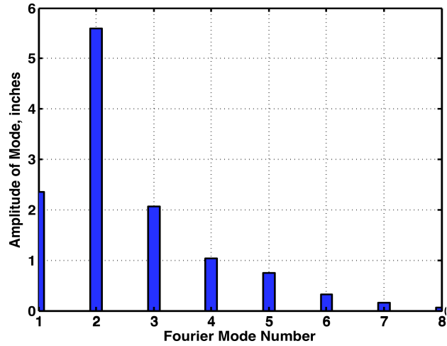
Figure 14. Estimated Fourier mode blade tip displacement amplitude based on measurements obtained in 2003 NFAC test of a UH-60 rotor system.
