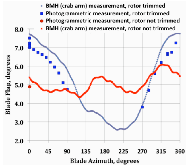
Figure 17. Comparison of measured blade flap of blade 1, C_T/\sigma=0.078 , \mu=0.25 , \alpha_s=-3.0 deg, q=38.9 lb/ft 2 .
