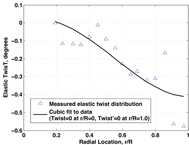
Figure 16. Elastic twist of blade 1, C_T/\sigma=0.078 , \mu=0.20 , \alpha_s=-1.6 deg, q=24.8 lb/ft 2 , \Psi = 40 deg.
