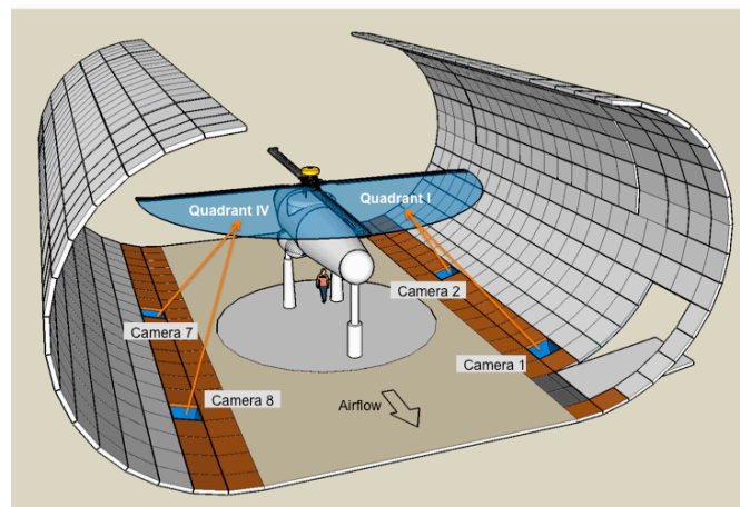
Figure 3. 40-ft by 80-foot test section schematic showing camera cavity locations for the two quadrant photogrammetry measurements.
