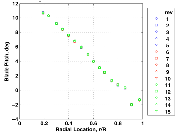
Figure 15. Measured pitch distribution \mu=0.20 , \alpha_s = -1.6 deg, C_T/\sigma = 0.078 , collective = 6.7 deg, \Psi = 40 deg.
