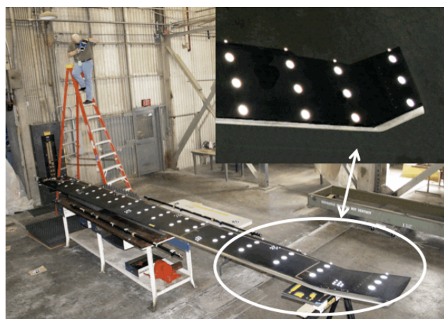
Figure 5. Blade with two-inch diameter retro reflective targets installed.
