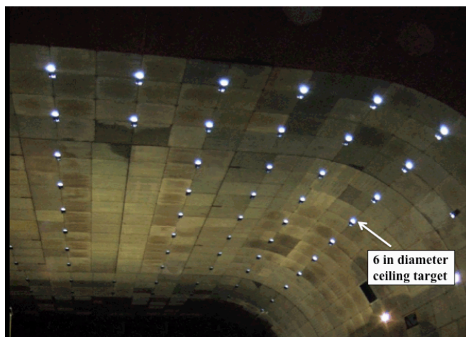
Figure 6. Ceiling of the test section with six-inch diameter targets installed.
