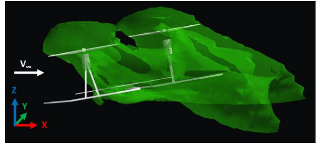
Figure 19. LILI in forward flight mode: velocity magnitude iso surface flow field prediction ( \theta_{S, \text{front}} = 20^\circ , \theta_{0, \text{front}} = 10^\circ , C_{T, \text{front}} = 0.031 , \theta_{0, \text{rear}} = 10^\circ , \theta_{S, \text{rear}} = 20^\circ , C_{T, \text{rear}} = 0.028 ).
