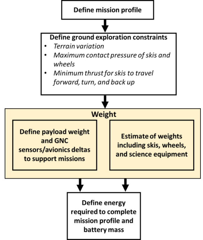
Figure 9. LILI design flow chart.
