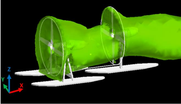
Figure 18. LILI in ground mobility mode: velocity magnitude iso surface flow field prediction ( \theta_{S, \text{front}} = 90^\circ , \theta_{0, \text{front}} = 10^\circ , C_{T, \text{front}} = 0.0315 , \theta_{S, \text{rear}} = 90^\circ , \theta_{0, \text{rear}} = 10^\circ , C_{T, \text{rear}} = 0.0281 ).
