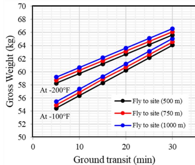
Figure 11. Gross Weight verses ground transit for variation in fly to site distance and temperature.
