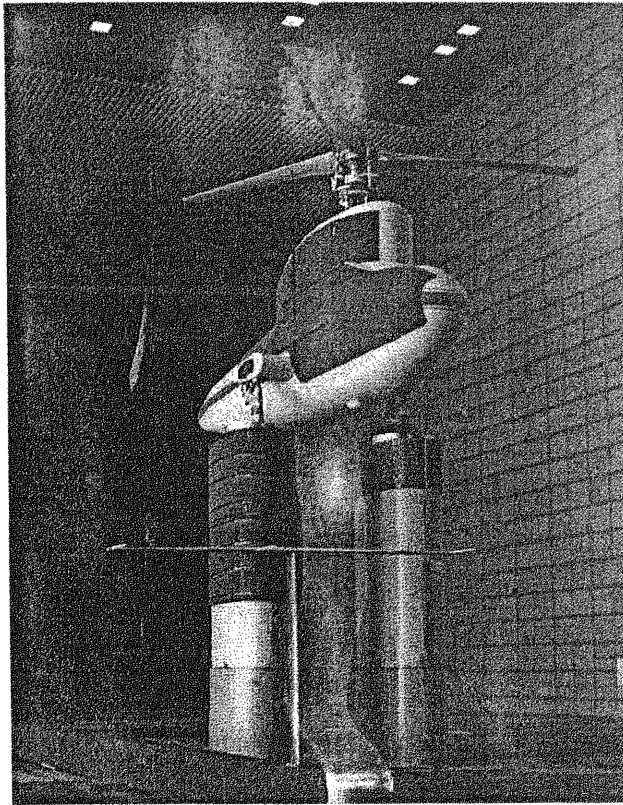
Figure 16. The XV-15 right-hand rotor mounted on the RTA in the 80- by 120-Foot Wind Tunnel.
