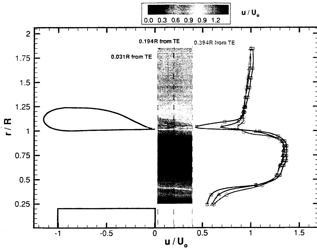
Fig. 19 Duct exit velocity profiles in propeller mode at \alpha = 0^\circ , r_{LE}/c = 0.05 , \Delta r_t/R = 0.01 , V_o = 41 \text{ kts} , 9000RPM.
