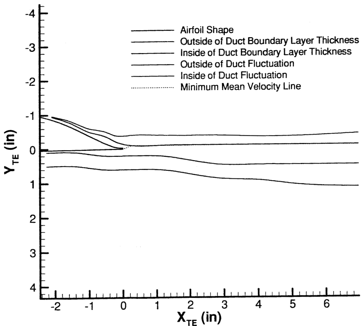
Fig. 20 Measured internal/external boundary layer geometry and duct exit wake thickness in propeller mode at \alpha = 0^\circ , r_{LE}/c = 0.05 , \Delta r_1/R = 0.01 , V_o = 41 \text{ kts} , 9000 \text{ RPM} .
