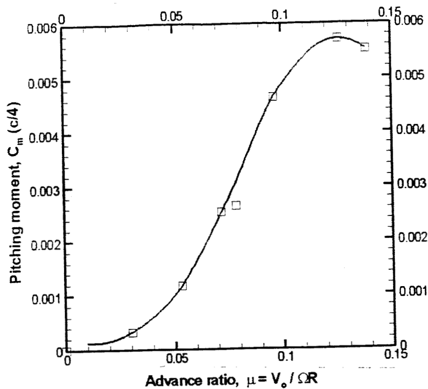
Fig. 12 Development of pitching moment instability in hover with increasing crosswind velocity component, r_{LE}/c = 0.05 , \Delta r_l/R = 0.02 , 9000 RPM.
