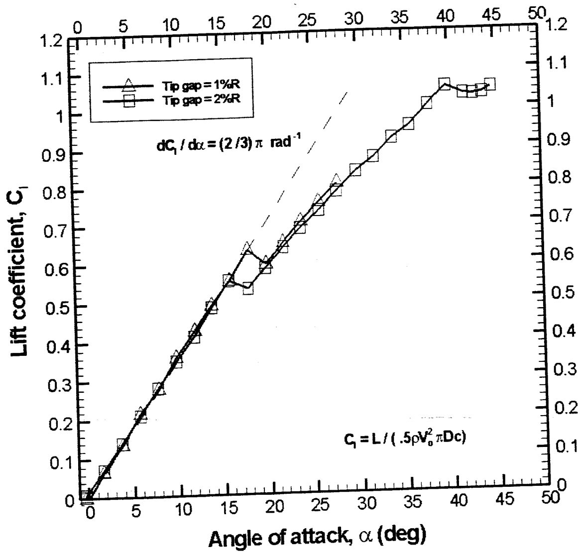
Fig. 16 Effect of tip gap on stall performance, c_{fLE}/c = 0.05 , V_o = 35 \text{ kts} , 9000 RPM.
