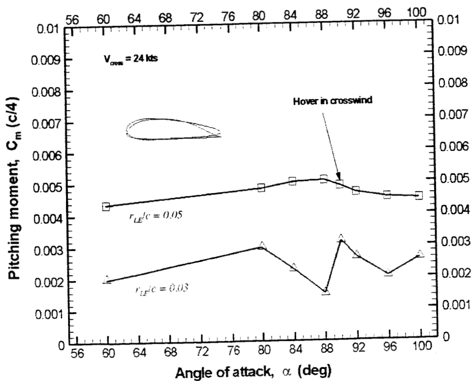
Fig. 13 Alleviation of pitching moment instability in hover with decrease in duct leading edge radius, \Delta r_l/R = 0.02 , V_\infty = 24 kts, 9000 RPM.
