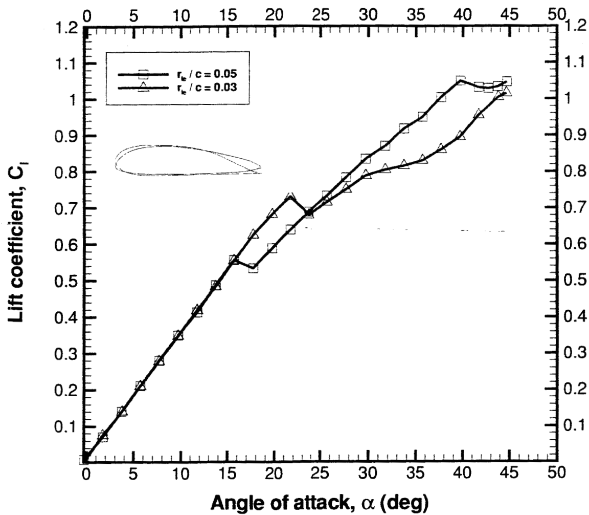
Fig. 17 Effect of duct leading edge radius on stall performance: lift coefficient, \Delta r_t/R = 0.02 , V_o = 35 \text{ kts} , 9000 RPM.
