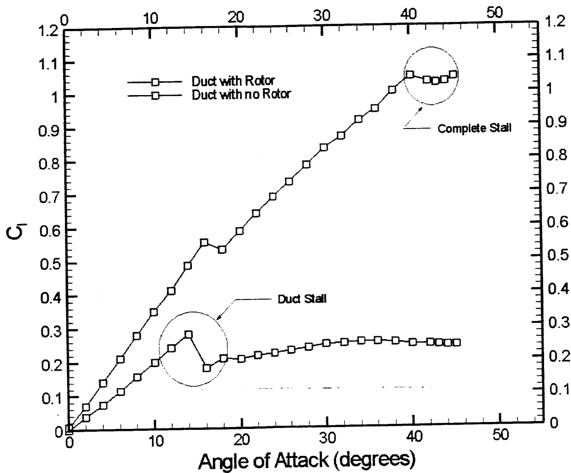
Fig. 14 Comparison of stall performance of isolated duct and rotor/duct combination. J_{LE}/c = 0.05 , \Delta r_t/R = 0.02 , V_o = 35 kts, 9000 RPM.
