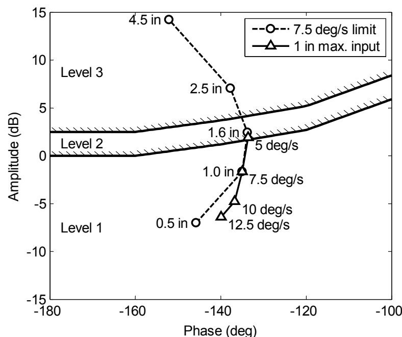
Figure 76. OLOP specifications for varying nacelle rate limits (15 ft/s/in sensitivity and 1.0 in maximum pilot input).
