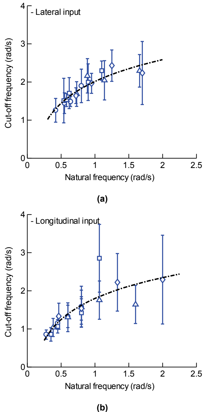
Figure 52. Relationship between pilot input cutoff frequencies and aircraft second-order response dynamics for Hover MTE: (a) lateral axis and (b) longitudinal axis.
