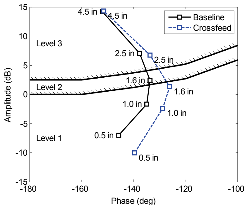
Figure 78. Effect of crossfeed on OLOP specifications for TRC control (15 ft/s/in control sensitivity and \pm 7.5 deg/s rate limits).
