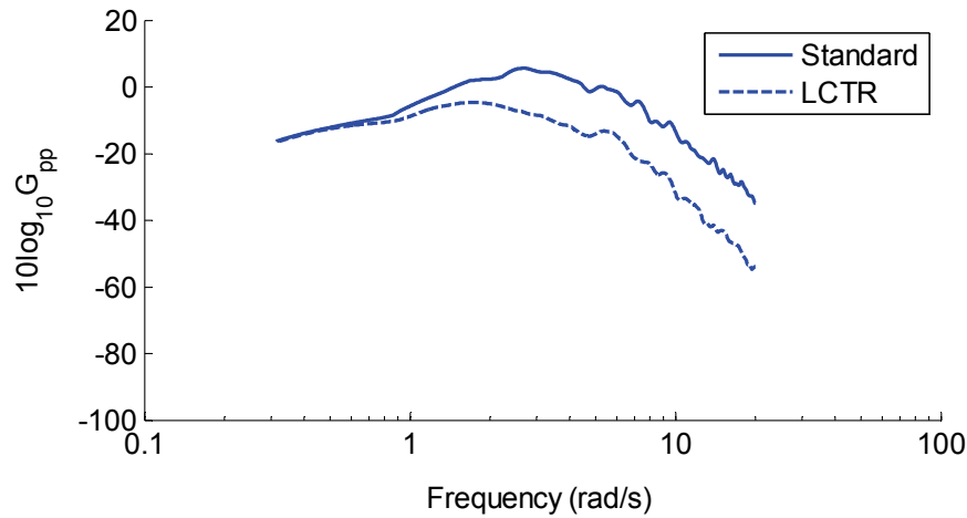
Figure 11. Roll rate auto spectrum comparison for the standard and tiltrotor CETI model implementations on the LCTR2 (ACAH).
