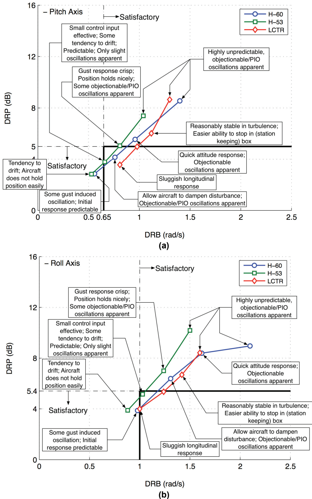
Figure 36. Proposed boundaries for attitude DRB and DRP: (a) pitch and (b) roll.
