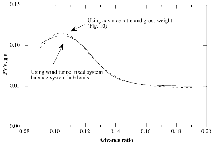
Fig. 19. PVV prediction using six components of N/rev balance-system hub loads and operating parameters ( C_w/\sigma = 0.08 ).
