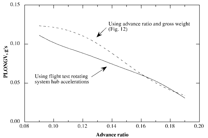
Fig. 15. PLONGV prediction using flight test rotating system hub accelerations and operating parameters ( C_W/\sigma = 0.08 ).
