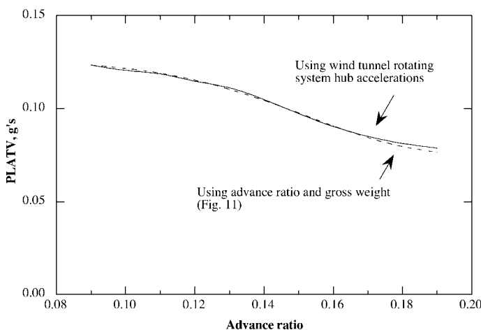
Fig. 17. PLATV prediction using wind tunnel rotating system hub accelerations and operating parameters ( C_W/\sigma = 0.08 ).
