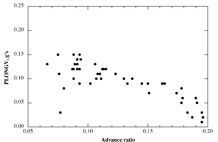
Fig. 3. UH-60A peak, N/\text{rev} pilot floor longitudinal vibration, PLONGV, variation with advance ratio.
