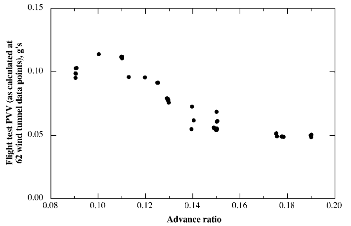
Fig. 10. Predicted flight test PVV using advance ratio and gross weight, evaluated at 62 wind tunnel data points, includes thrust variations.
