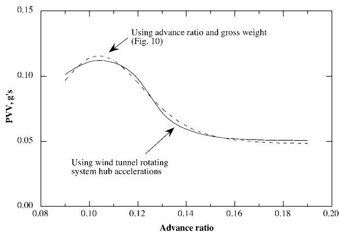
Fig. 16. PVV prediction using wind tunnel rotating system hub accelerations and operating parameters ( C_W/\sigma = 0.08 ).
