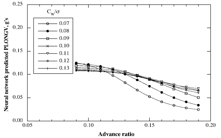
Fig. 9. Predicted PLONGV trends using advance ratio and gross weight.
