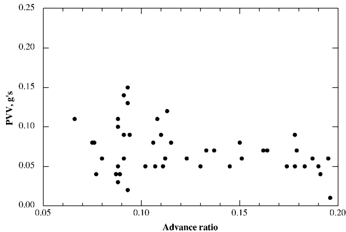
Fig. 1. UH-60A peak, N/\text{rev} pilot floor vertical vibration, PVV, variation with advance ratio.
