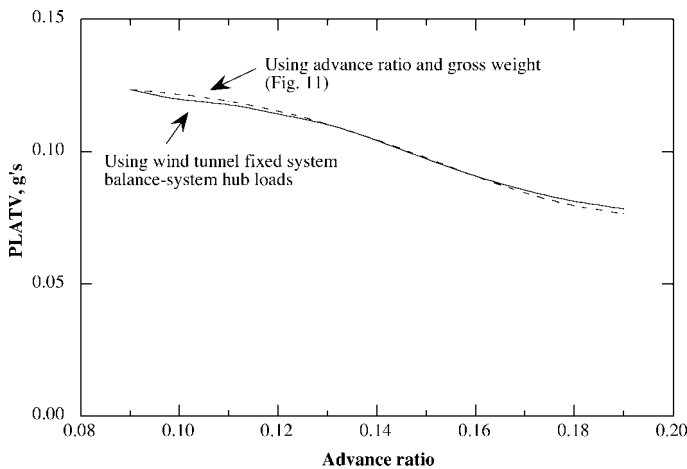
Fig. 20. PLATV prediction using six components of N/rev balance-system hub loads and operating parameters ( C_w/\sigma = 0.08 ).
