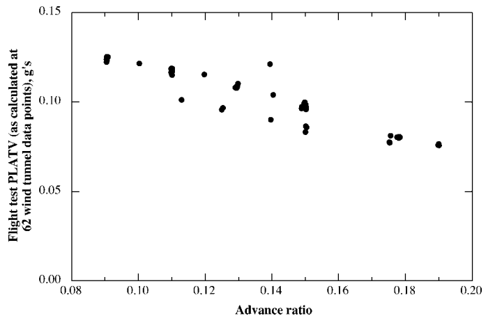
Fig. 11. Predicted flight test PLATV using advance ratio and gross weight, evaluated at 62 wind tunnel data points, includes thrust variations.
