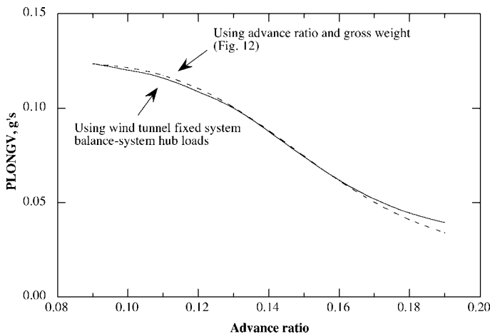
Fig. 21. PLONGV prediction using six components of N/rev balance-system hub loads and operating parameters ( C_w/\sigma = 0.08 ).
