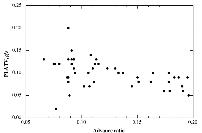
Fig. 2. UH-60A peak, N/\text{rev} pilot floor lateral vibration, PLATV, variation with advance ratio.
