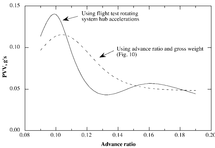
Fig. 13. PVV prediction using flight test rotating system hub accelerations and operating parameters ( C_W/\sigma = 0.08 ).
