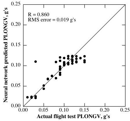
Fig. 6. PLONGV correlation using advance ratio and gross weight.
