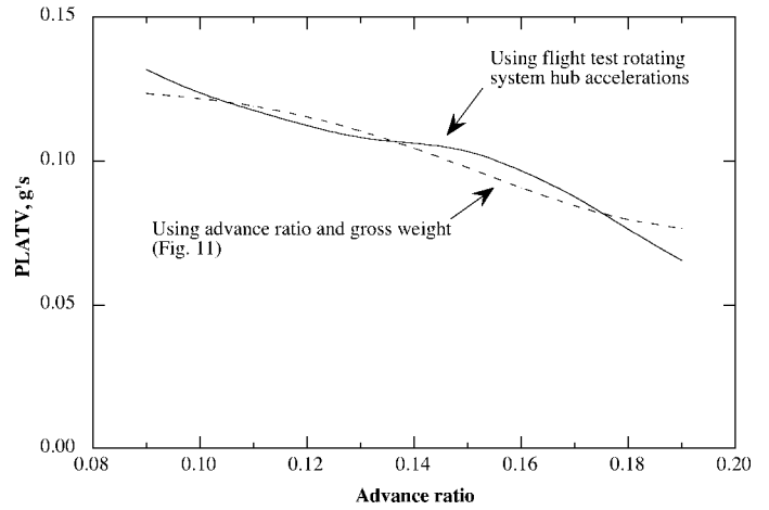
Fig. 14. PLATV prediction using flight test rotating system hub accelerations and operating parameters ( C_W/\sigma = 0.08 ).
