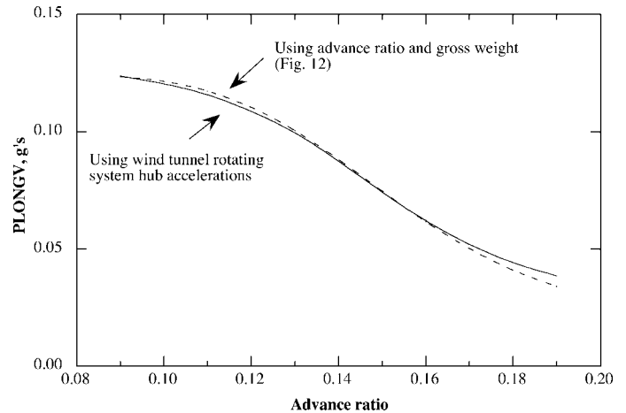
Fig. 18. PLONGV prediction using wind tunnel rotating system hub accelerations and operating parameters ( C_W/\sigma = 0.08 ).
