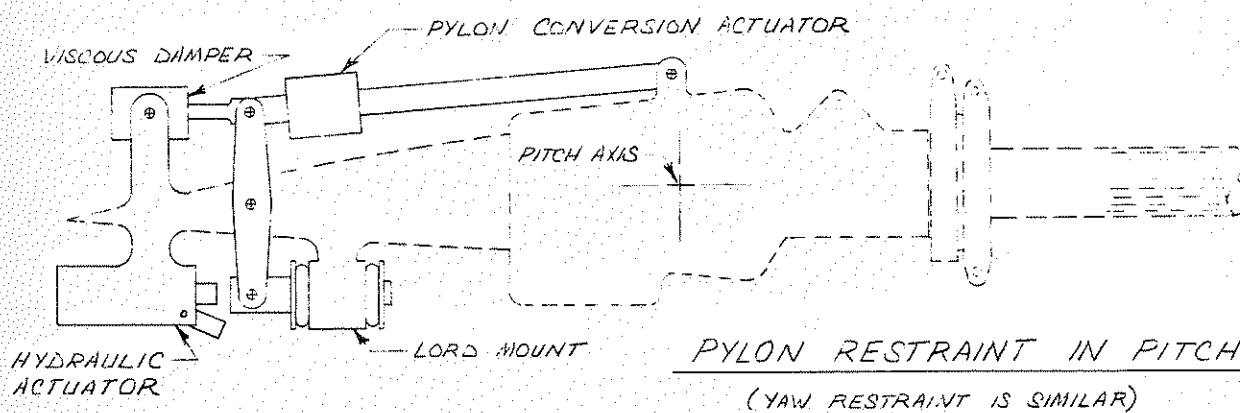
(9) Swashplate Coupling and Pylon Restraint Figure 3. - Concluded.
