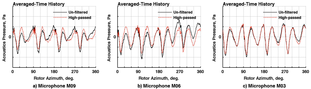
Figure 3. High-pass filtering of measured acoustic time histories.
