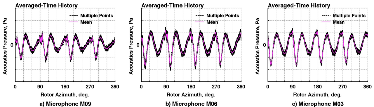
Figure 4. Repeatability of acoustics measurements for baseline condition.
