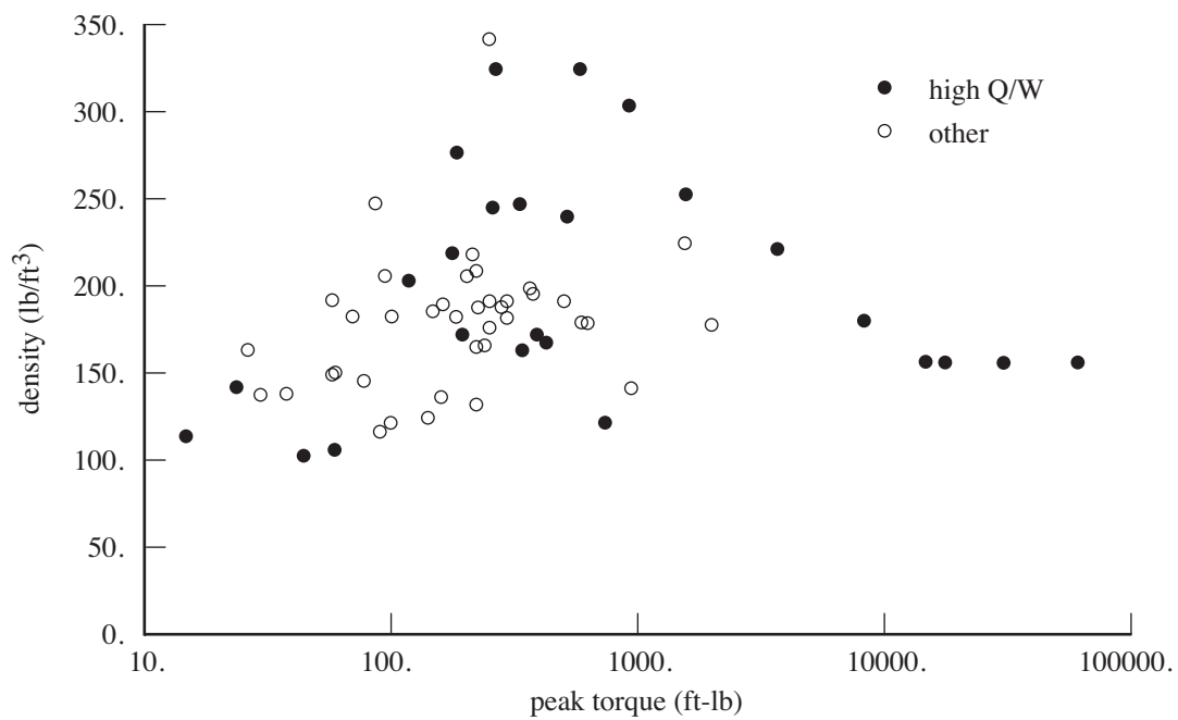
Figure 24-4. Motor density.
