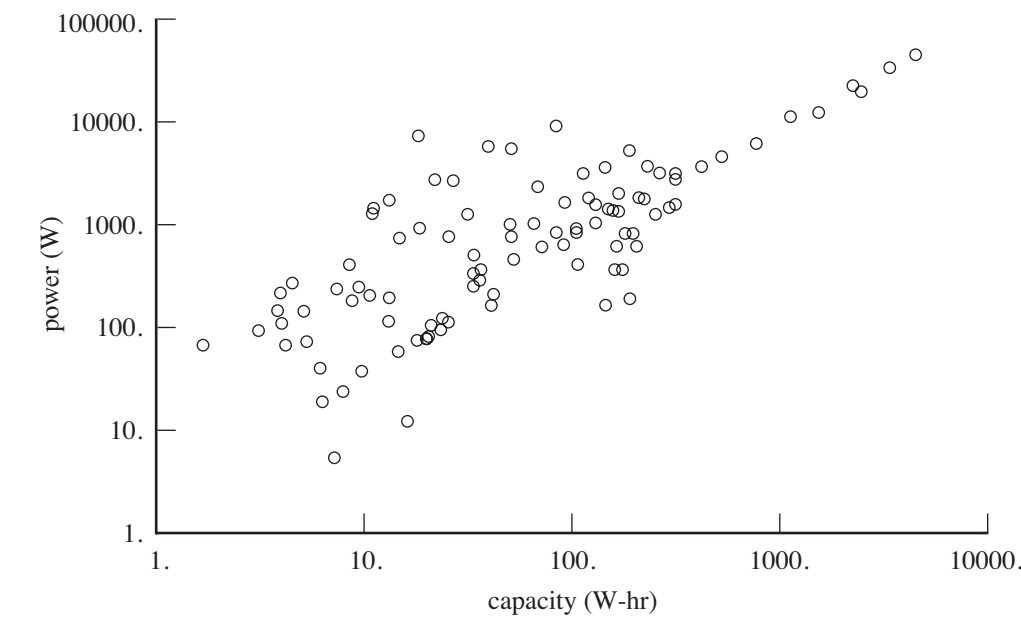
Figure 28-1. Lithium-ion battery capacity (W-hr) and power (W).
