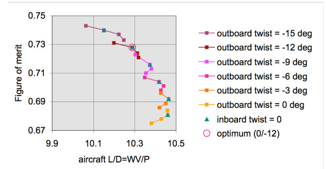
Figure 11. LCTR twist optimization.
