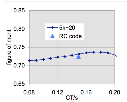
Figure 12. LCTR rotor hover performance.
