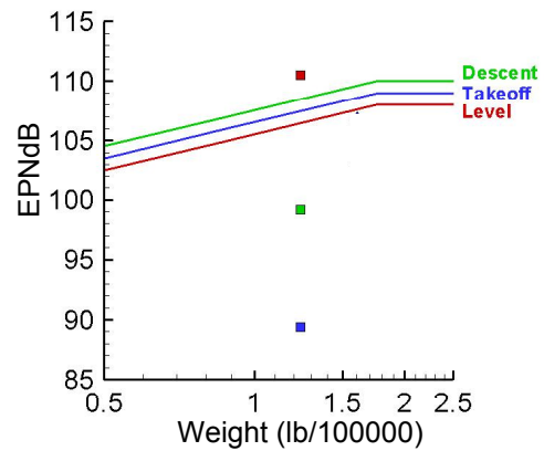
(a) Descent, takeoff, and level flight.
