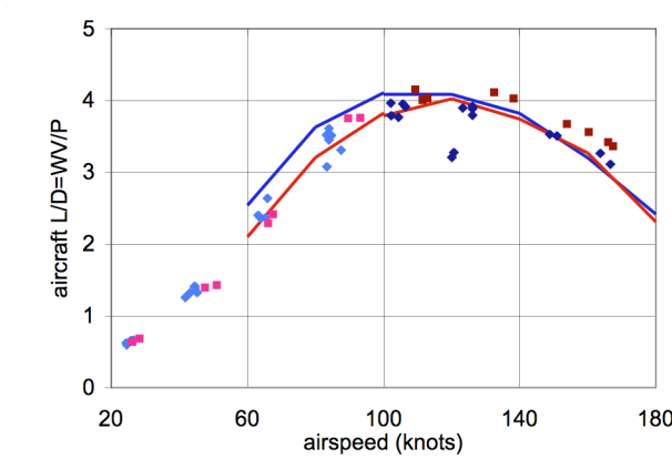
Figure 30. Comparison of XH-59A forward flight performance with CAMRADII calculations.
