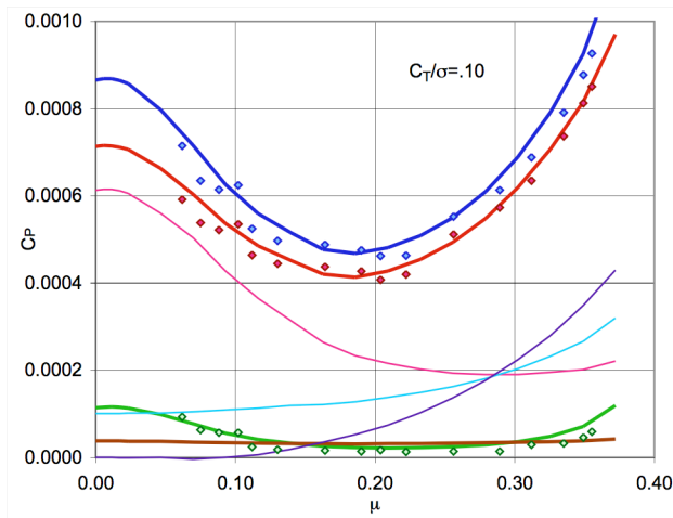
Figure 16. Comparison of UH-60A Airloads flight test performance with NDARC calculations.
