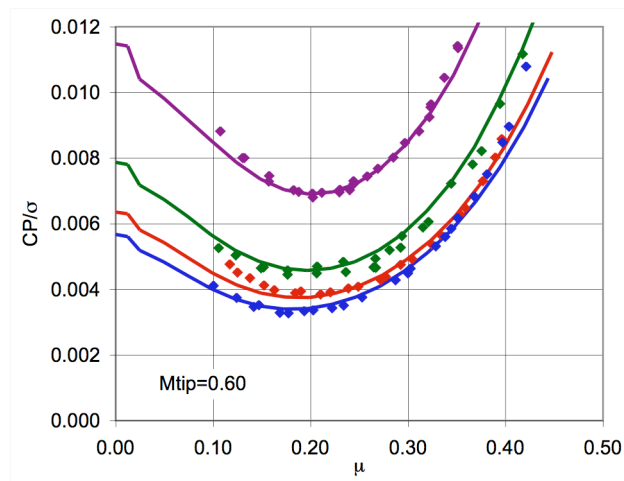
Figure 28. Comparison of CH-47D forward flight performance with NDARC calculations.
