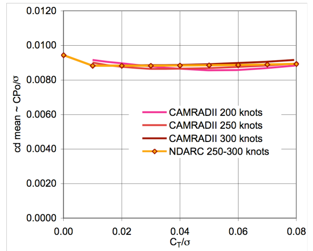
Figure 52. XV-15 rotor model: cruise profile power (axial flight).
