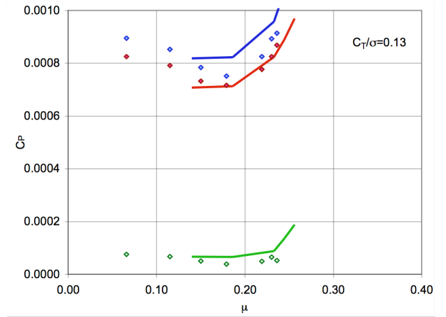
Figure 4. Comparison of UH-60A Airloads flight test performance with CAMRADII calculations.
