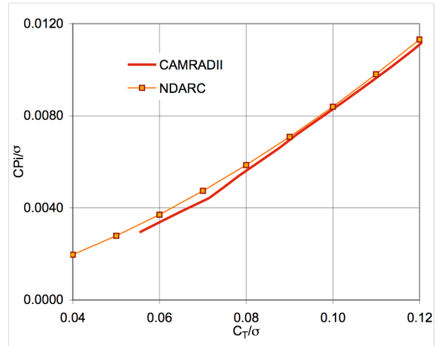
Figure 21. CH-47D rotor model: hover induced power for tandem rotors.
