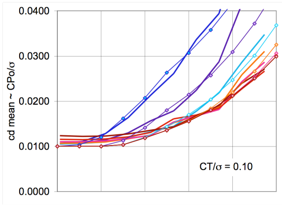
(a) NDARC parameters to match CAMRADII single rotor profile power
