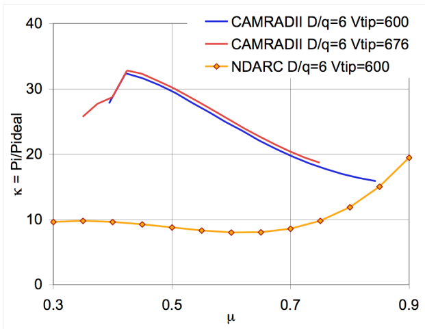
Figure 50. XV-15 rotor model: airplane mode induced power (nacelle angle 0 deg).
