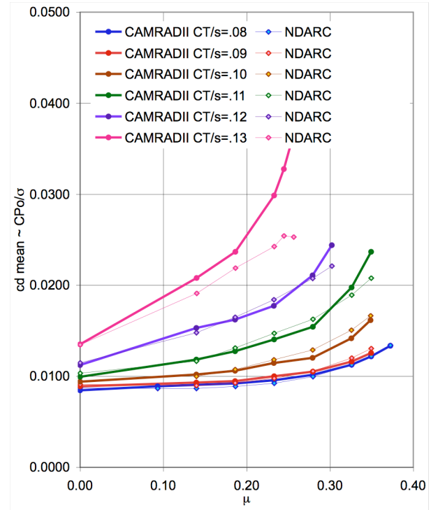
Figure 10. UH-60A rotor model: forward flight profile power.
