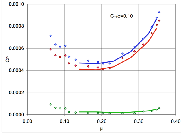
Figure 4. Comparison of UH-60A Airloads flight test performance with CAMRADII calculations.
