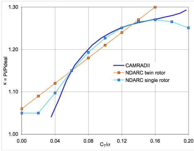
Figure 19. CH-47D rotor model: hover induced power for single rotor.
