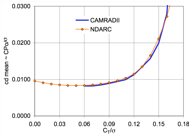
Figure 7. UH-60A rotor model: hover profile power.
