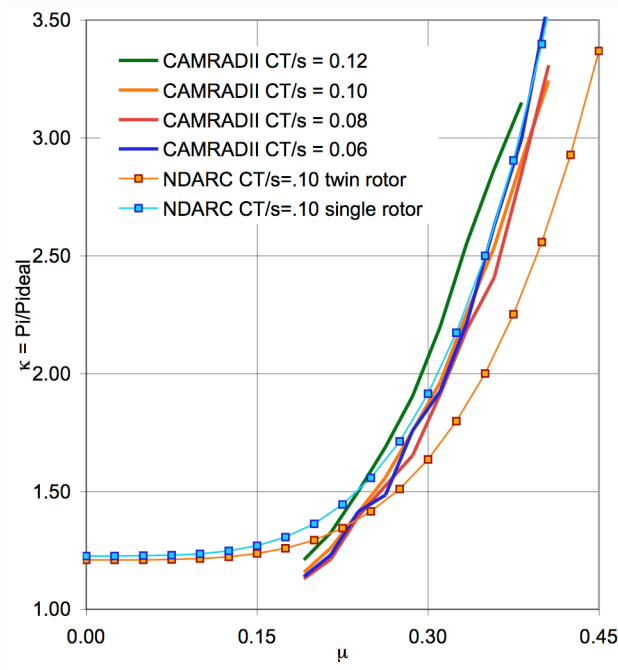
Figure 20. CH-47D rotor model: forward flight induced power for single rotor.
