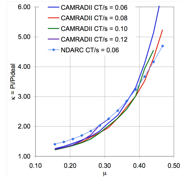
Figure 33. XH-59A rotor model: forward flight induced power for single rotor, helicopter operation.
