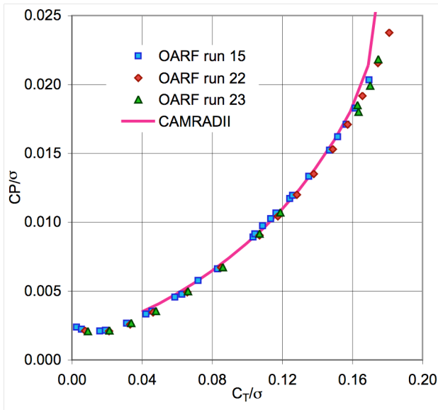
Figure 43. Comparison of XV-15 rotor hover performance with CAMRADII calculations.
