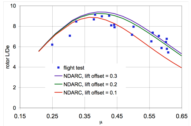
Figure 42. Comparison of XH-59A forward flight performance (using auxiliary propulsion) with NDARC calculations.
