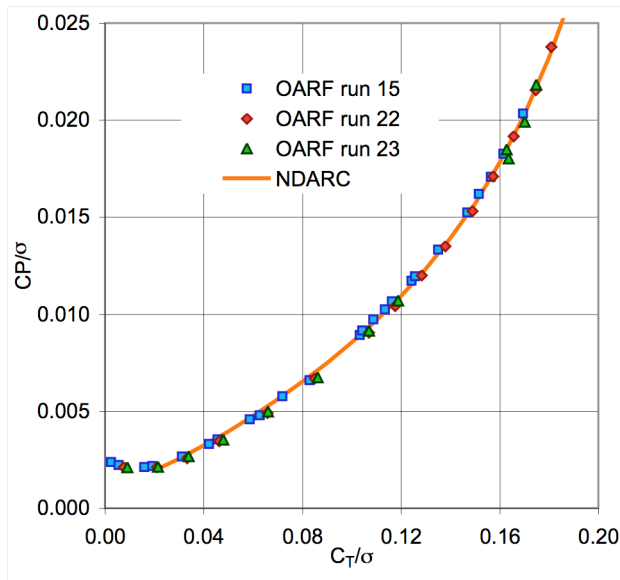
Figure 58. Comparison of XV-15 rotor hover performance with NDARC calculations.
