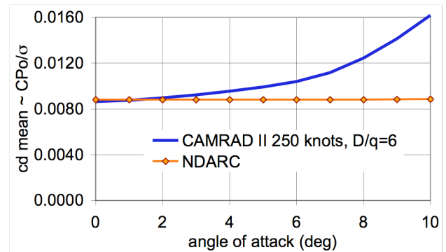
Figure 57. XV-15 rotor model: influence of shaft angle-of-attack on induced and profile power in cruise.
