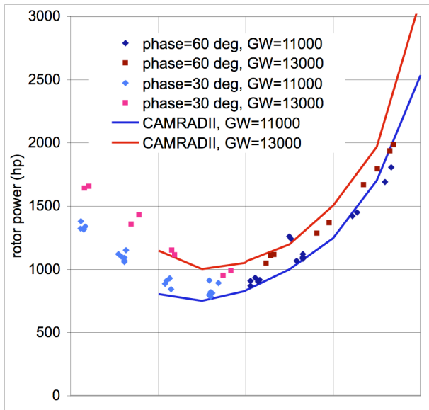
Figure 29. Comparison of XH-59A hover performance with CAMRADII calculations.
