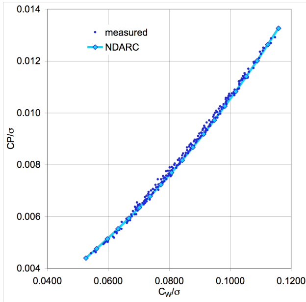
(a) rotor power
