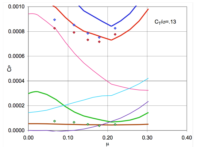
Figure 16. Comparison of UH-60A Airloads flight test performance with NDARC calculations.
