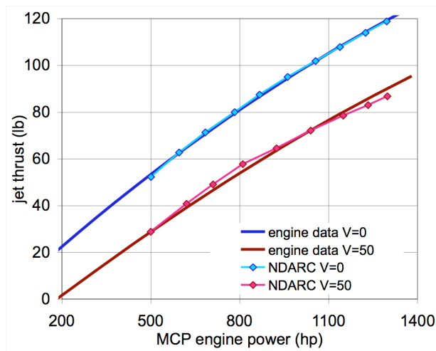
Figure 45. XV-15 engine jet thrust.
