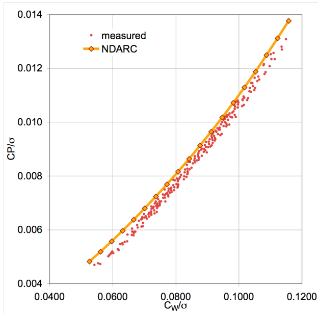
(b) aircraft power
