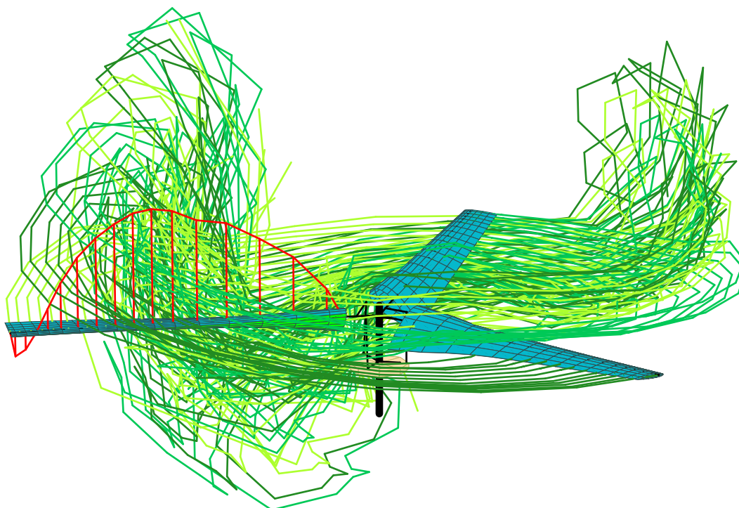
Figure 25b. Calculated TRAM wake geometry and loading for \mu = 0.15 , \alpha_s = 6 , C_T/\sigma = 0.089 . Multiple-trailer wake model, azimuth of reference blade = 105 deg.
