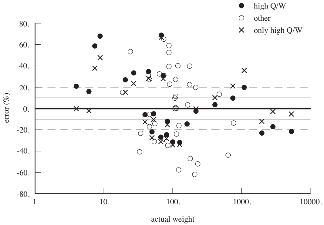
Figure 22-5. Motor weight (NASA15).
