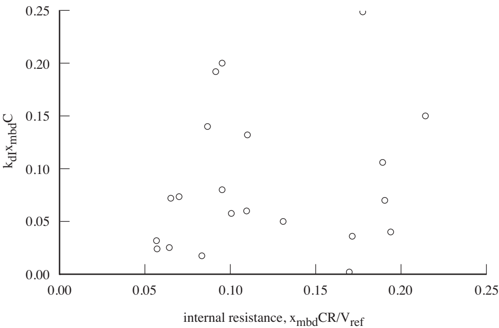
Figure 26-9. Lithium-ion battery discharge model, current parameters.
