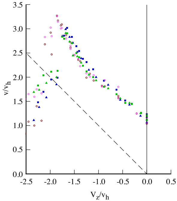
Figure 9c. Castles and Gray (1951) wind tunnel test: axial flow; \sigma = 0.05 , \theta_{tw} = -12 deg, constant chord.
