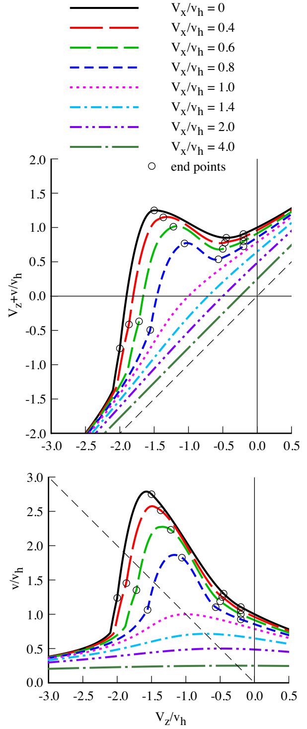
Figure 39. VRS model.
