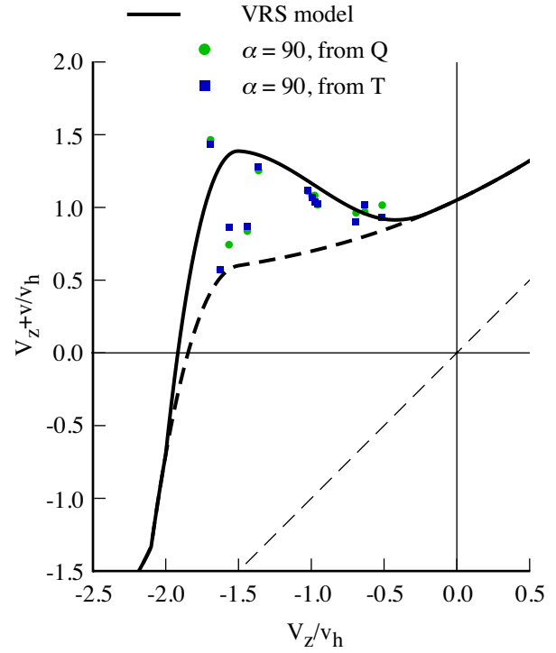
Figure 44. Betzina (2001) wind tunnel test: axial flow; \sigma = 0.1194 , \theta_{tw} = -41^\circ , rotor only; \kappa = 1.05 .
