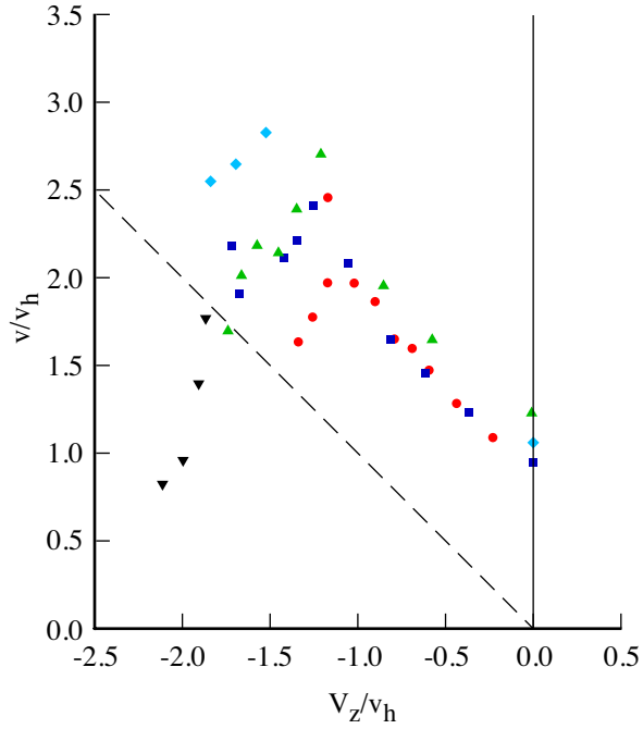
Figure 12. Washizu (1966) moving track test: axial flow; \sigma = 0.0573 , \theta_{tw} = -8.33 deg.
