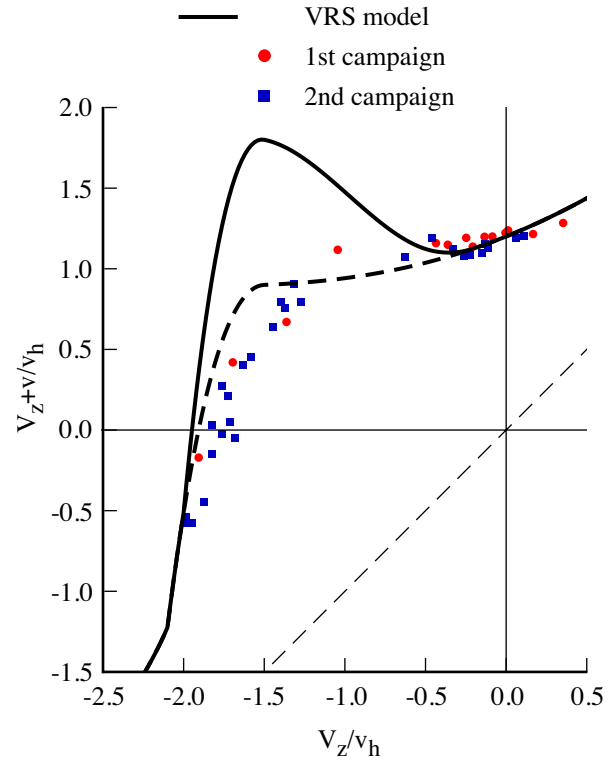
Figure 45. Taghizad (2002) flight test: axial flow; \sigma = 0.083 , \theta_{tw} = -10^\circ ; \kappa = 1.20 .
