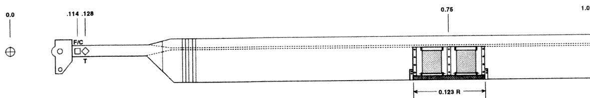
Fig. 2a. Blade planform showing Flap (F), Chord (C), and Torsion (T) strain gage locations on root flexure, as well as transition, constant blade, and active elevon section (approximate scale).
