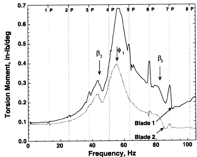
Fig. 13. Blade-to-blade variation in blade root torsion moment frequency response function magnitude, RPM = 760.
