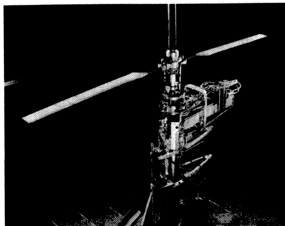
Fig. 1. Rotor installed on the Small Scale Rotor Test Rig in the US Army Aeroflightdynamics Directorate Hover Test Chamber.
