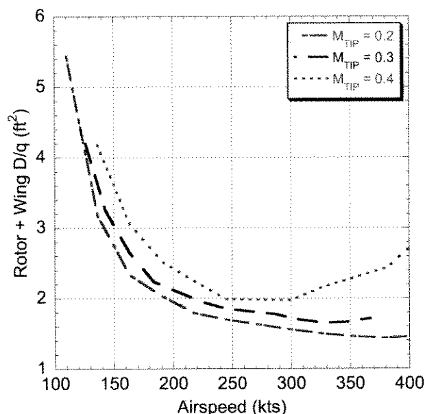
Fig. 31. D/q of rotor and wing at tip Mach numbers of 0.2–0.4, 0 deg collective pitch.
