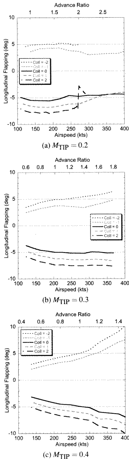
Fig. 20. Longitudinal flapping vs. airspeed from -2 to 2 deg collective, 0.2 \leq M_{TIP} \leq 0.4 .
