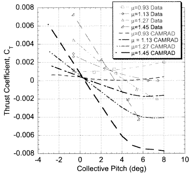
Fig. 1. Thrust correlation with high advance ratio data from reference 9, \alpha_s = 0.5 deg.
