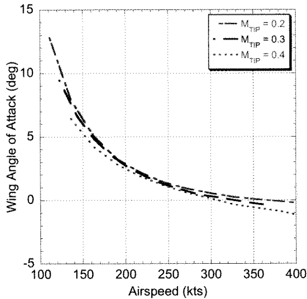
Fig. 25. Wing angle of attack at tip Mach numbers of 0.2–0.4, 0 deg collective pitch.
