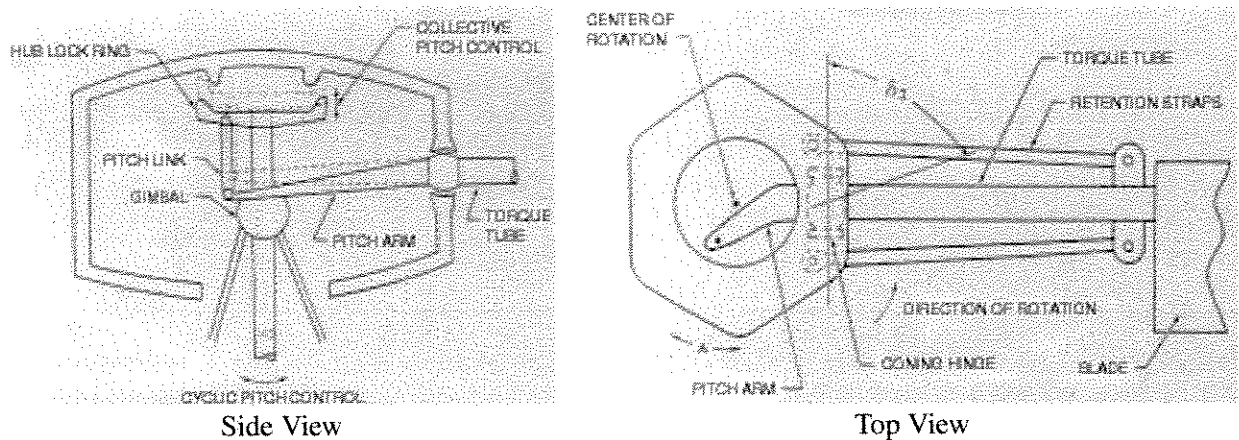
Fig. 6. Top and side view schematics of the XV-1 hub and blade assembly from reference 11.
