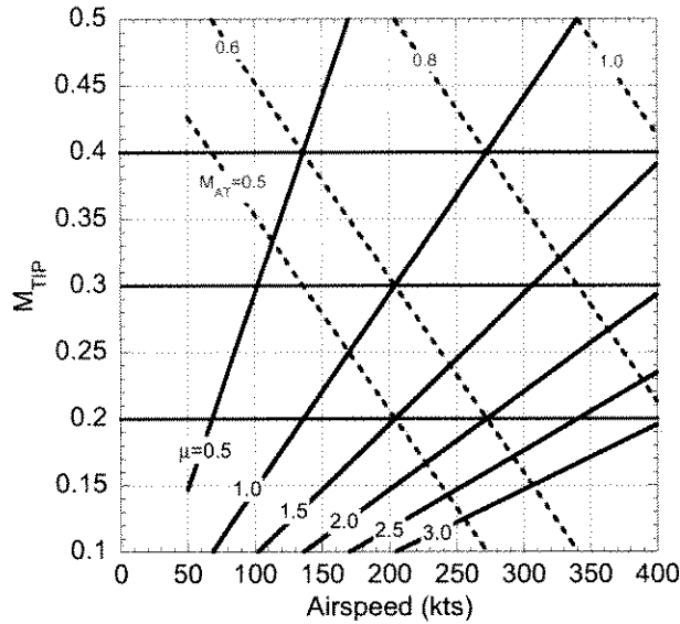
Fig. 11. Relationship between flight speed, hover tip Mach number, and advancing tip Mach number.
