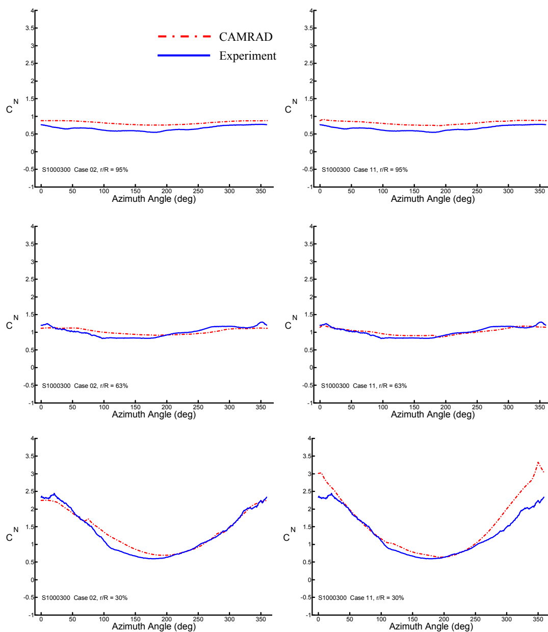
Figure 18 -- Dynamic Stall Model Effect 10 m/s, 30° Yaw Error
