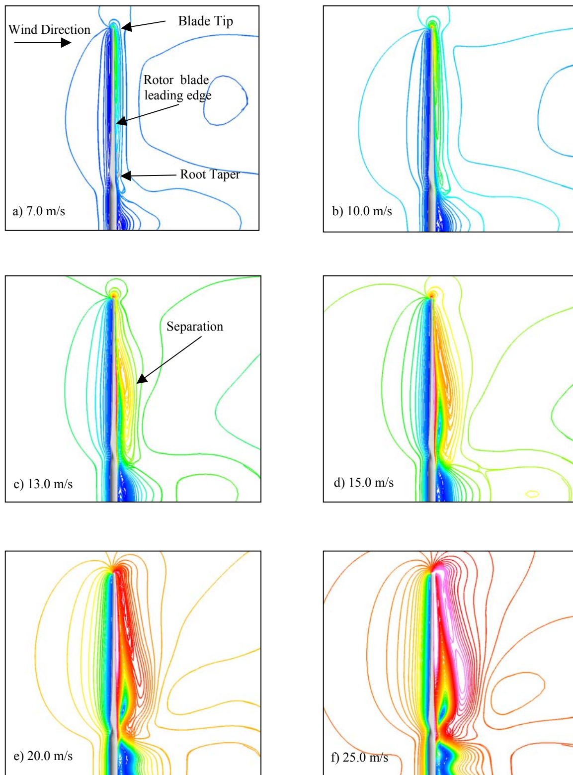
Figure 12 - Velocity Contours Cut-Plane x=0.0
