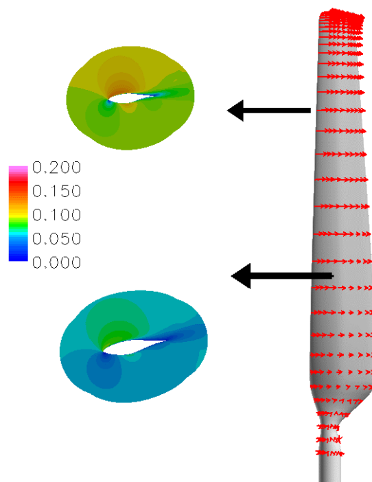
Figure 13 - Velocity Contour and Vectors Non-Inertial Coordinates, 7 m/s
