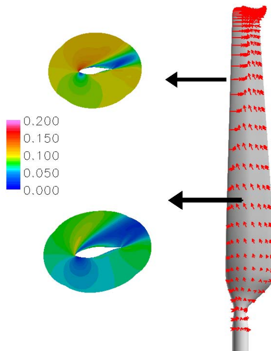
Figure 14 - Velocity Contour and Vectors Non-Inertial Coordinates, 13 m/s
