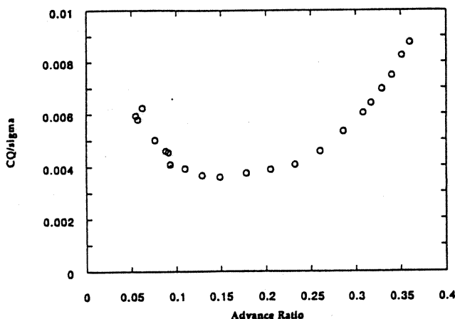
Fig. 4 Torque coefficient as a function of advance ratio; C_W/\sigma = 0.08 .
