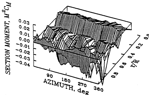
Fig. 17. Section lift and pitching moment for high weight coefficient/high speed case; C_W/\sigma = 0.13 ; \mu = 0.24 (Point F).
