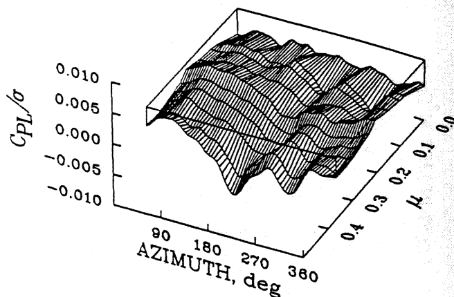
Fig. 5 Pitch-link load as a function of blade azimuth and advance ratio; C_W/\sigma = 0.08 .
