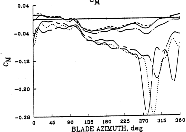
Fig. 12. Blade section lift and pitching moment coefficients at 0.865R with increasing weight coefficient at power-limit speeds.
