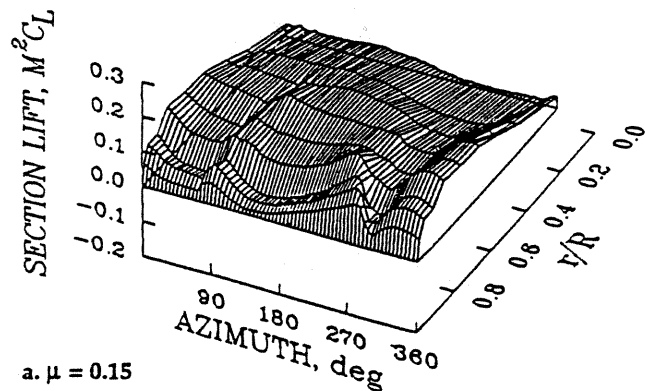
SECTION LIFT
