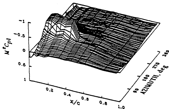
Fig. 8. Normalized pressure coefficient as a function of blade chord and azimuth at 0.965R for high weight coefficient/high speed case; C_w/\sigma = 0.08 , \mu = 0.37 (Point A).
