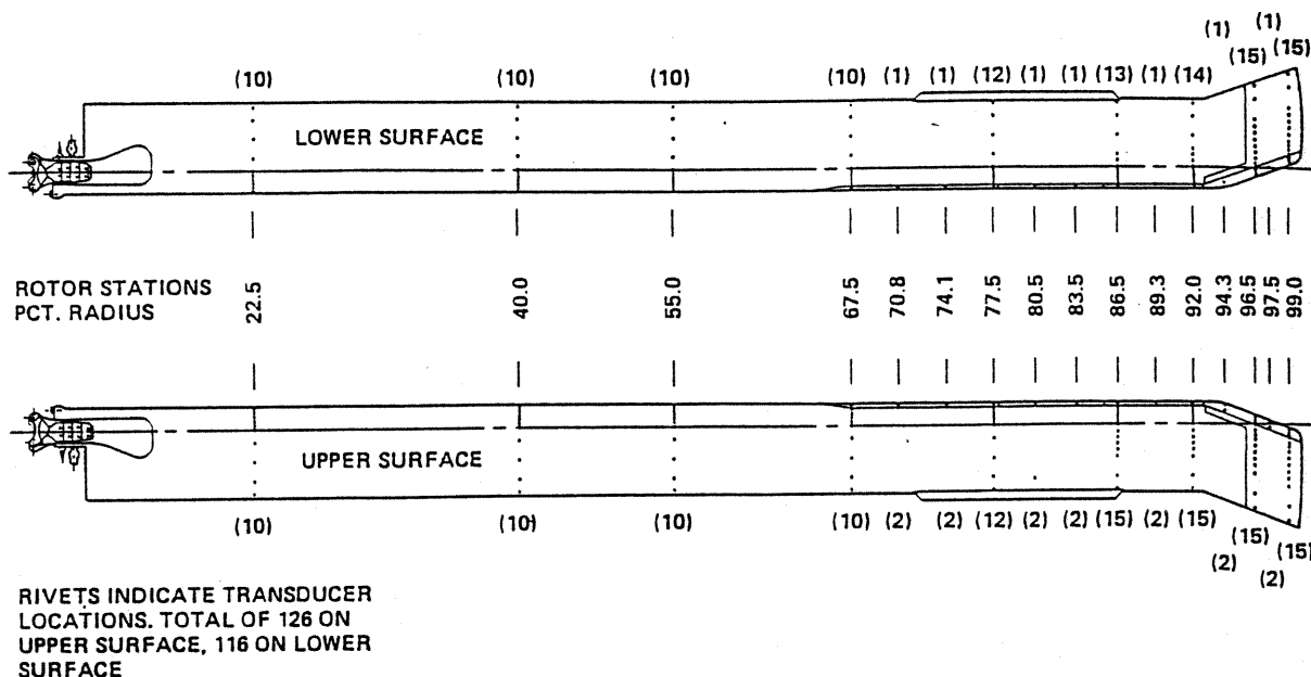
Fig. 1 UH-60A instrumented blade showing locations of pressure transducers.
