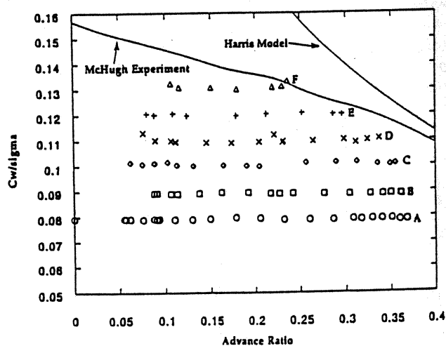
Fig. 2 UH-60A level flight data compared to McHugh (Ref. 1) and Harris (Ref. 7) boundaries.
