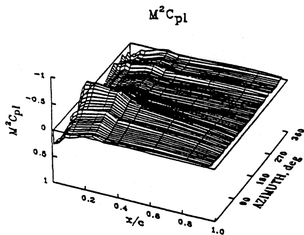
Fig. 15. Normalized pressure coefficient as a function of blade chord and azimuth at 0.865R for high weight coefficient/high speed case; C_w/\sigma = 0.13 , \mu = 0.24 (Point F).
