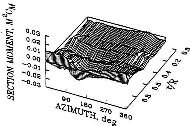
SECTION MOMENT
