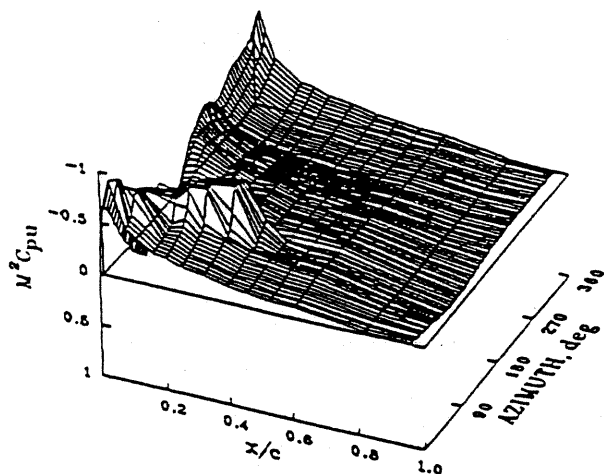
Fig. 7. Normalized pressure coefficient as a function of blade chord and azimuth at 0.865R for high weight coefficient/high speed case; C_w/\sigma = 0.08 , \mu = 0.37 (Point A).
