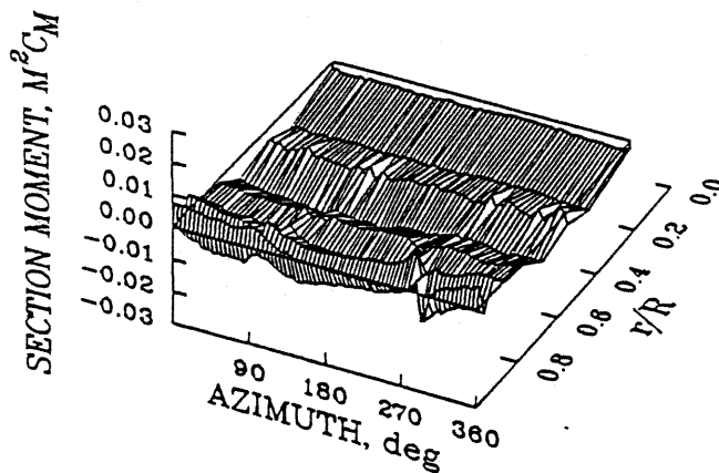
SECTION MOMENT
