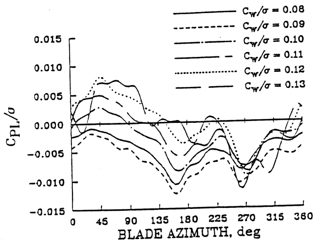
Fig. 13. Pitch-link load development with increasing weight coefficient at power-limit speeds.
