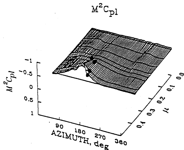
Fig. 6. Normalized pressure coefficient as a function of blade azimuth and advance ratio at 0.865R , 0.203c ; C_w/\sigma = 0.08 . Azimuth for Mach number divergence from 2-D data shown as solid circles.
