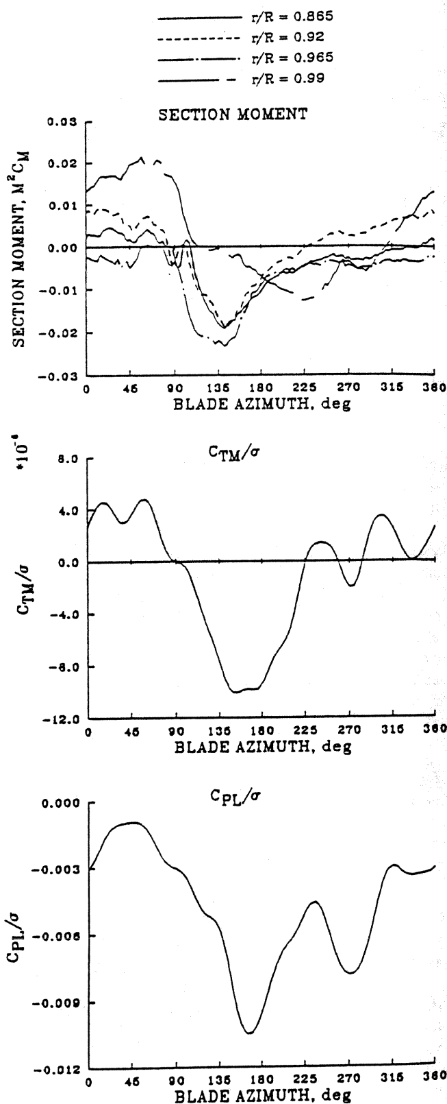
Fig. 10. Comparison of normalized section moment on outer portion of blade with torsion moment at 0.30R and pitch-link load for moderate weight coefficient/high speed case; C_W/\sigma = 0.08 , \mu = 0.37 (Point A).
