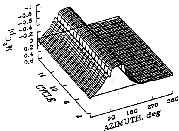
Fig. 9. Normalized surface pressure coefficient at 0.107c and 0.865R as a function of azimuth and cycle count for high weight coefficient/high speed case; C_W/\sigma = 0.08 , \mu = 0.37 (Point A).
