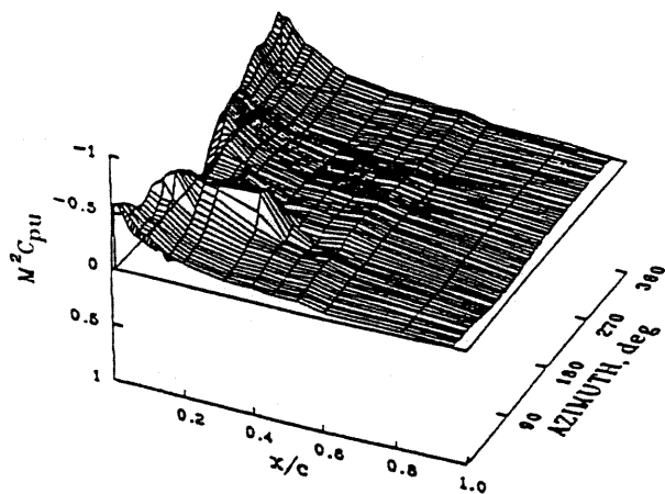
Fig. 8. Normalized pressure coefficient as a function of blade chord and azimuth at 0.965R for high weight coefficient/high speed case; C_w/\sigma = 0.08 , \mu = 0.37 (Point A).
