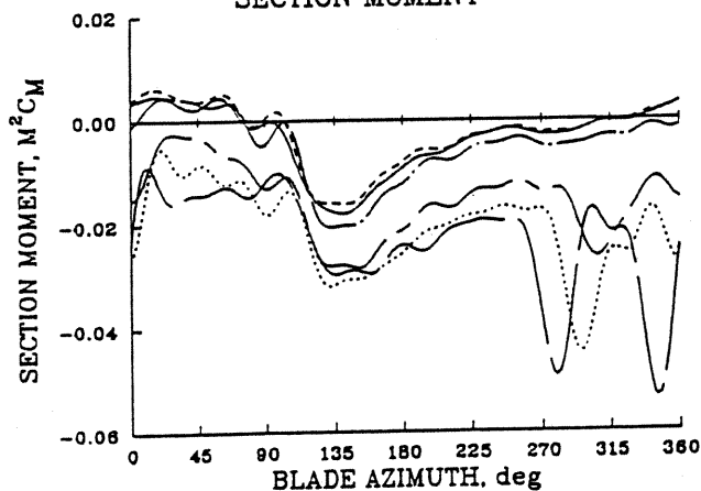
Fig. 11. Blade section lift and pitching moment normalized coefficients at 0.865R with increasing weight coefficient at power-limit speeds.
