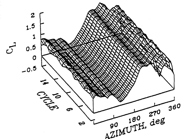
Fig. 16. Section lift coefficient at 0.865R as a function of azimuth and cycle count for high weight coefficient/high speed case; C_W/\sigma = 0.13 , \mu = 0.24 (Point F).
