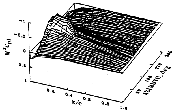
Fig. 7. Normalized pressure coefficient as a function of blade chord and azimuth at 0.865R for high weight coefficient/high speed case; C_w/\sigma = 0.08 , \mu = 0.37 (Point A).
