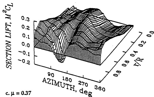
Fig. 3 Normalized section lift and pitching moments for three airspeeds; C_W/\sigma = 0.08 .
