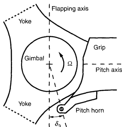
Fig. 8. Kinematics of V-22 hub and pitch horn, showing design \delta_3 of -15^\circ .
