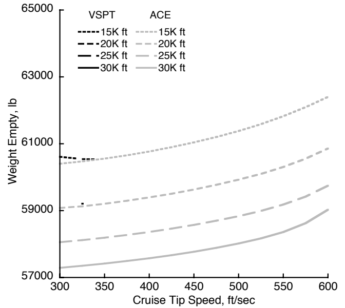
Fig. 11. Weight empty versus rotor tip speed for two propulsion concepts, for the 20-knot OEI sizing condition.
