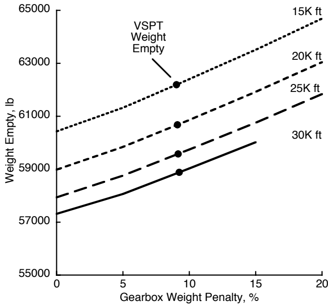
Fig. 15. Trends of weight empty with ACE gearbox weight penalty a V_{tip} = 600 ft/sec.
