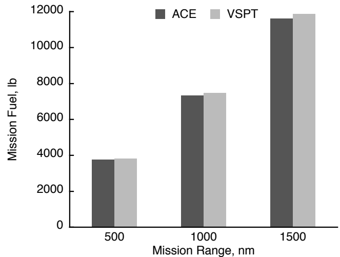
Fig. 17. Summary of effect of mission range on LCTR2 mission fuel burn.
