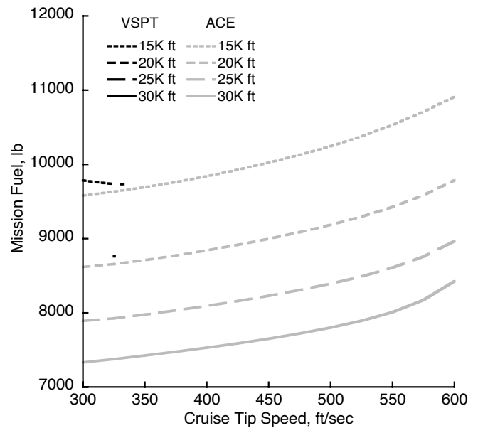
Fig. 12. Mission fuel burn versus rotor tip speed for two propulsion concepts, for the 20-knot OEI sizing condition.
