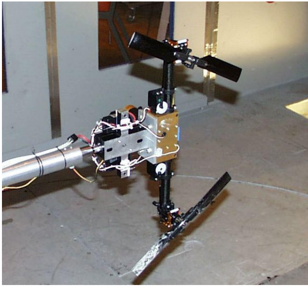
Fig. 3. Dual-rotor configuration of tiltrotor model.
