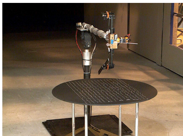
Fig. 2. Single-rotor with image plane configuration.
