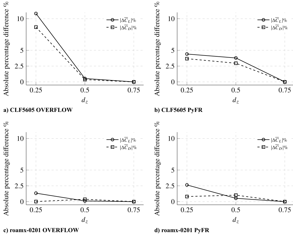
Fig. B2 Absolute percentage differences in time-averaged lift and drag coefficients with respect to the largest spanwise extent of the domain d_z = 0.75 , |\Delta \bar{C}_L| \% , and |\Delta \bar{C}_D| \% , plotted as a function of d_z for 3D-SP OVERFLOW and 3D-SP PyFR to assess the required spanwise extent of the domain for CLF5605 and roamx-0201 at \alpha = 6 deg.
