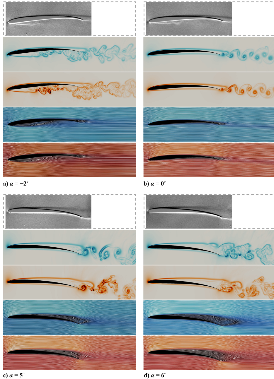
Fig. 14 Schlieren images for MWT experiments on clf5605-us-s (top) and images of instantaneous density gradient magnitude |\nabla\rho| (middle) and of time-averaged normalized velocity magnitude |v|/v_\infty with superimposed LICs (bottom) for 3D-SP OVERFLOW (blue) and 3D-SP PyFR (red) on CLF5605 for different \alpha .
