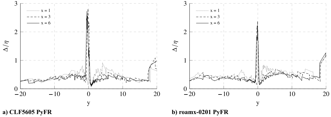
Fig. C1 Plots of \Delta/\eta in the midspan plane as a function of y at x = 1 , x = 3 , and x = 6 for 3D-SP PyFR at \alpha = 6 deg.
