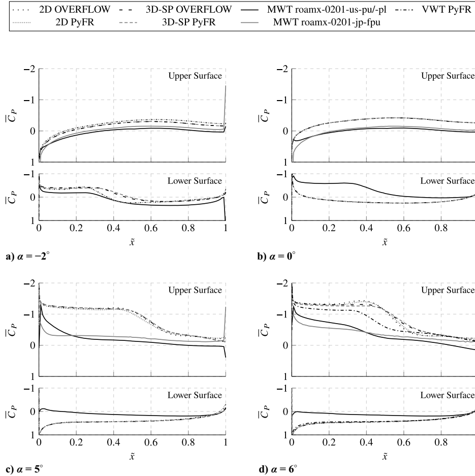
Fig. 13 Plots of time-averaged pressure coefficient \bar{C}_p as a function of \tilde{x} for different angles of attack for the roamx-0201 airfoil.
