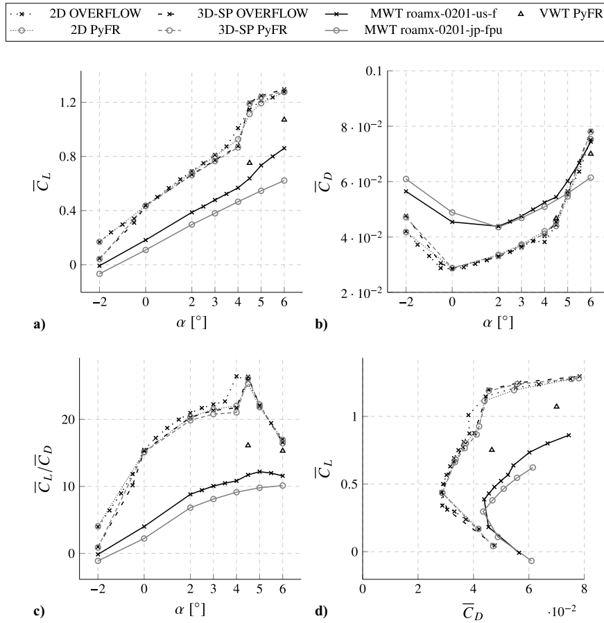
Fig. 11 Plots of time-averaged lift coefficient \bar{C}_L (a), drag coefficient \bar{C}_D (b), and lift-to-drag ratio \bar{C}_L/\bar{C}_D (c) as a function of angle of attack \alpha and lift coefficient \bar{C}_L as a function of drag coefficient \bar{C}_D (d) for the roamx-0201 airfoil.
