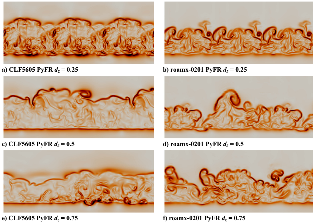
Fig. B3 Images of instantaneous density gradient magnitude |\nabla \rho| in the y - z plane at a distance of 0.05 chord lengths from the trailing edge for 3D-SP PyFR on CLF5605 (left) and roamx-0201 (right) at \alpha = 6 deg with domain span lengths of d_z = 0.25 , d_z = 0.5 , and d_z = 0.75 chord lengths. Note that for d_z = 0.25 and d_z = 0.5 chord lengths the periodic data are repeated 3 and 1.5 times, respectively, to facilitate comparison.
