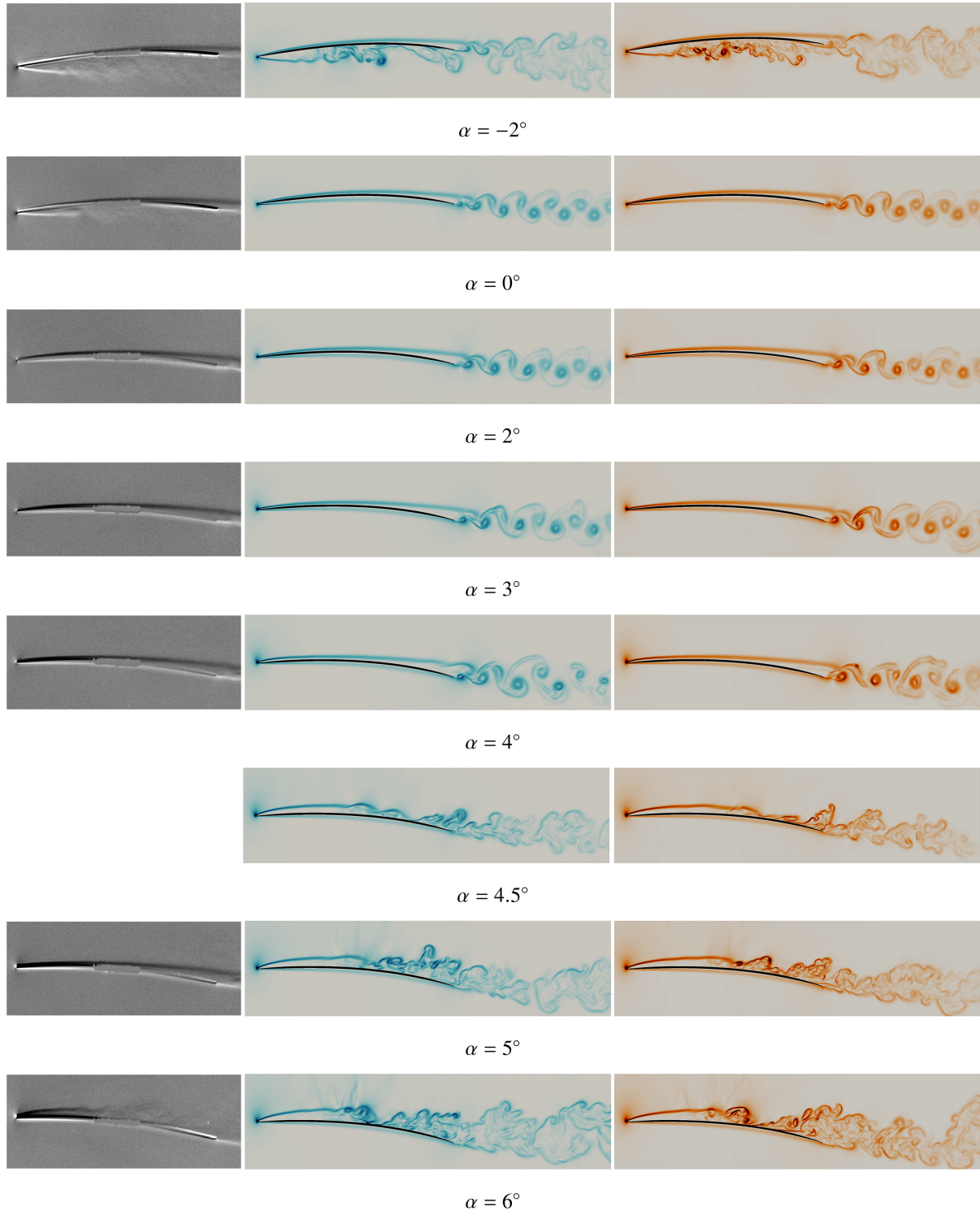
Fig. E2 Schlieren images for MWT experiments on model roamx-0201-jp-s (left) and images of instantaneous density gradient magnitude |\nabla\rho| for 3D-SP OVERFLOW (middle) and PyFR (right) on roamx-0201 for different \alpha .
