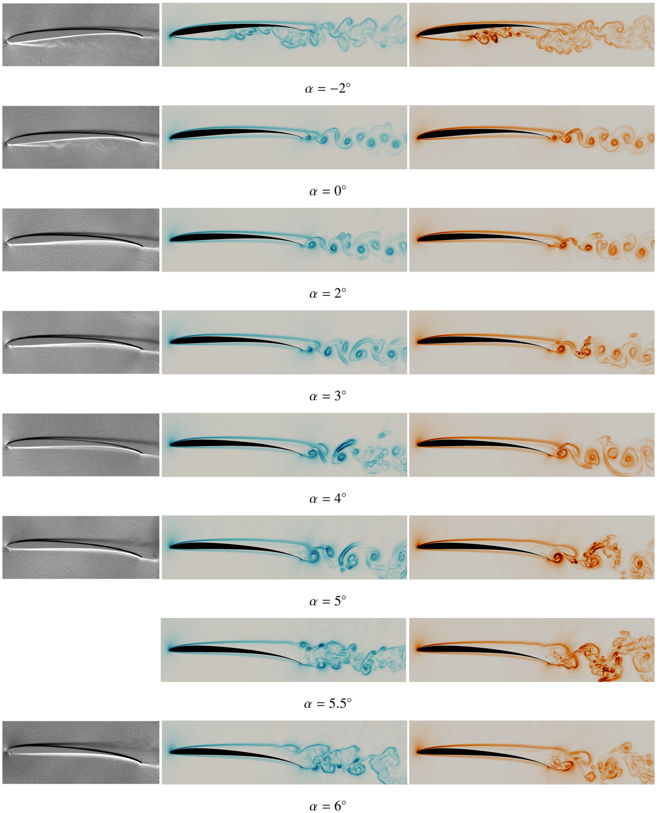
Fig. E1 Schlieren images for MWT experiments on model clf5605-us-s (left) and images of instantaneous density gradient magnitude |\nabla\rho| for 3D-SP OVERFLOW (middle) and PyFR (right) on CLF5605 for different \alpha .
