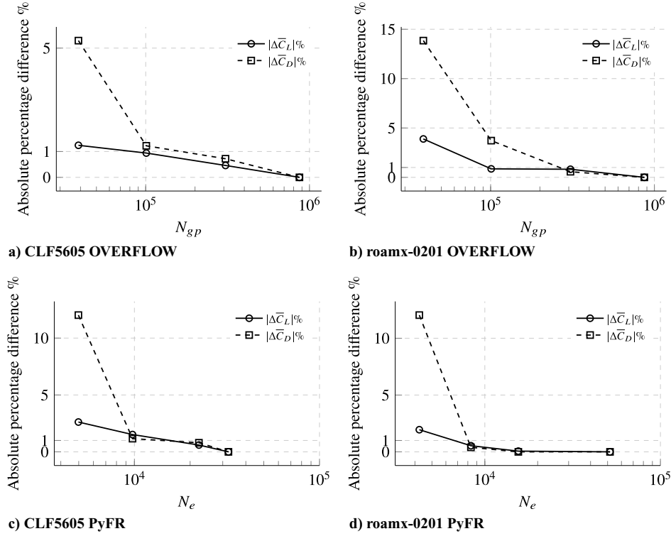
Fig. A1 Absolute percentage differences in time-averaged lift and drag coefficients with respect to the finest mesh, |\Delta \bar{C}_L| % and |\Delta \bar{C}_D| %, plotted as a function of the number of grid points N_{gp} for 2D OVERFLOW and number of elements N_e for 2D PyFR to assess grid convergence of CLF5605 and roamx-0201 at \alpha = 6 .
