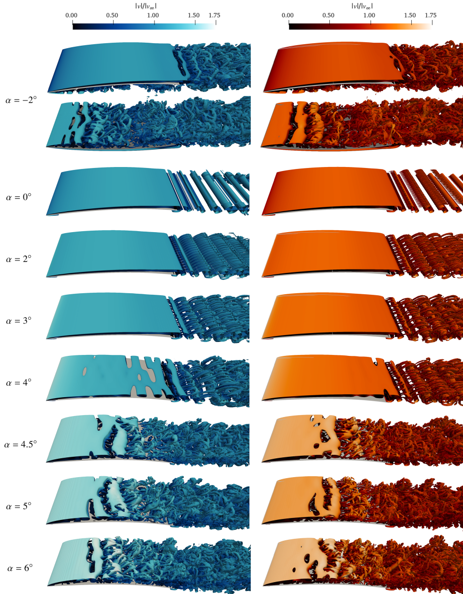
Fig. 17 Images of instantaneous Q -criterion isosurfaces Q = 1 colored by normalized velocity magnitude |v|/|v_\infty| obtained with 3D-SP OVERFLOW (left) and 3D-SP PyFR (right) for the roamx-0201 airfoil.
