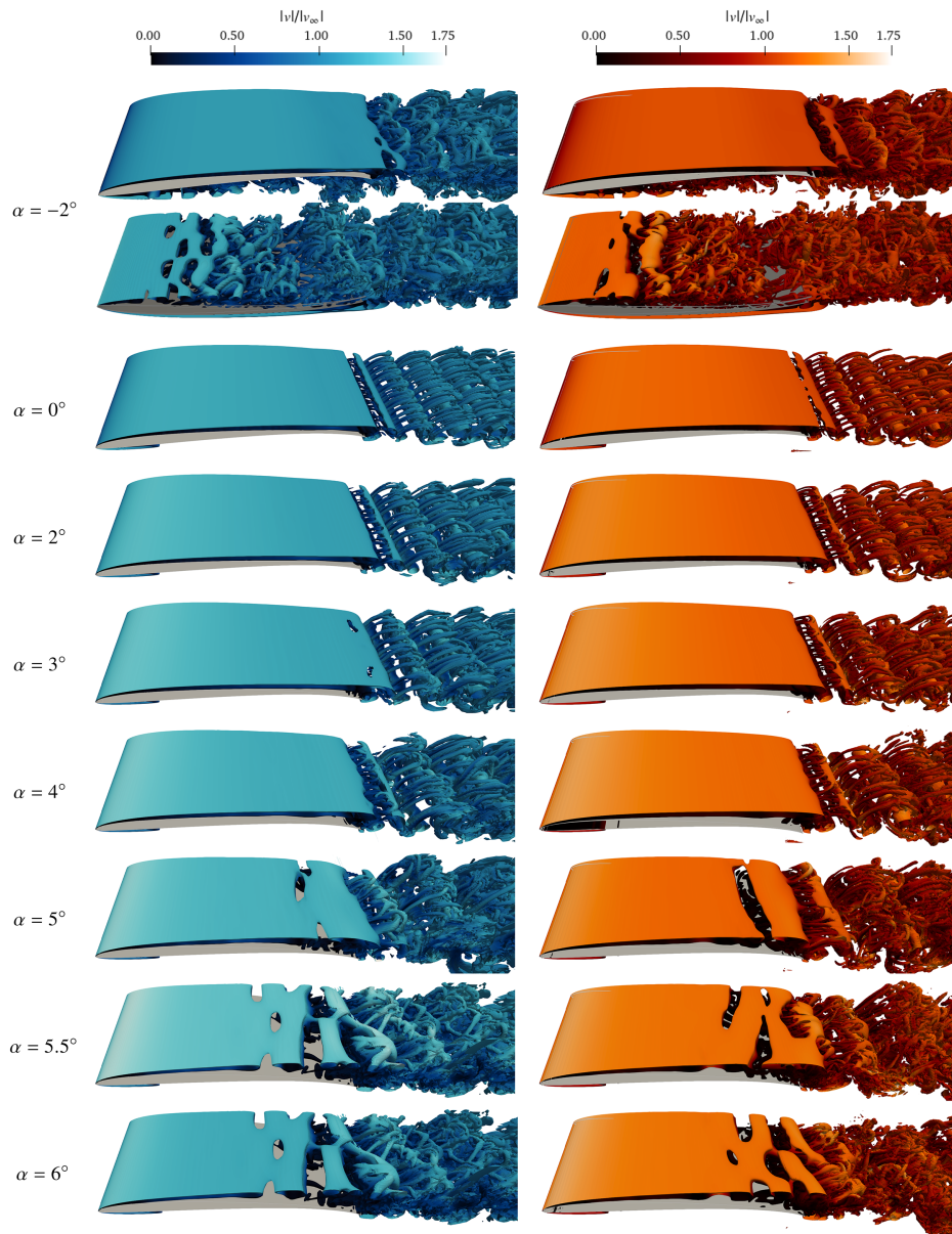
Fig. 16 Images of instantaneous Q -criterion isosurfaces Q = 1 colored by normalized velocity magnitude |v|/|v_\infty| obtained with 3D-SP OVERFLOW (left) and 3D-SP PyFR (right) for the CLF5605 airfoil.
