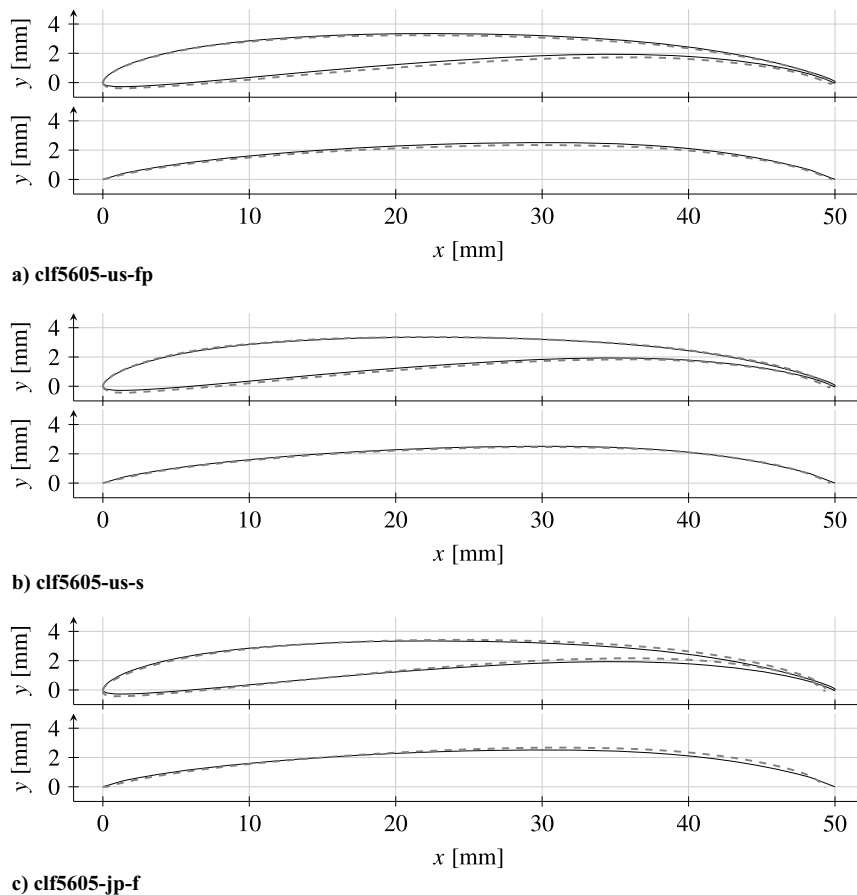
Fig. 20 CLF5605 airfoil profiles (top) and their camber lines (bottom) extracted from the scanned models (dashed lines) and compared with the reference CLF5605 airfoil and camber line (solid lines). The scanned geometries were aligned by identifying the leading and trailing edges and rotating them such that both points lie on a common horizontal axis ( y = 0 ). The reference airfoil geometry is scaled to a chord length of 50 mm, corresponding to the target length of the manufactured models.
