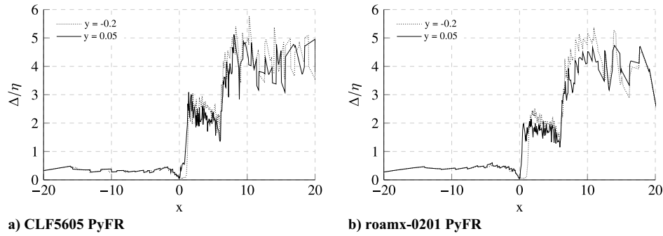
Fig. C4 Plots of \Delta/\eta in the midspan plane as a function of x at y = 0.05 , and y = -0.2 for 3D-SP PyFR at \alpha = 6 deg.
