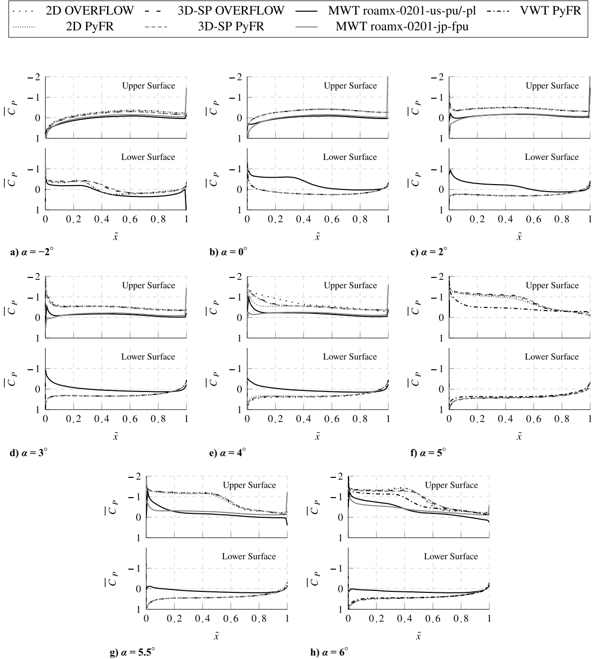
Fig. D2 Plots of time-averaged pressure coefficient \bar{C}_P as a function of \tilde{x} for different angles of attack \alpha for the roamx-0201 airfoil.
