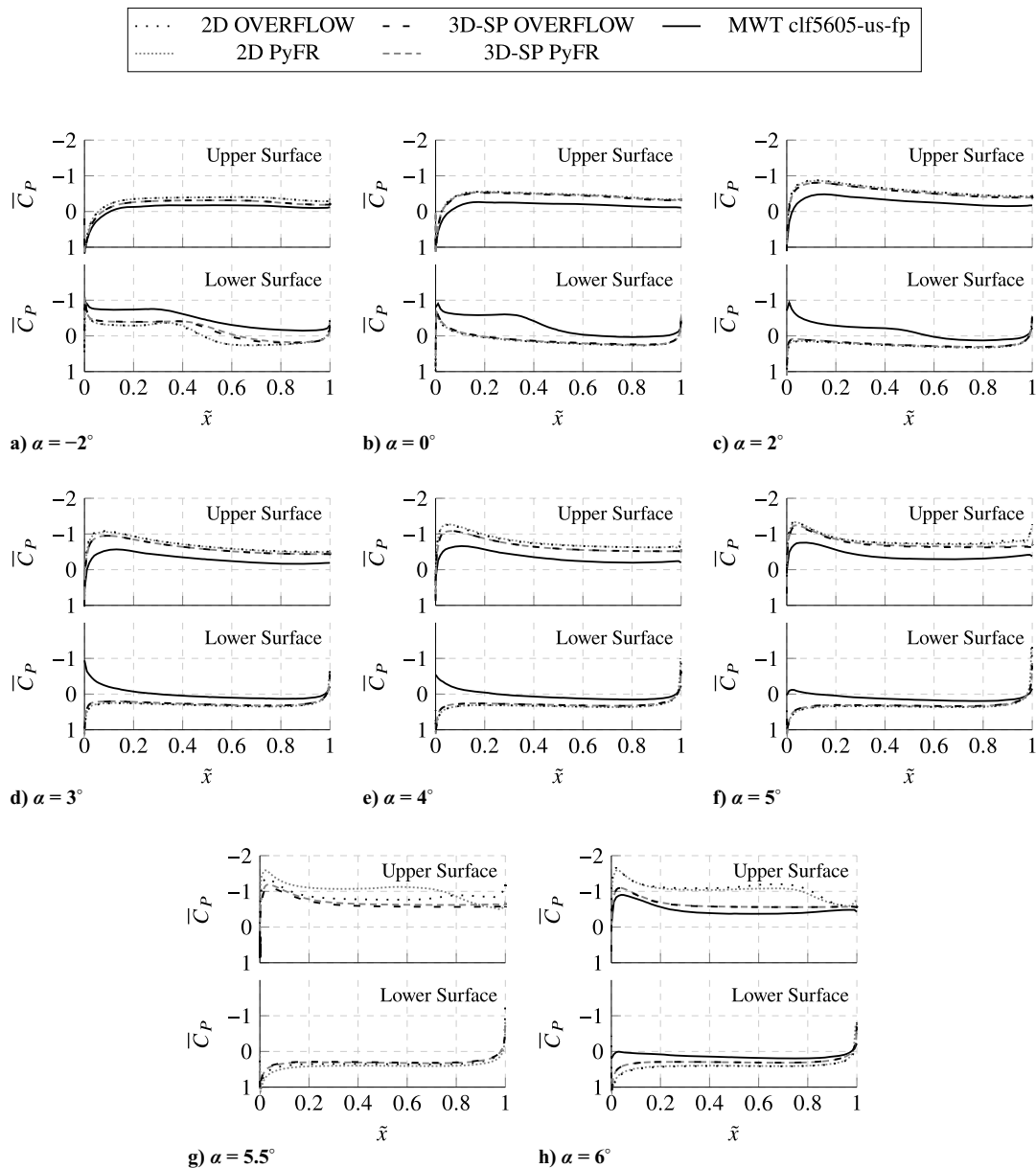
Fig. D1 Plots of time-averaged pressure coefficient \bar{C}_p as a function of \tilde{x} for different angles of attack \alpha for the CLF5605 airfoil.
