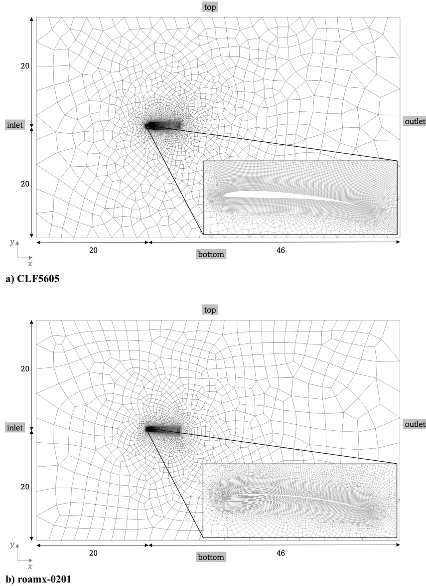
Fig. 3 Views of domain and mesh in the streamwise-vertical xy -plane used for 2D and 3D-SP simulations with PyFR for the CLF5605 (a) and roamx-0201 (b) airfoils when \alpha = 6 deg.
