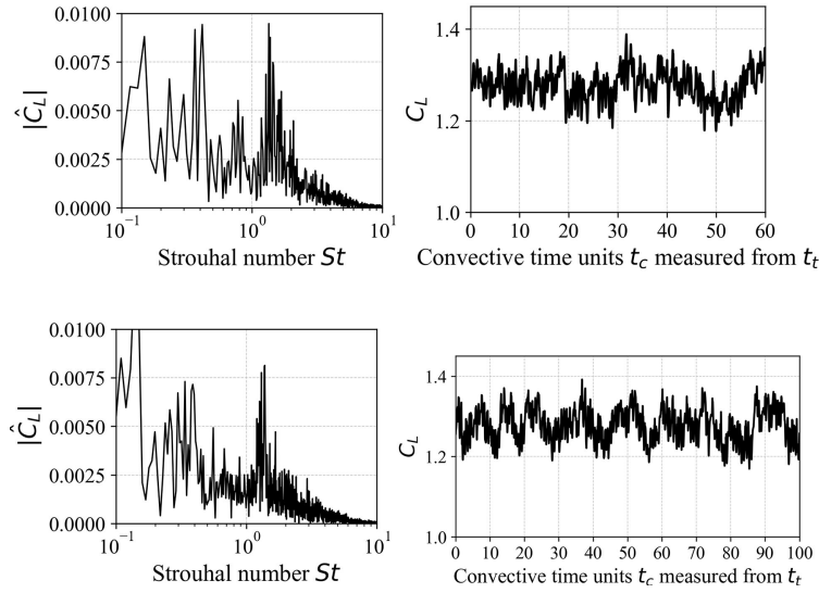
a) 2D OVERFLOW (top) and 2D PyFR (bottom)
