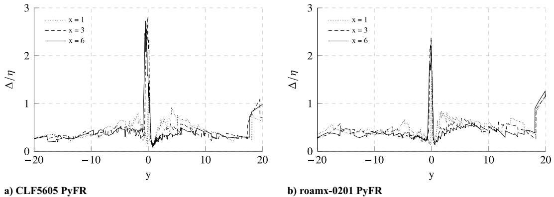
Fig. C3 Plots of \Delta/\eta in the midspan plane as a function of y at x = 1 , x = 3 , and x = 6 for 3D-SP PyFR at \alpha = 6 deg.
