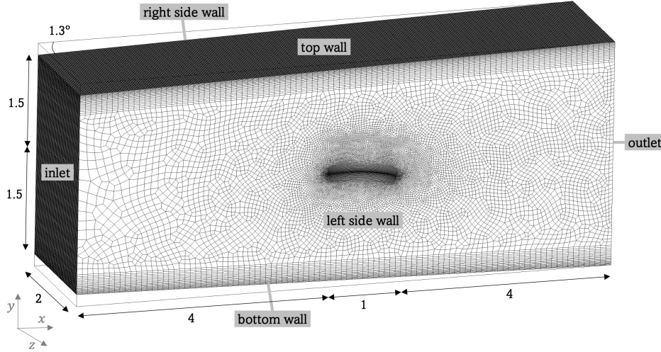
Fig. 4 View of the computational mesh used for the virtual wind tunnel (VWT) with PyFR for roamx-0201 at \alpha = 6 deg. The origin in the streamwise-vertical xy -plane is located at the leading edge of the airfoil when \alpha = 0 deg.
