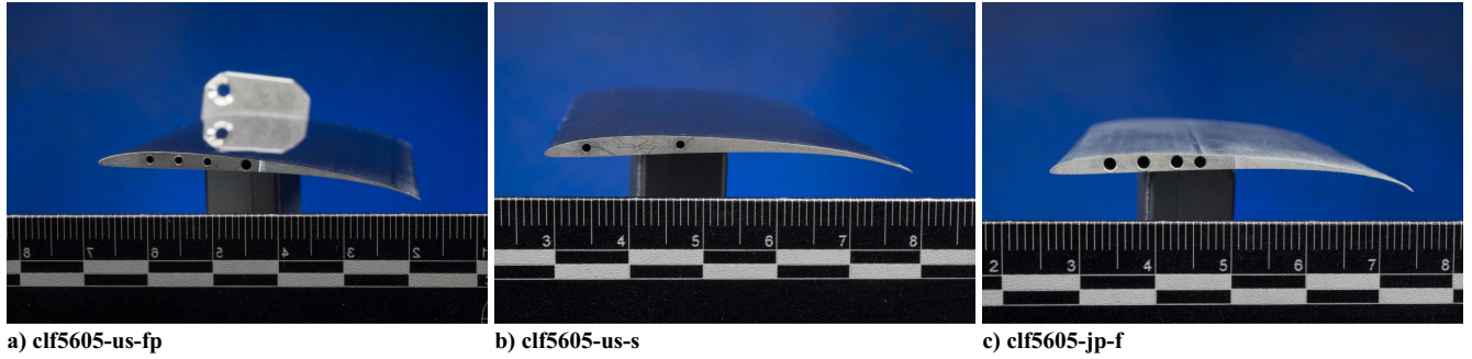
Fig. 6 Images of CLF5605 models (scale shown in cm).
