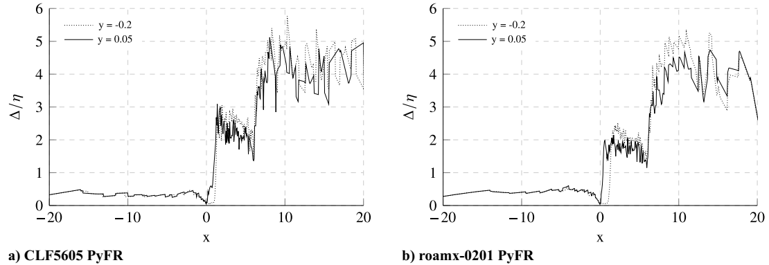
Fig. C2 Plots of \Delta/\eta in the midspan plane as a function of x at y = 0.05 and y = -0.2 for 3D-SP PyFR at \alpha = 6 deg.
