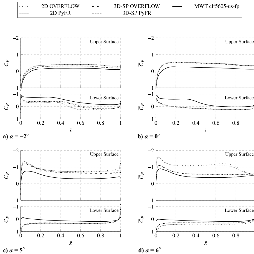
Fig. 12 Plots of time-averaged pressure coefficient \bar{C}_P as a function of \tilde{x} for different angles of attack for the CLF5605 airfoil.
