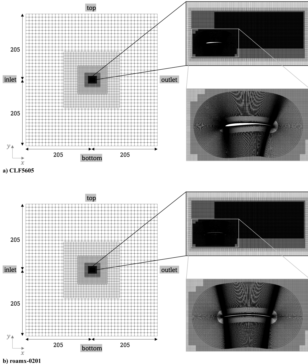
Fig. 2 Views of domain and mesh in the streamwise-vertical xy -plane used for 2D simulations with OVERFLOW for the CLF5605 (a) and roamx-0201 (b) airfoils.
