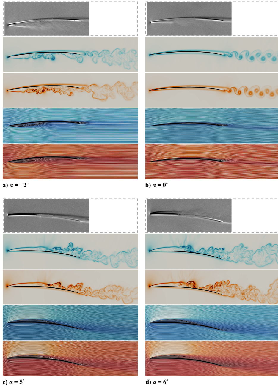
Fig. 15 Schlieren images for MWT experiments on roams-0201-jp-s (top) and images of instantaneous density gradient magnitude |\nabla\rho| (middle) and of time-averaged normalized velocity magnitude |v|/v_\infty with superimposed LICs (bottom) for 3D-SP OVERFLOW (blue) and 3D-SP PyFR (red) on roams-0201 for different \alpha .
