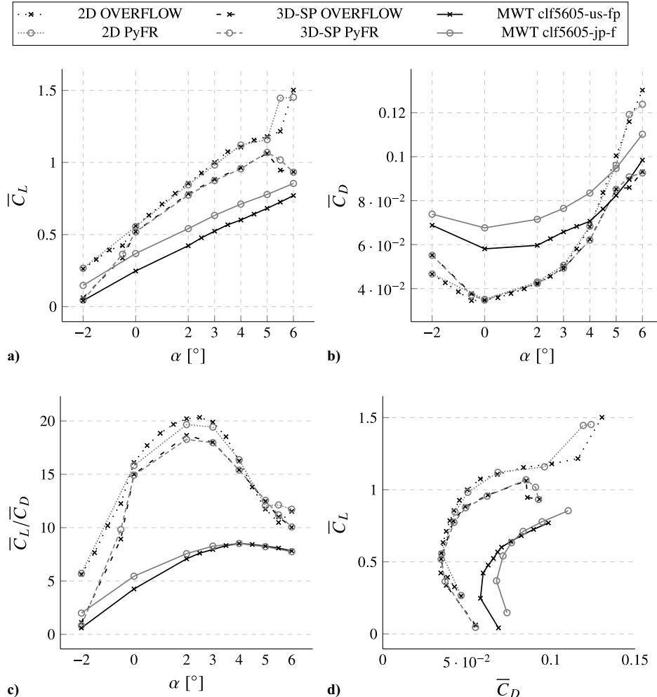
Fig. 10 Plots of time-averaged lift coefficient \bar{C}_L (a), drag coefficient \bar{C}_D (b), and lift-to-drag ratio \bar{C}_L/\bar{C}_D (c) as a function of angle of attack \alpha and lift coefficient \bar{C}_L as a function of drag coefficient \bar{C}_D (d) for the CLF5605 airfoil.
