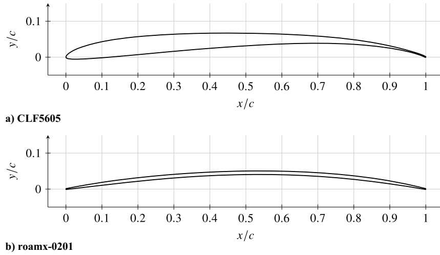
Fig. 1 CLF5605 (a) and roamx-0201 (b) airfoils.
