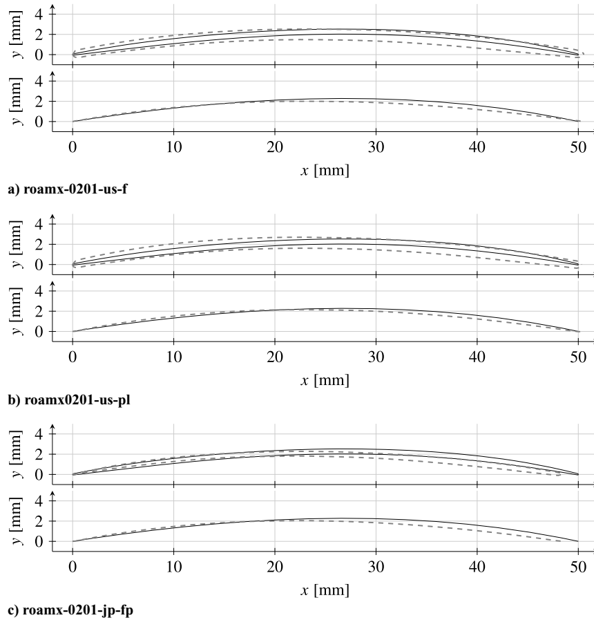
Fig. 21 Roamx-0201 airfoils (top) and their camber lines (bottom) extracted from the scanned models (dashed lines) compared with the reference roamx-0201 airfoil and camber line (solid lines). The scanned geometries were aligned with the reference roamx-0201 airfoil by identifying the leading and trailing edges and rotating them such that both points lie on a common horizontal axis ( y = 0 ). The reference airfoil geometry is scaled to a chord length of 50 mm, corresponding to the target length of the manufactured models.
