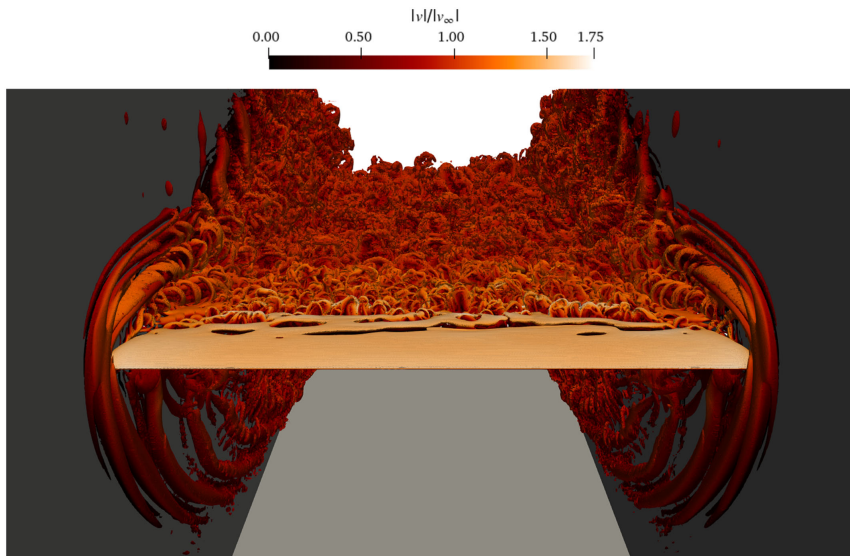
Fig. 18 Instantaneous snapshot of Q -criterion isosurfaces colored by normalized velocity magnitude |v|/|v_\infty| obtained with a VWT PyFR simulation for the roamx-0201 airfoil with \alpha = 6 deg case.
