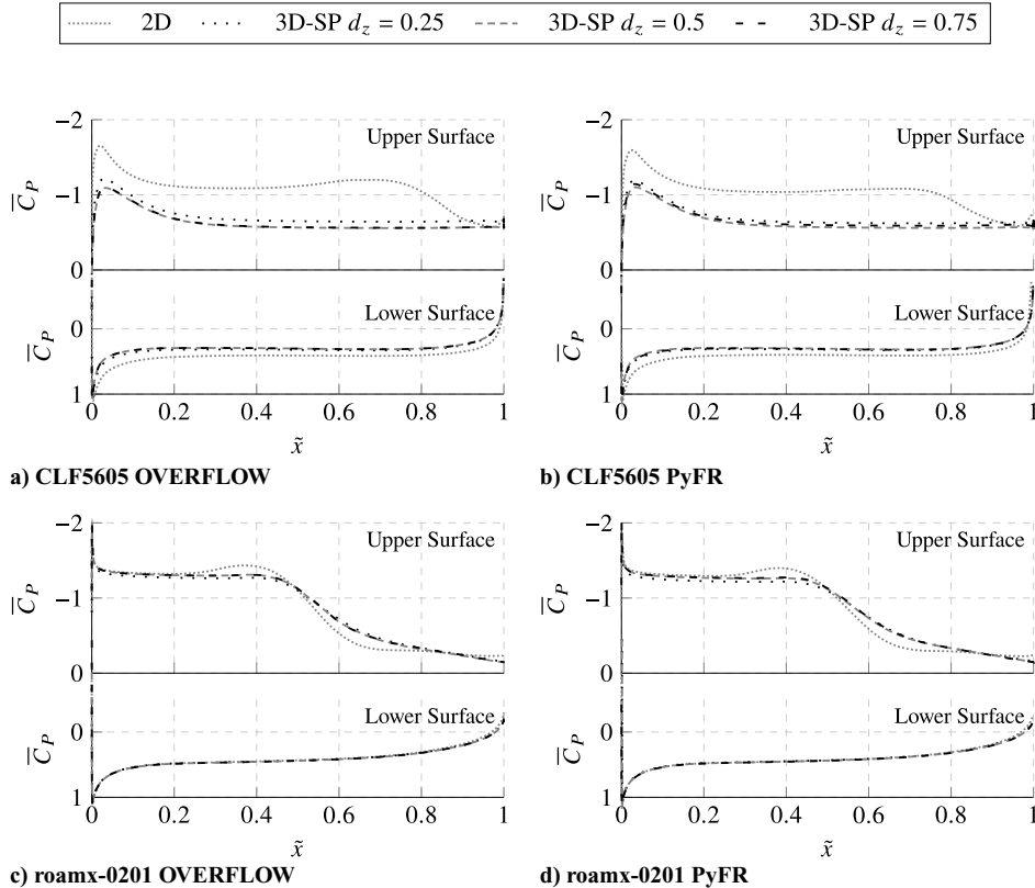
Fig. B1 Plots of time-averaged pressure coefficient \bar{C}_p as a function of \tilde{x} for different span lengths of the domain d_z to assess domain span length independence for 3D-SP OVERFLOW and PyFR simulations of CLF5605 and roamx-0201 at \alpha = 6 deg.
