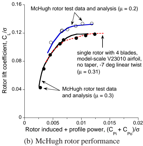
Fig. 8. Comparison of rotor performance.
