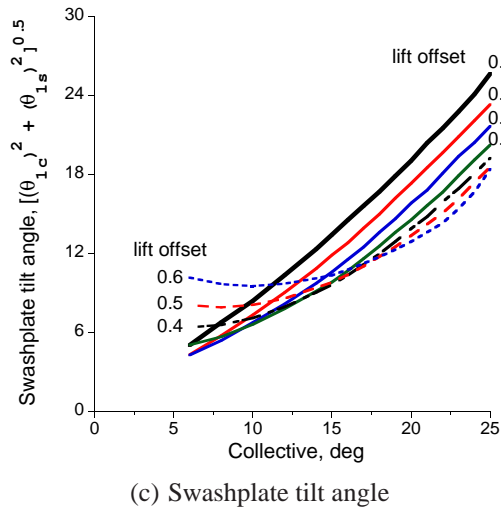
Fig. 10. Upper rotor cyclic control angles of the coaxial rotor, 120 knots ( \mu = 0.31 ), \alpha_s = 0^\circ .
