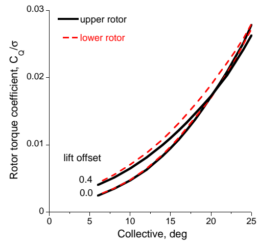
(b) torque
