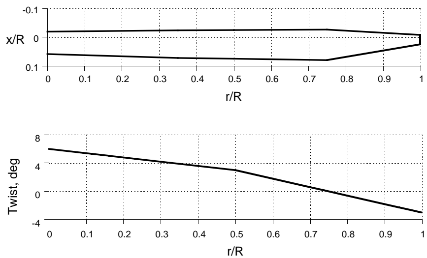
Fig. 2. Blade planform and twist
