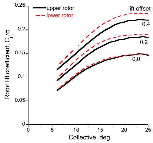
(a) lift
