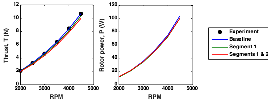
Figure 23. Effect of segment substitution on thrust and power, free wake, \theta_o = -1 deg, \Delta TR_{lim} = 0.05 .
