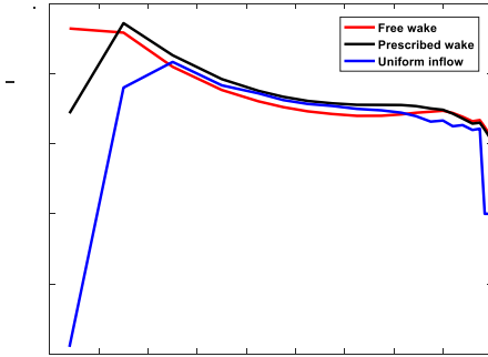
(c) Sectional lift coefficient
