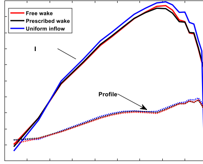
(f) Sectional power
