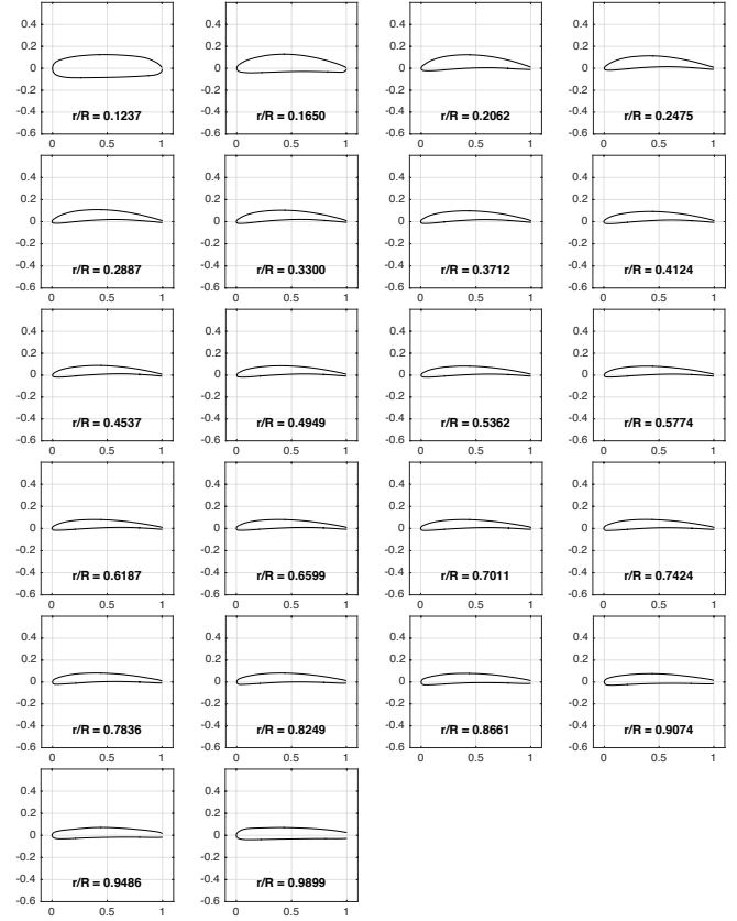
Figure 4. SUI Endurance airfoil geometry at various span-wise locations, chord length normalized.
