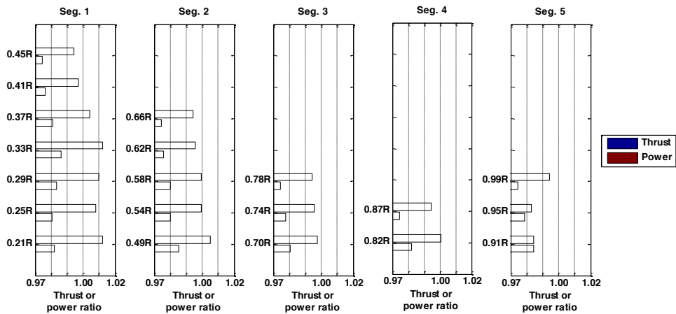
Figure 21. Effect of airfoil selection on thrust and power, free wake, \theta_o = -1 deg, \Delta TR_{lim} = 0.01 .
