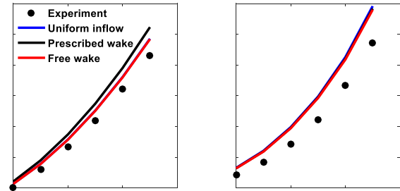
Figure 13. Effect of wake modeling on SUI performance, \theta_o = 0^\circ , hover.
