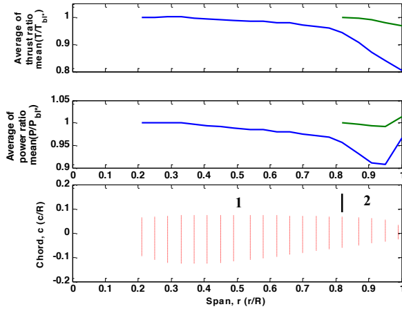
Figure 22. Change in thrust and power ratio due to changes in airfoil distribution, free wake, \theta_o = -1 deg, \Delta TR_{lim} = 0.05 .
