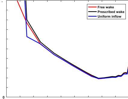
(e) Sectional drag coefficient
