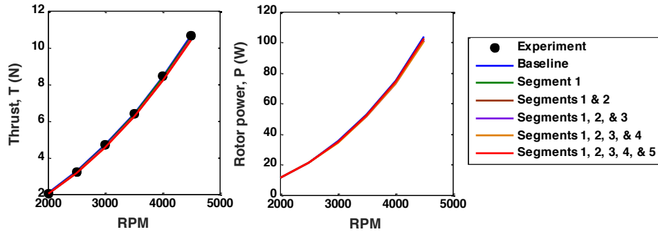
Figure 20. Effect of segment substitution on thrust and power, free wake, \theta_o = -1 deg, \Delta TR_{lim} = 0.01 .
