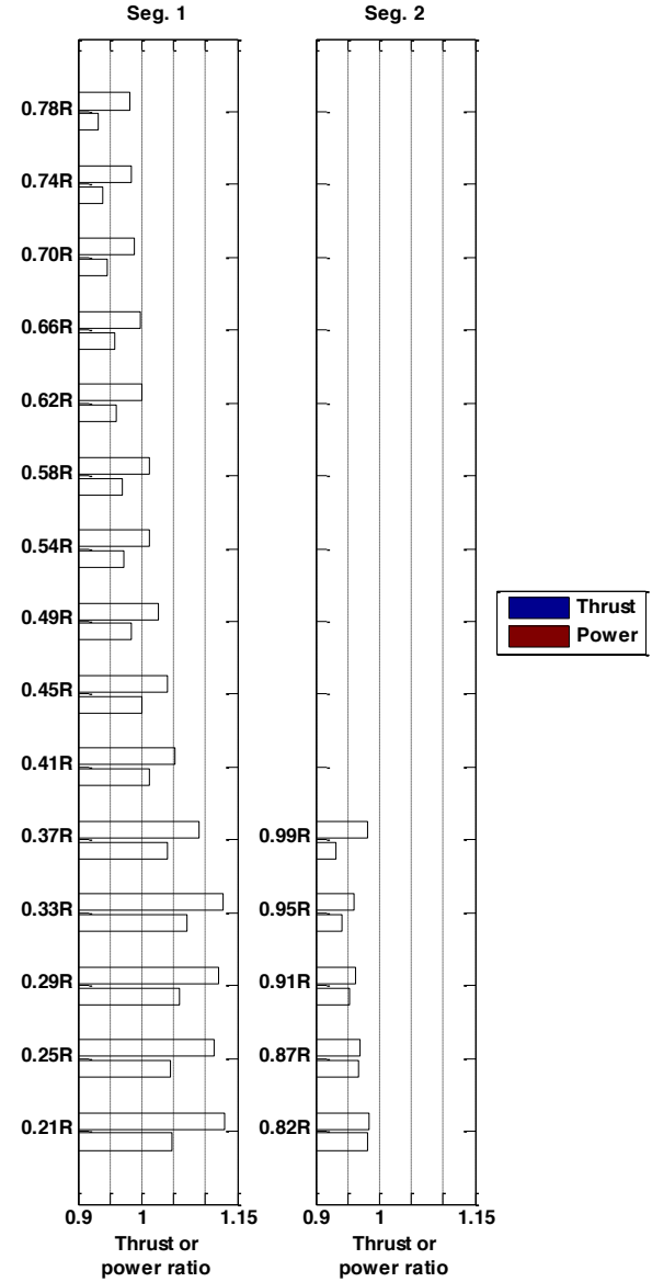
Figure 24. Effect of airfoil selection on thrust and power, free wake, \theta_o = -1 deg, \Delta TR_{lim} = 0.05 .
