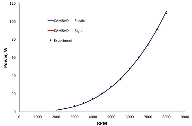
Figure 8. Predicted power for DJI Phantom 3 rotor.
