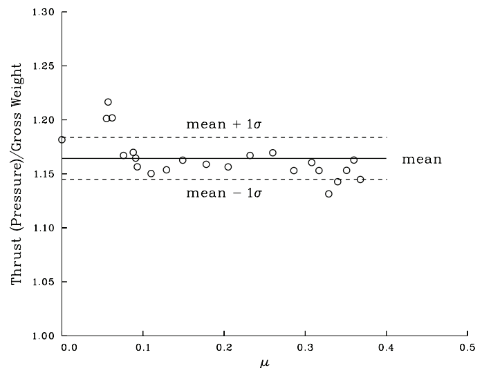
Figure 26. Thrust/weight comparison for the UH-60A flight test as a function of advance ratio; Flight 85, n = 23 .
