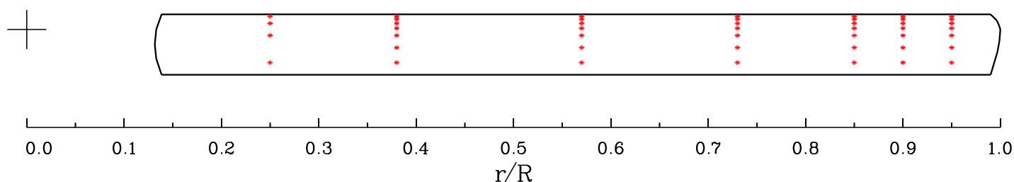
Figure A-28. XH-51A blade planform showing locations of pressure transducers at seven radial stations.
