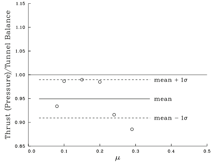
Figure 24. Thrust/balance comparison for NACA model rotor as a function of advance ratio (Rabbott and Churchill, 1956); n = 6 .
