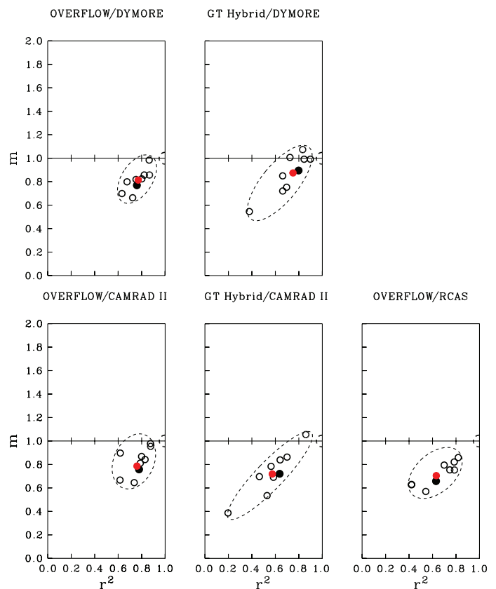
Figure 50. Accuracy maps of measured normal forces at nine radial stations (open circles) for the UH-60A with five coupled CFD/CSD methods for the Second Problem, \mu = 0.24 , C_w/\sigma = 0.133 . Solid black circles are 0.92R ; solid red circles show the combined accuracies.
