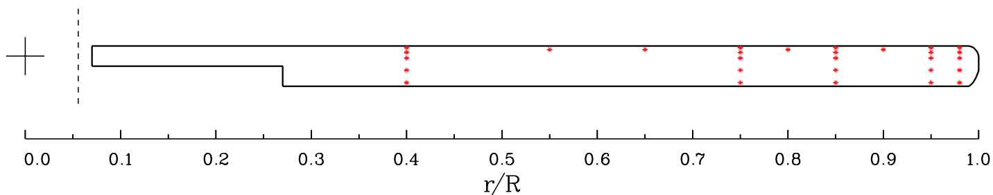
Figure A-32. CH-53A blade planform showing locations of pressure transducers at five radial stations.
