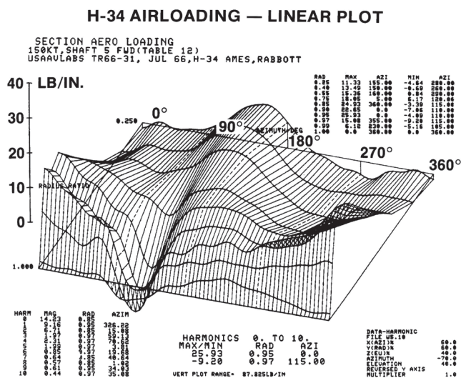
Figure 43. CH-34 section normal forces in wind tunnel test, \mu = 0.39 , \alpha_s = -5^\circ (courtesy of Euan Hooper).
